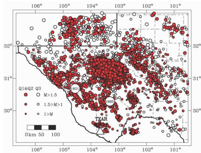
Figure 3. Map of epicenters (2000-2017) determined in this study from the analysis of TXAR data. Symbol size and color indicates magnitude M_{\text{TXAR}} and quality Q1 (better) to Q3 (worse) assigned by analyst to P and S time picks (see Data and Methods section 2.2)
