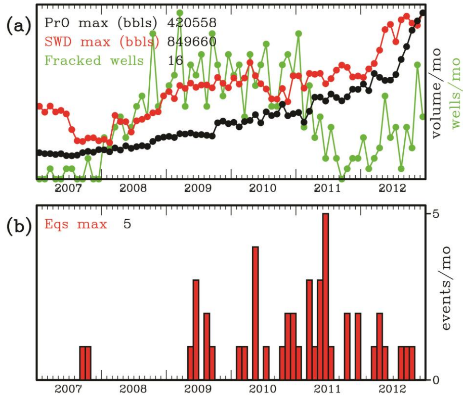
Figure 10. Petroleum-production activity near the 2009 epicenters (within 10 km of 31.395N 103.390W). (a) Monthly volumes for produced oil (PrO), wastewater disposal (SWD), and the number of hydraulically fractured wells initiated. Plotted values are normalized to maximum monthly values, given at upper left. (b) Monthly earthquake numbers in TXAR catalog.
