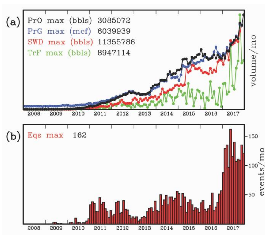
Figure 11. Petroleum-production operations and seismicity in circle 7c. (a) Monthly volumes for produced oil (PrO), produced gas (PrG), wastewater disposal (SWD), and hydraulic fracturing treatment fluid (TrF). Plotted values on vertical axes are normalized to maximum monthly values, given at upper left. (b) Monthly earthquake numbers in TXAR catalog.
