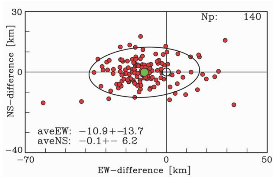
Figure 5. Comparison of epicenters determined using (S-P) intervals and apparent direction at TXAR with epicenters determined by the TexNet seismic network using conventional location methods. Data are for 140 earthquakes within Pecos Cluster Circle S3b; all plotted events had P and S picks that the analyst assigned quality 1 or 2 (red circles in Figure 3). The ellipsoid indicates the 2\sigma fit for these data; the green dot at -10.9 km is the center of the ellipsoid—this indicates that before back azimuths for TXAR locations are adjusted by adding 3^\circ (see text), they average 10.9 km west of TexNet locations.
