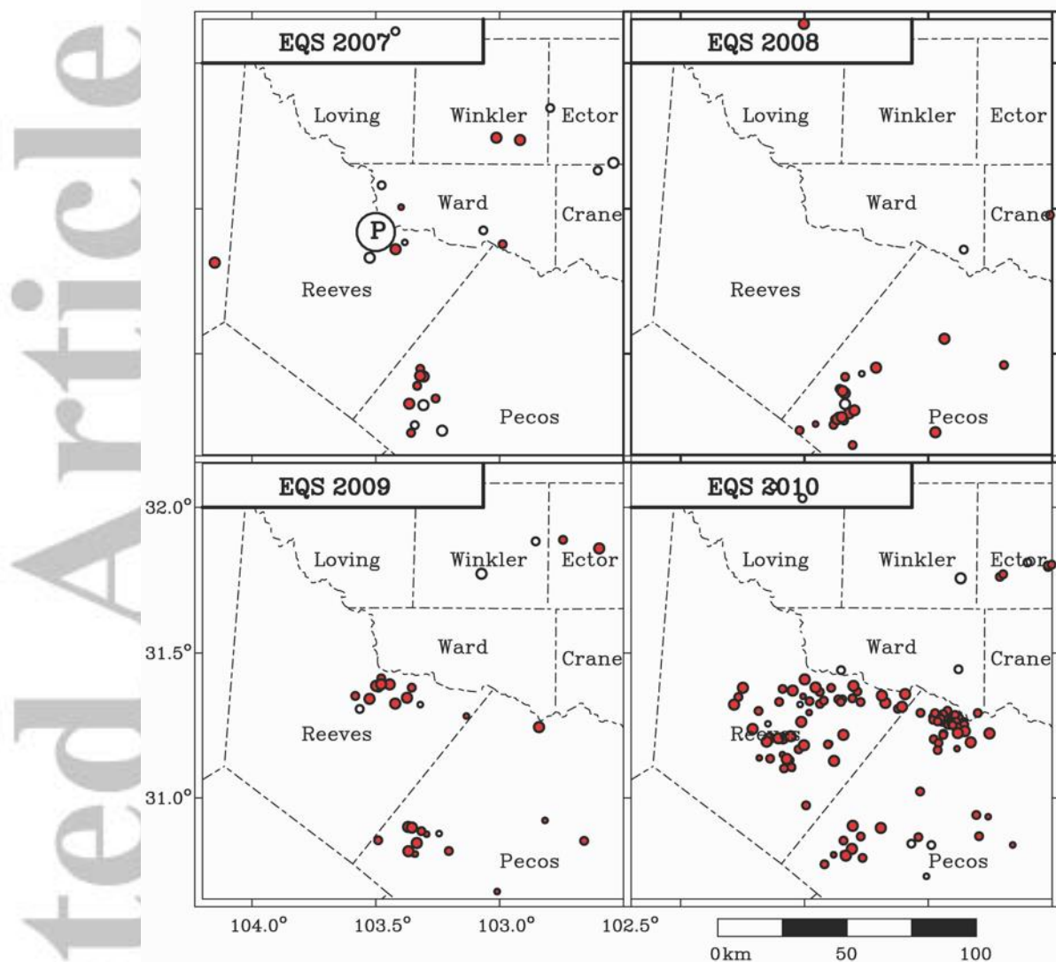
Figure 8. Maps of TXAR-determined epicenters near Pecos, 2007-2010. Small circles are seismic events; sizes and colors are as in Figure 3. The large circle labeled “P” on 2007 map is the town of Pecos, TX. Note also that near the town of Pecos, multiple earthquakes occur in 2009, and activity grows in number and aerial extent in 2010. See Figure S4 for maps of all years 2000 through 2017.
