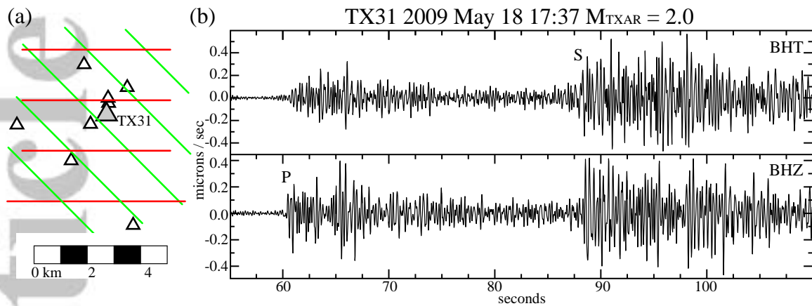
Figure 4. Earthquake location with the Lajitas TXAR array. (a) Map view of the seismic stations in the TXAR array. Note that two high-gain stations (white triangles) are hidden by the broadband station (grey triangle) at this scale. Red and green lines depict P-wave fronts crossing the array from earthquakes occurring to the north and northeast, respectively. Automated detection of relative arrival times across TXAR array stations constrains the source-to-station direction for the event. (b) Transverse- (BHT) and vertical-component (BHZ) seismograms for a Pecos Cluster earthquake at station TX31 of TXAR. Analyst-refined picks for P and S arrivals and the (S-P) interval at TX31 constrain the source-to-station distance for the event.
