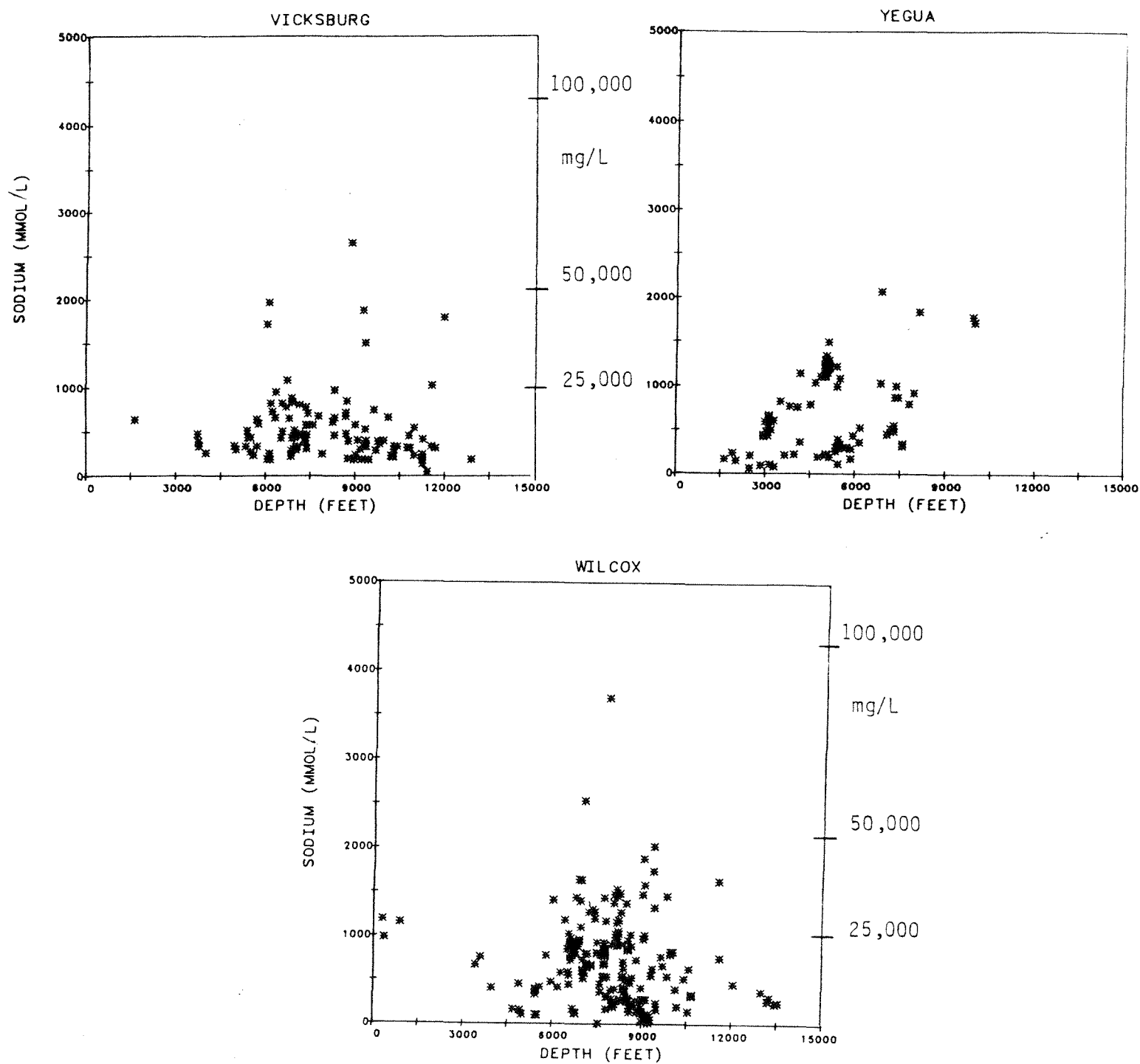
Figure 23. Sodium-depth plot for Vicksburg, Yegua, and Wilcox formation waters.
