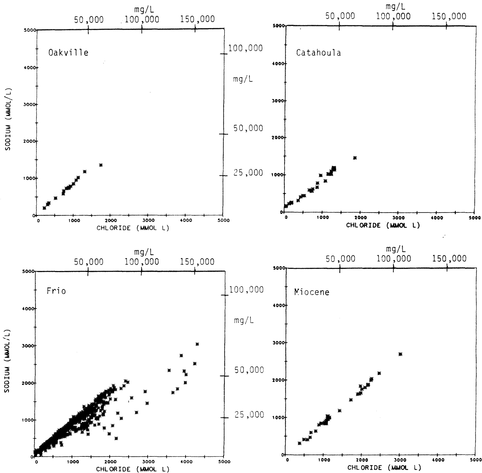
Figure 24. Sodium-chloride plot for Oakville, Catahoula, Frio, and Miocene formation waters.
