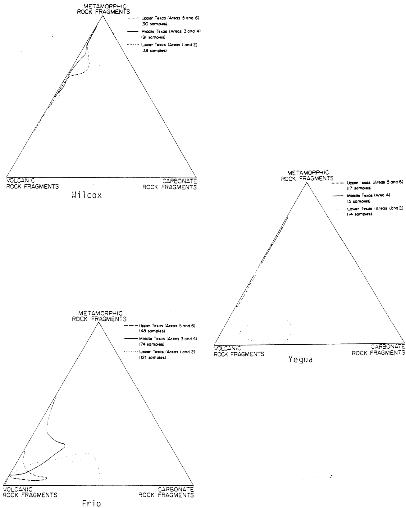
Figure 56. Composition of Wilcox, Yegua, and Frio rock fragments (from Loucks and others, 1979).
