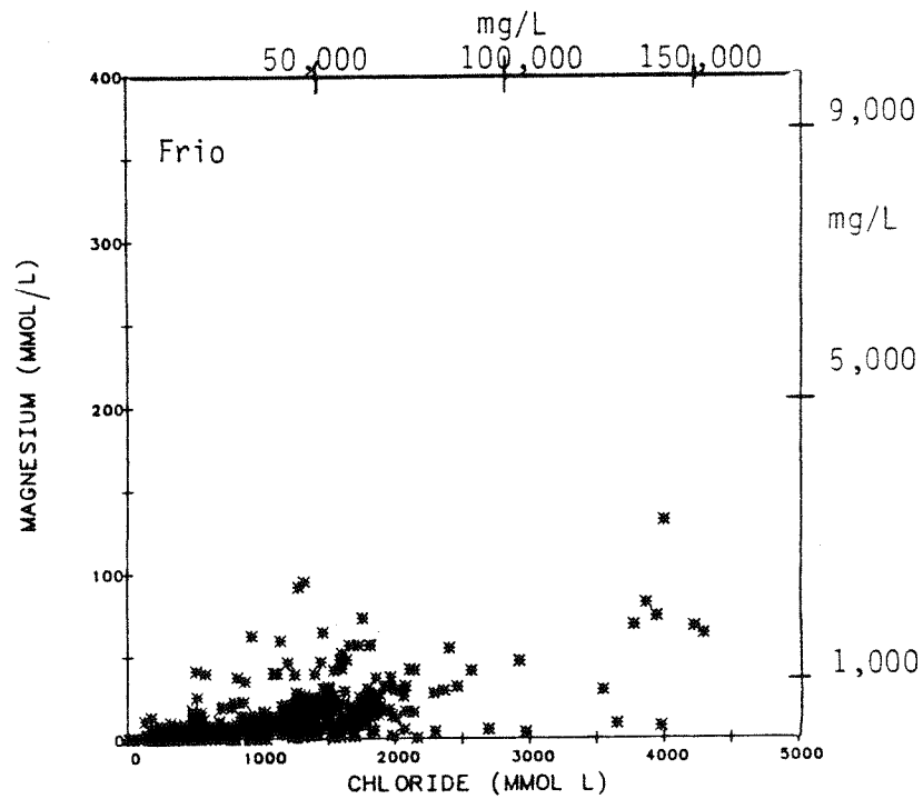
Figure 32. Magnesium-chloride plots of Oakville, Catahoula, Frio, and Miocene formation waters.
