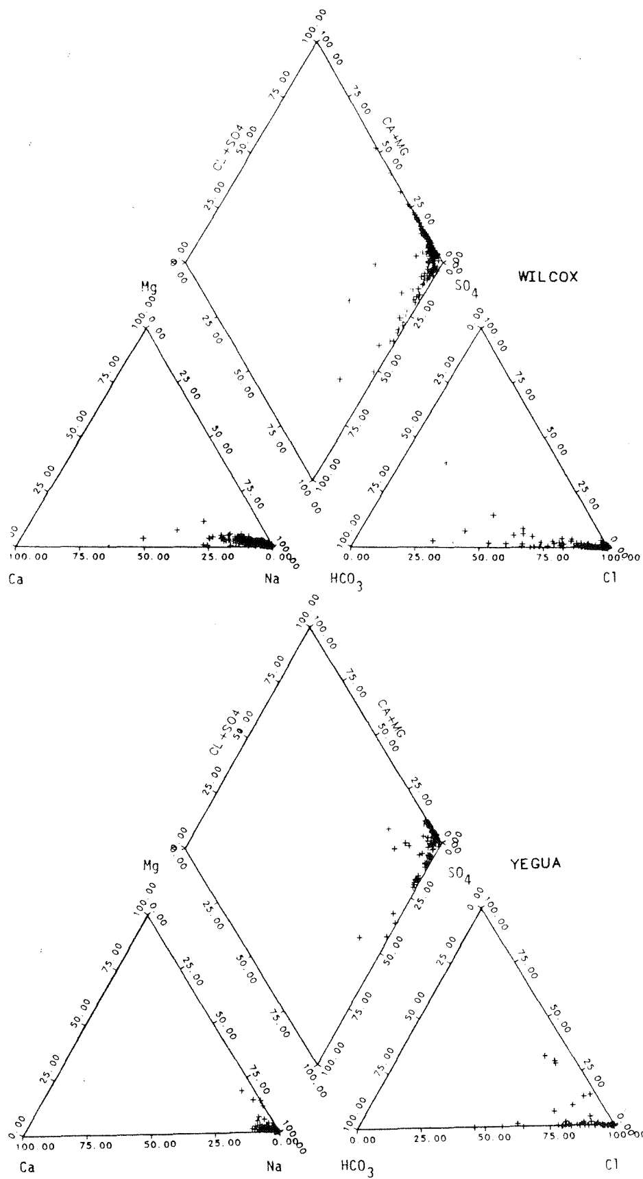
Figure 16. Piper diagrams of Yegua and Wilcox formation waters.
