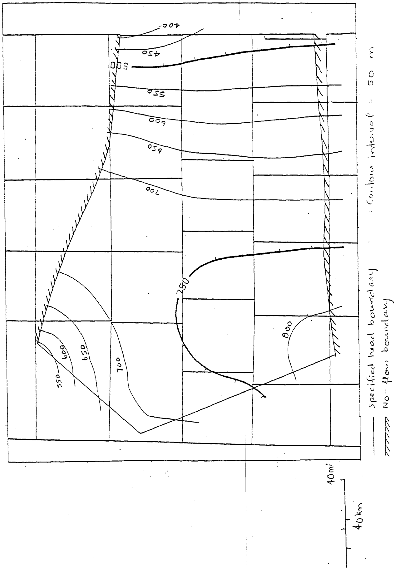
Figure 3'. Contours of computed head, Wolfcamp Aquifer Simulation A-1.
