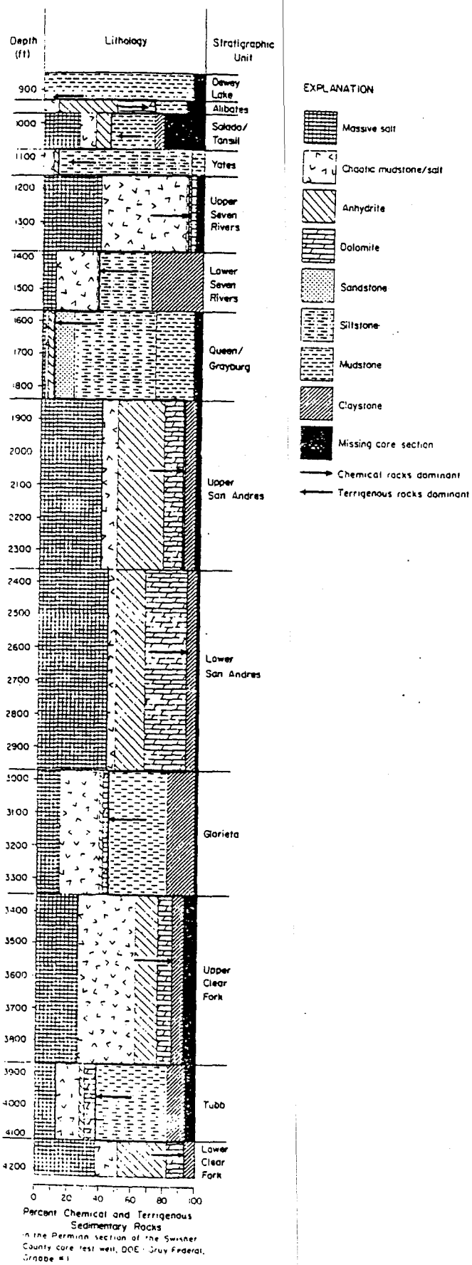
Figure 18. Swisher County core test well DOE-Gray Federal, Grabbe no. 1: percent lithologic type per stratigraphic unit (McGraw-Hill, 1964)
