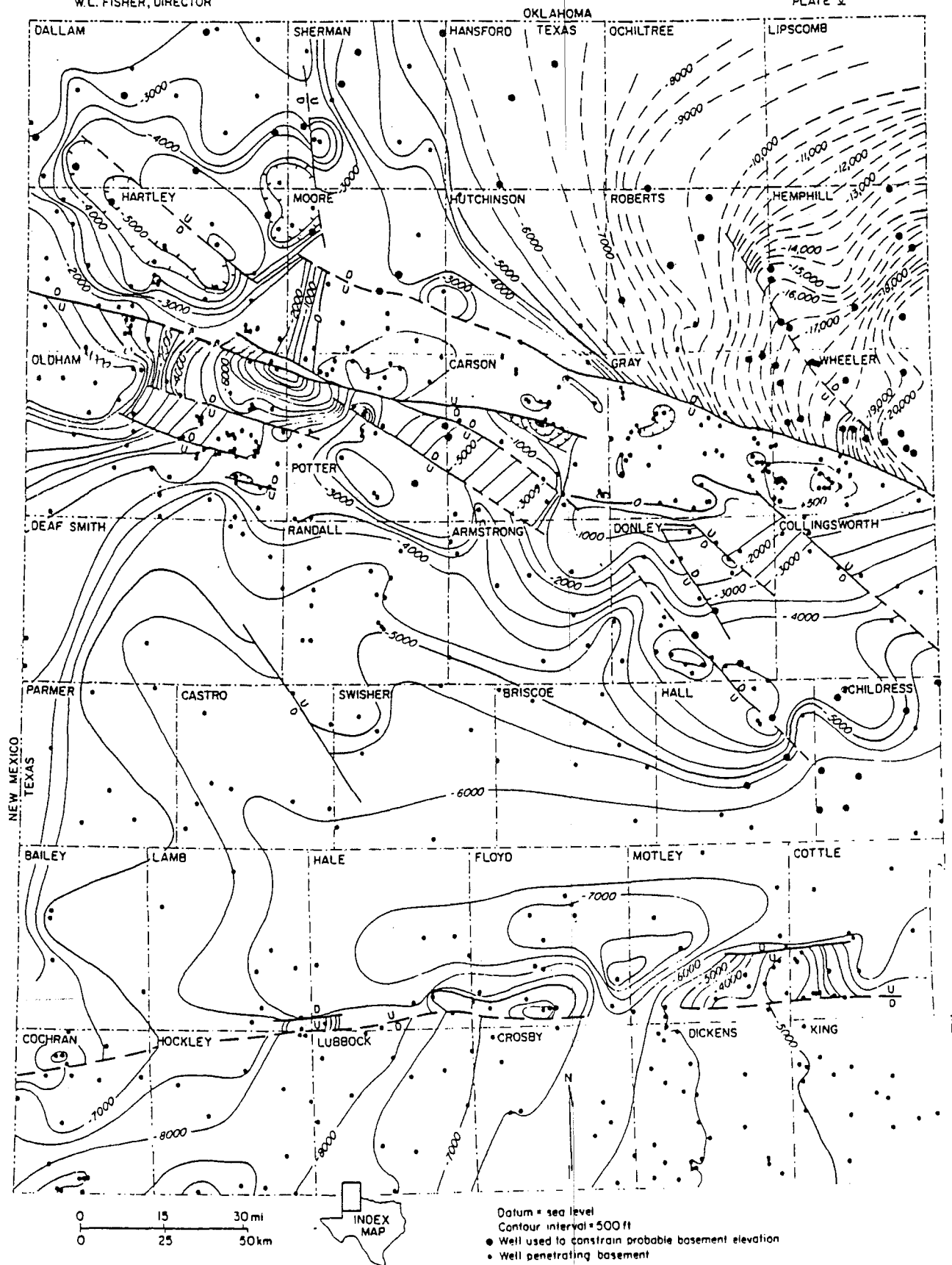
Figure 2. Structure contour map on top of crystalline basement, Texas (from Dutton and others, 1932).
