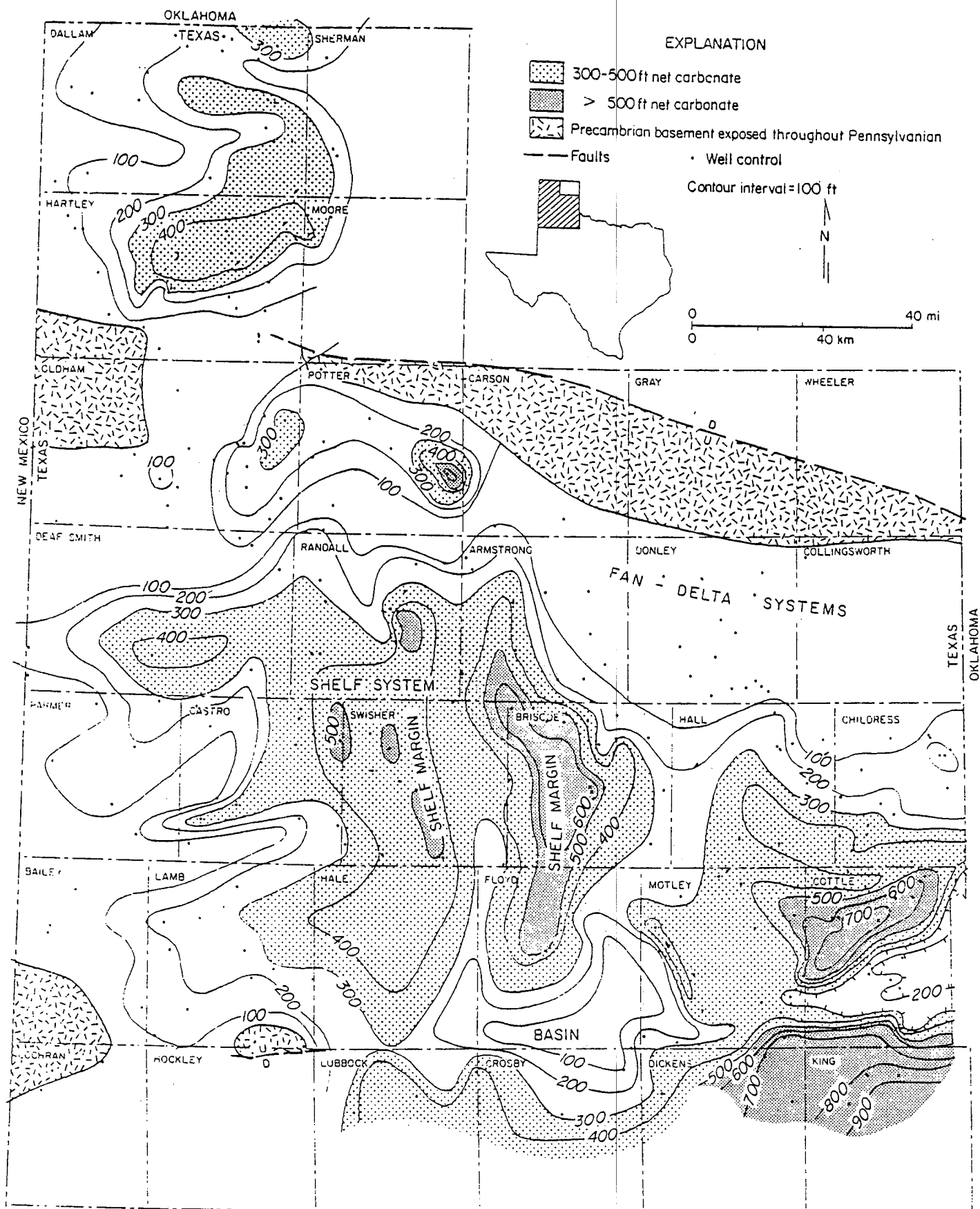
Figure 7 . Net-carbonate map of lower part of Pennsylvanian System (from DeToro, 1962).
