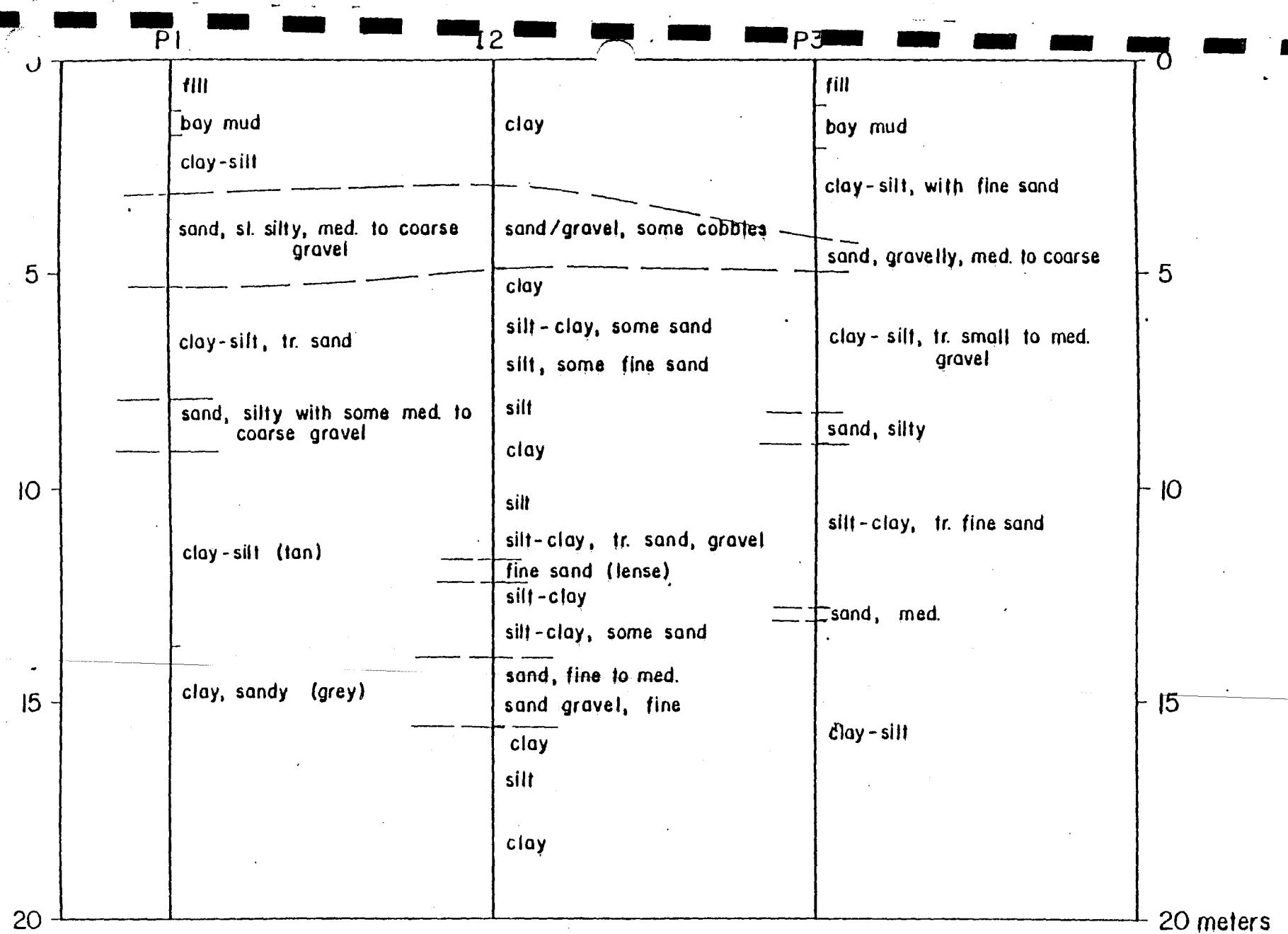
FIGURE 21. Profiles at I-2
