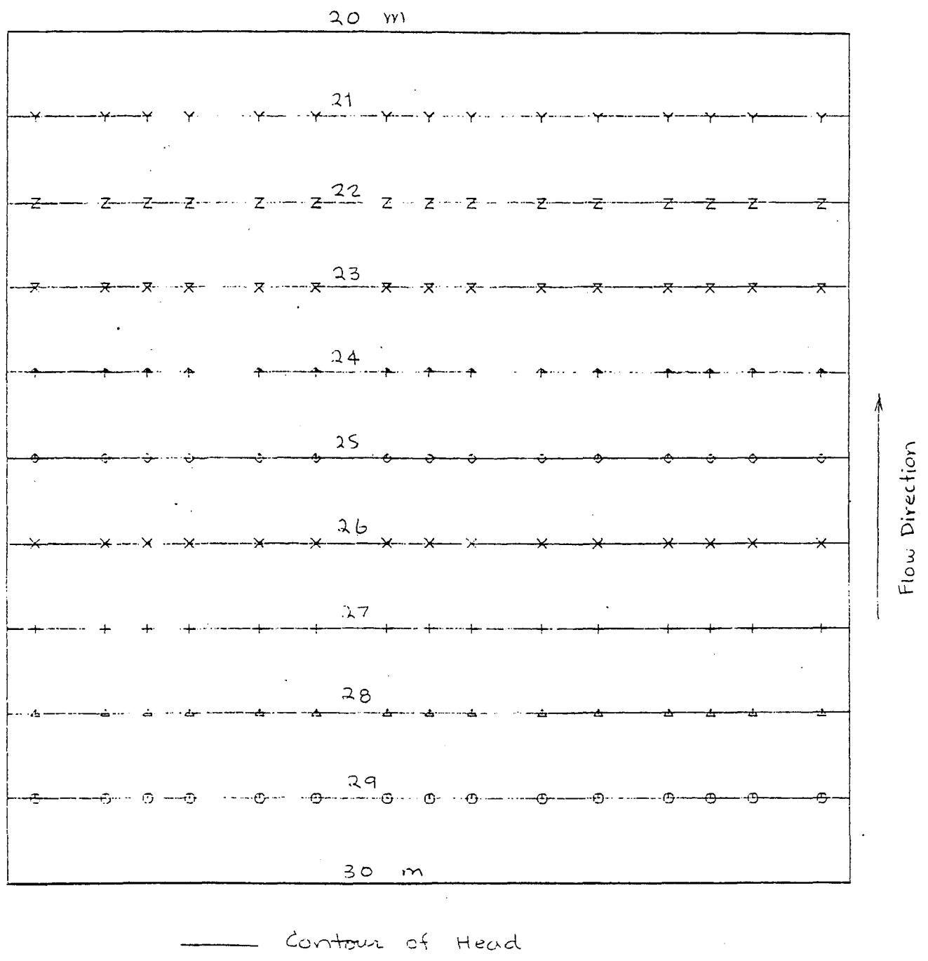
Figure 5 Sample Output - Contours of Head
