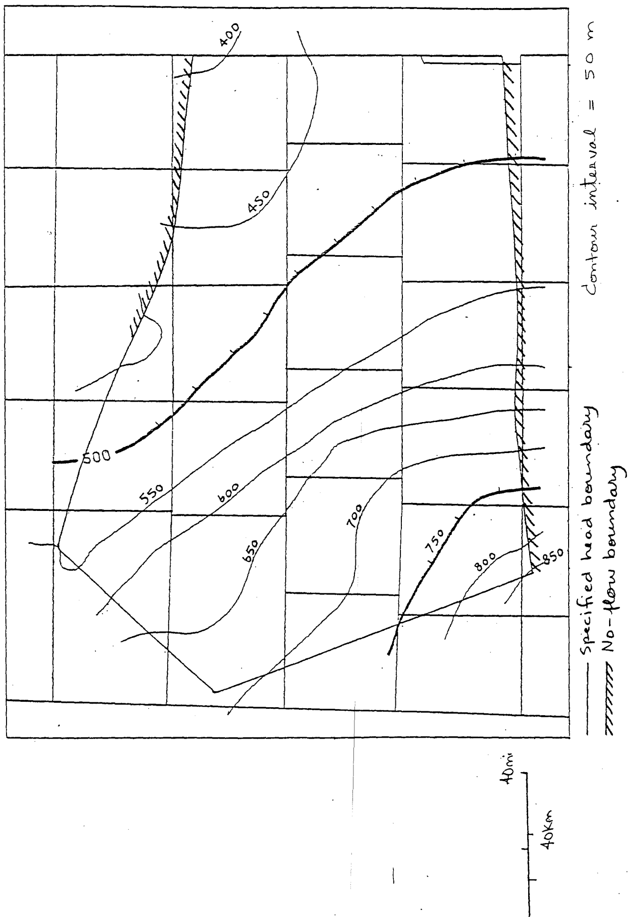
Figure 45: Contours of computed head, Wolfcamp Aquifer Simulation. E.
