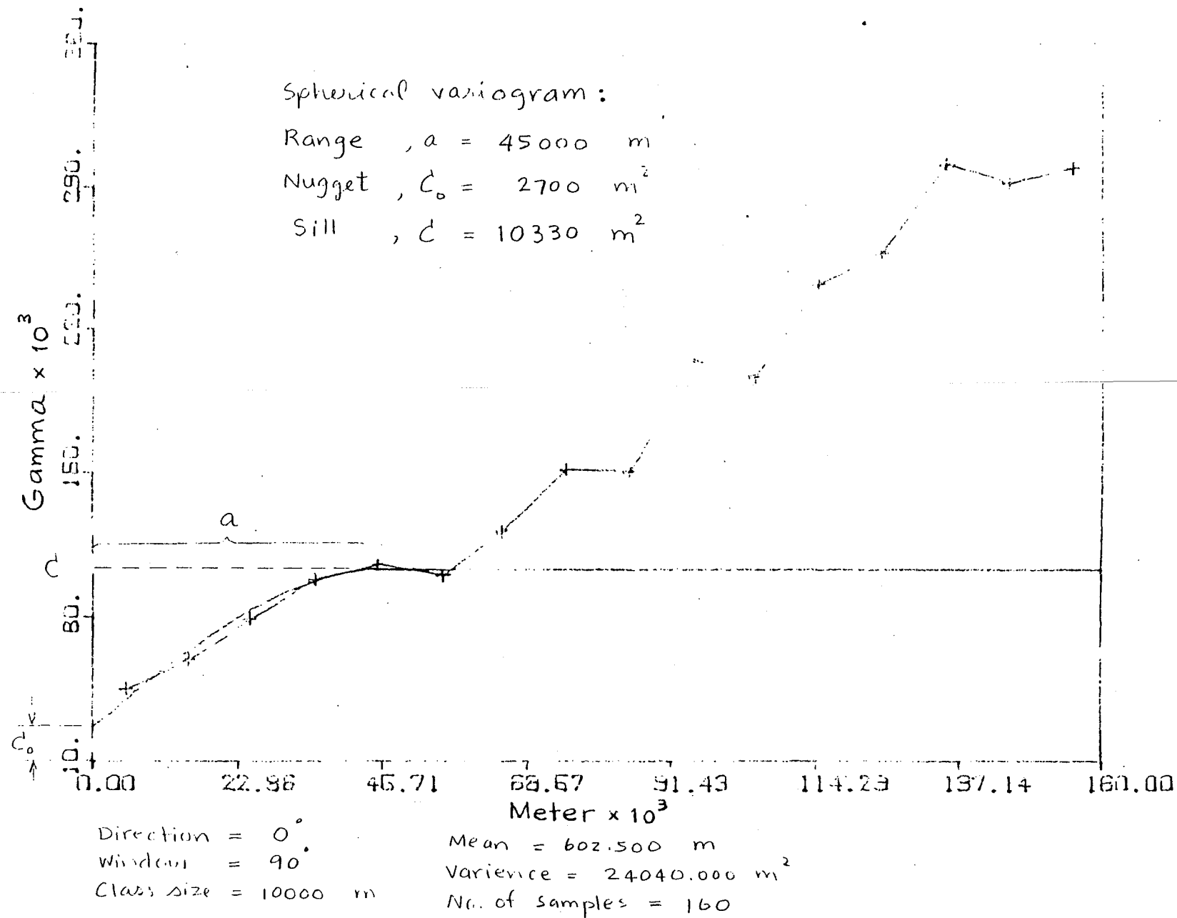
Figure 26. Representative variogram of the 118 selected class A and 42 class H average head data for the whole deep-brine aquifer.
