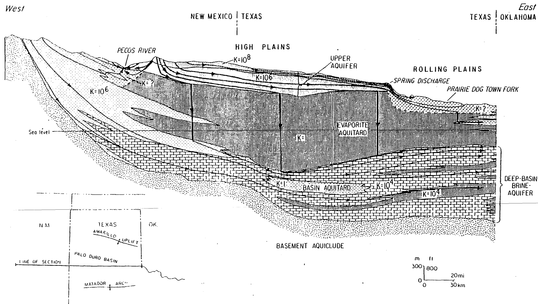
Figure 19. Regional east-west section illustrating conceptual flow patterns based on hydrologic conditions and relative permeabilities of major hydrogeologic units (after Bassett and Bentley, 1982).
