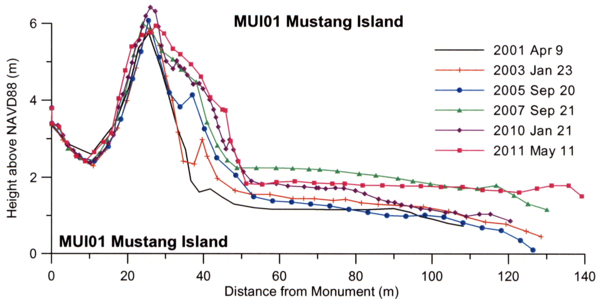
Figure 14. Foredune expansion at MUI01 on Mustang Island.
