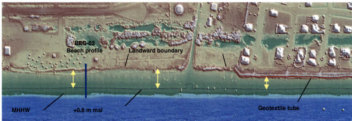
Figure 10. Lidar topographic relief image of Galveston Island State Park and Pirates Beach subdivision. Note difference in beach width between the natural beach and that in front of the subdivision.
