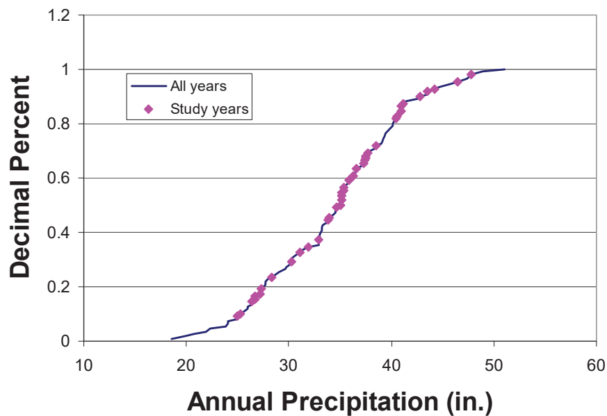
Figure 4: Cumulative Distribution of Precipitation Data for Climate Region 3
