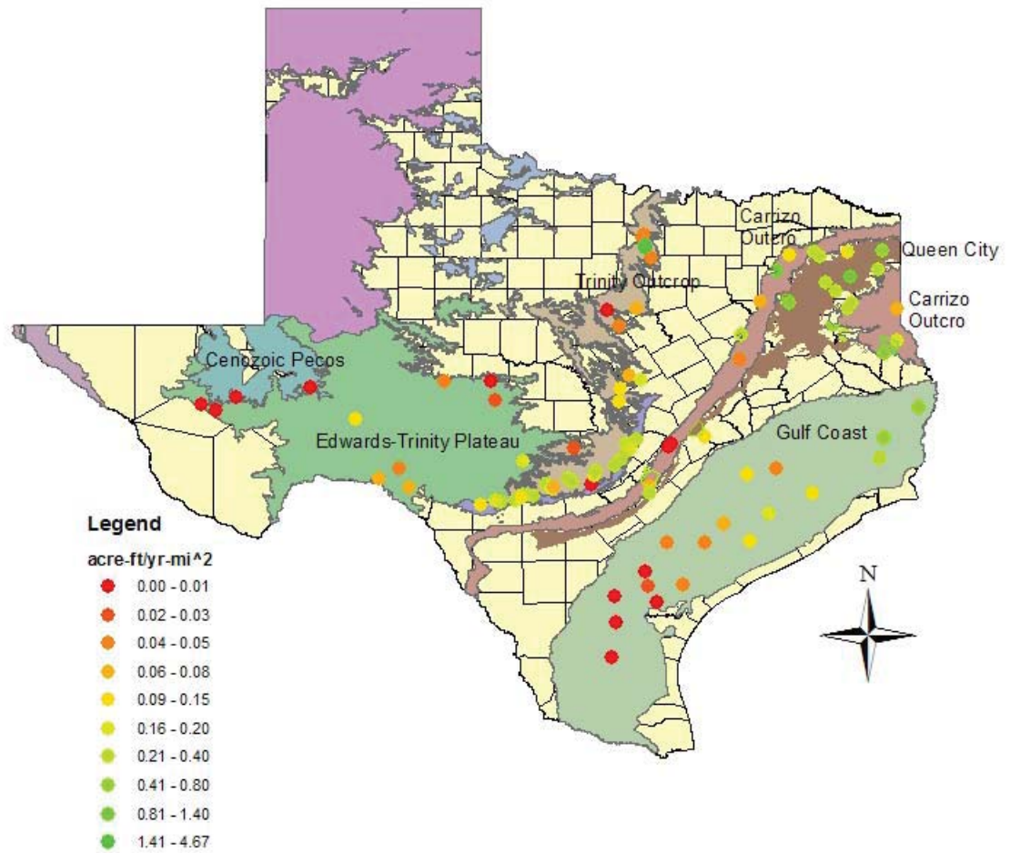
Figure 10: Spatial distribution of normalized baseflow ( \text{acre-ft/yr-mi}^2 )
