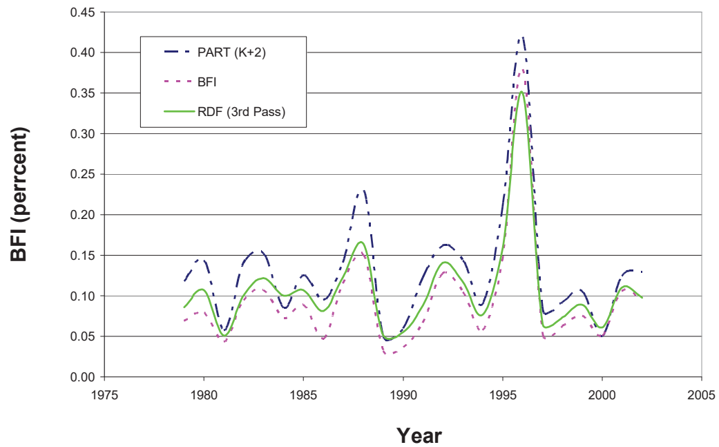
Figure 4: Methods of baseflow analysis: PART, BFI, RDF Big Creek near Freestone, TX (08110430)
