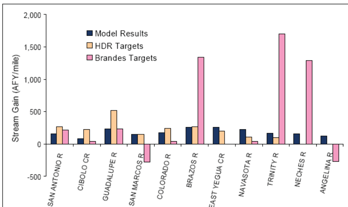
Figure 7. Comparison to measurements of steady-state model gain/loss for the central model of the Queen City GAM (from Figure 8.2.8 of Kelley et al., 2004)
