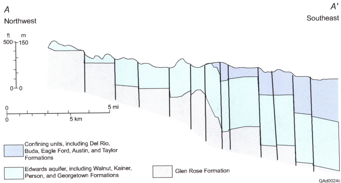
Fig. 8. Geologic cross section of the study area. Location of cross section shown in figure 7.
