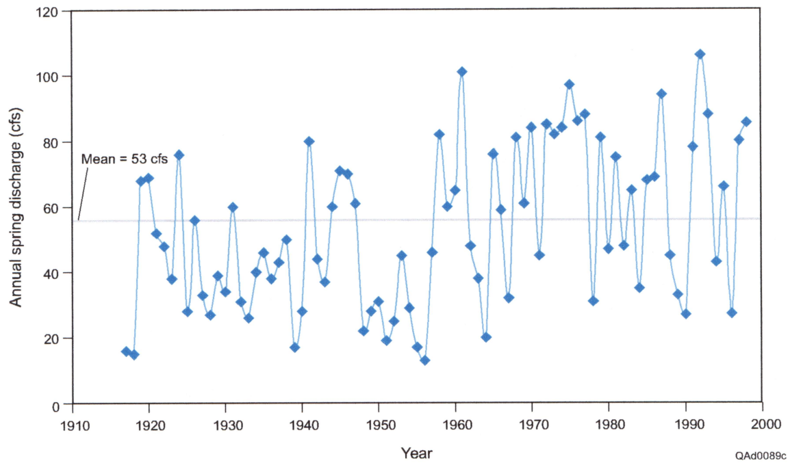
Figure 26. Discharge at Barton Springs.
