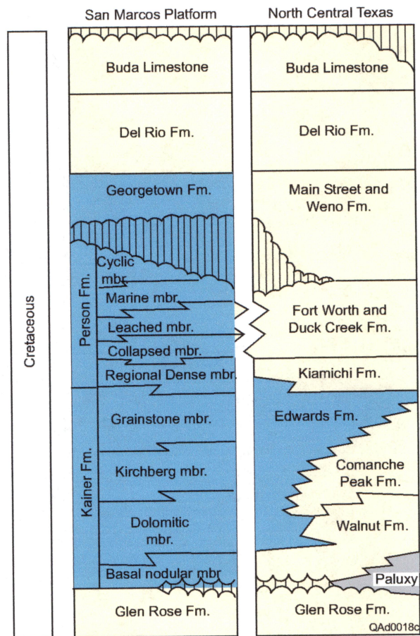
Fig. 6. Stratigraphic and hydrostratigraphic section of the study area.
