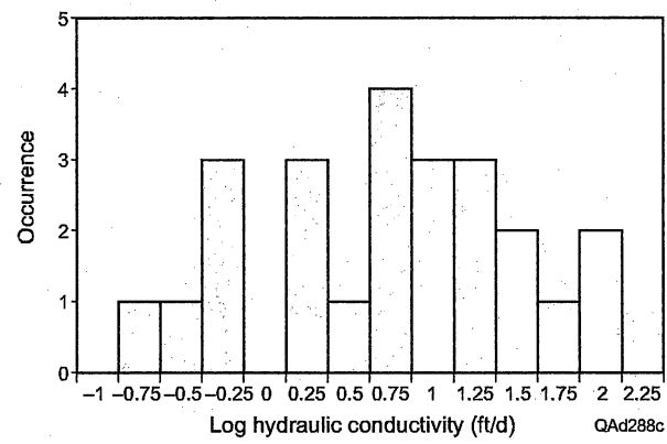
Figure 27. Histogram of hydraulic conductivity from aquifer tests.
