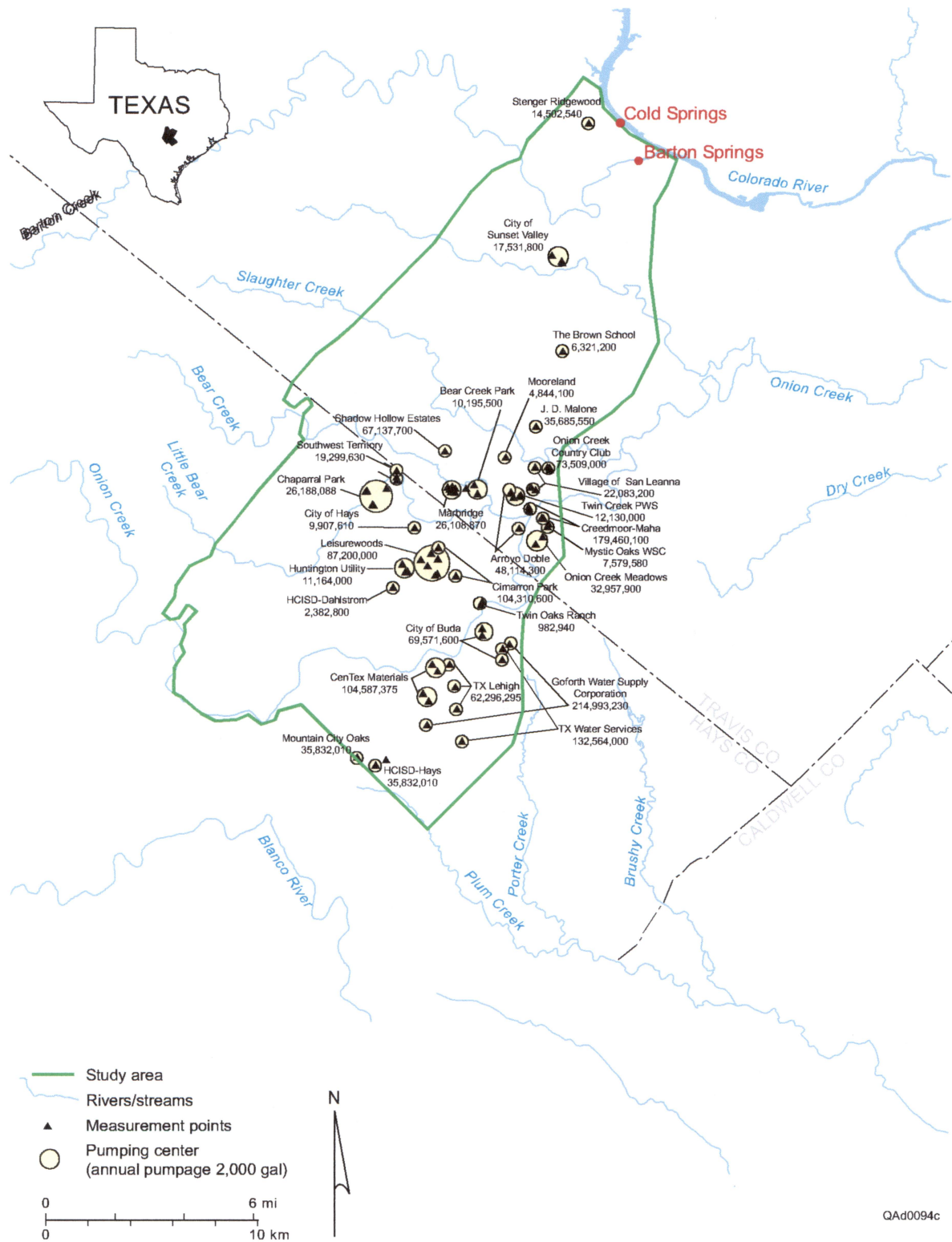
Figure 28. Spatial distribution of pumping in the aquifer.
