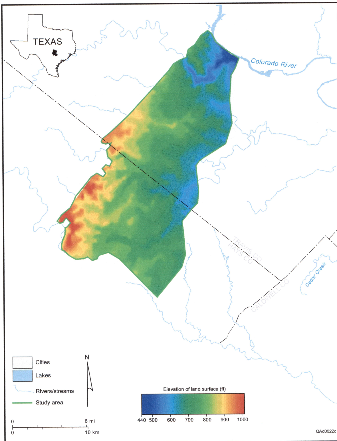
Figure 3. Land-surface elevation in the study area.
