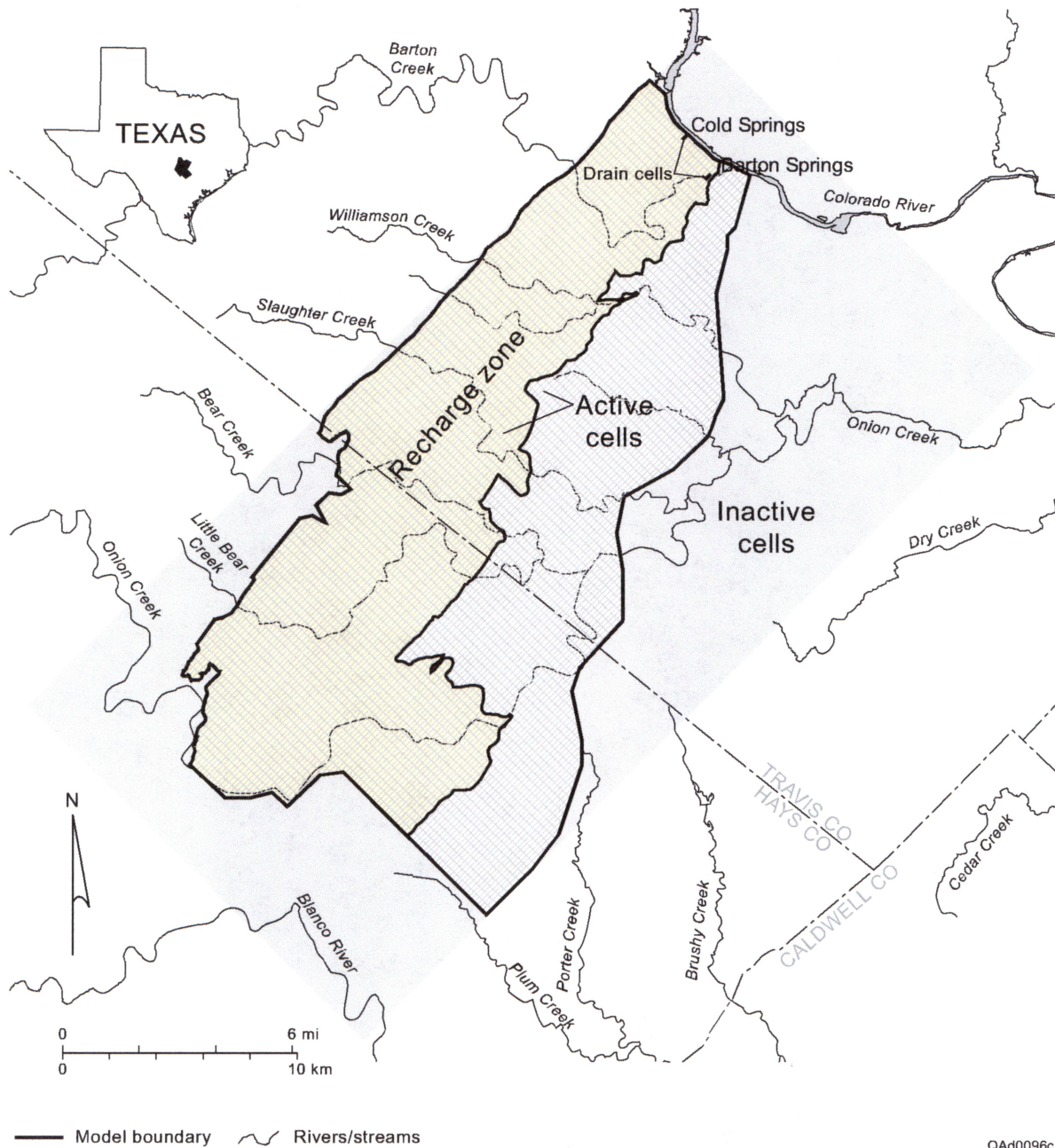
Fig. 29. Model grid, consisting of 120 cells (14,400 cells) that are 1,000 ft long 500 ft wide. The active zone of the model is shown by the solid line and consists of 7,043 cells.
