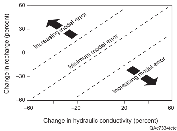
Figure 5. Diagram showing relation between change in recharge and change in hydraulic conductivity. Groundwater-model calibration using hydraulic heads only provides information on the ratio of recharge to hydraulic conductivity. Model error can be minimized using a wide range of recharge and hydraulic-conductivity values if the ratio between recharge and hydraulic conductivity is constant (modified from Luckey et al. 1986).
