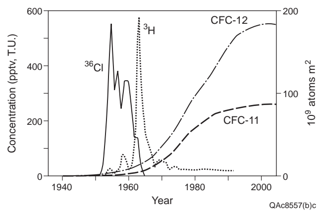
Figure 2. Input functions for historical tracers, including ^3H , ^{36}Cl , CFC-11 and CFC-12 ( ^3H data from Ottawa, Canada; ^{36}Cl data, Phillips 2000; CFC data, http://water.usgs.gov/lab/cfc/background/air_curve.html ).
