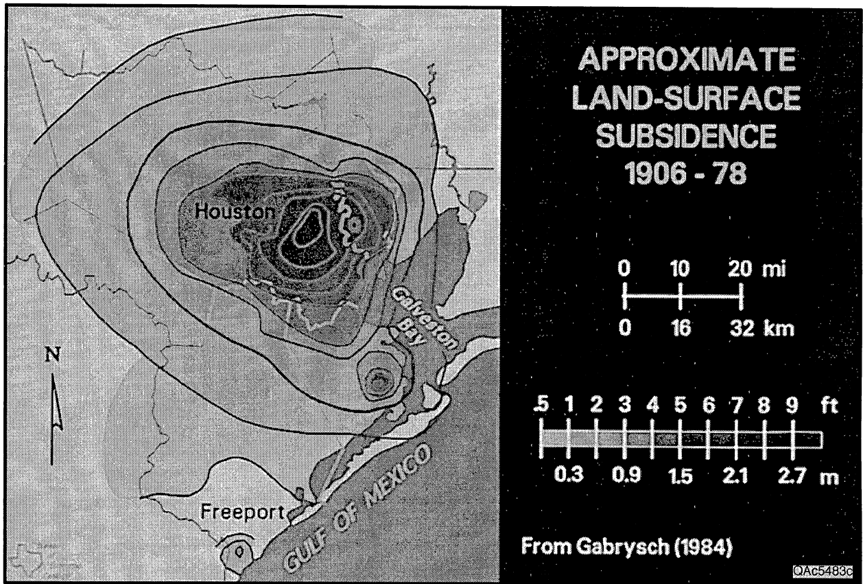
Figure 7. Land surface subsidence in the Houston-Galveston area from 1906-1978. (26)
