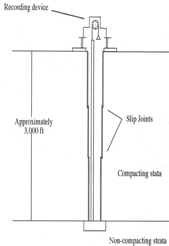
Figure 10. Illustration of a typical borehole extensometer. The inner rigid pipe maintains its position with respect to the outer segmented pipe and surface installation, which become lower as subsurface strata compact. The amount of compaction or shortening is measured by the wire tape rolling over the drum. (27)
