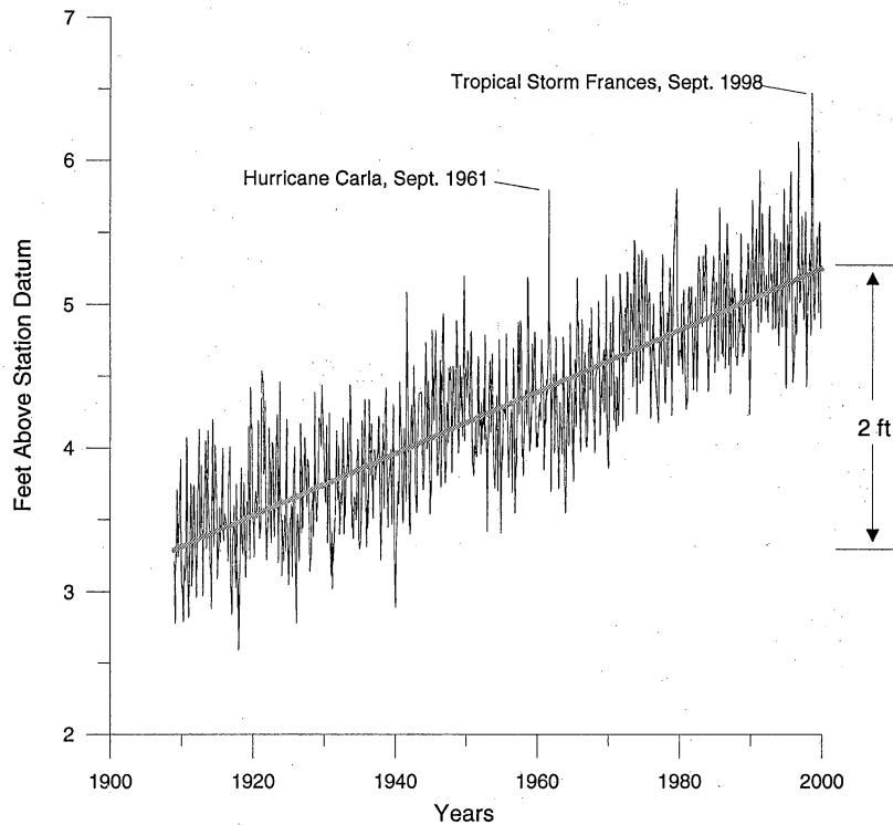
Figure 2. Monthly average sea level since 1909 as measured by the Pier 21 tide gauge in Galveston Bay. Straight line is a linear regression through all the data points.
