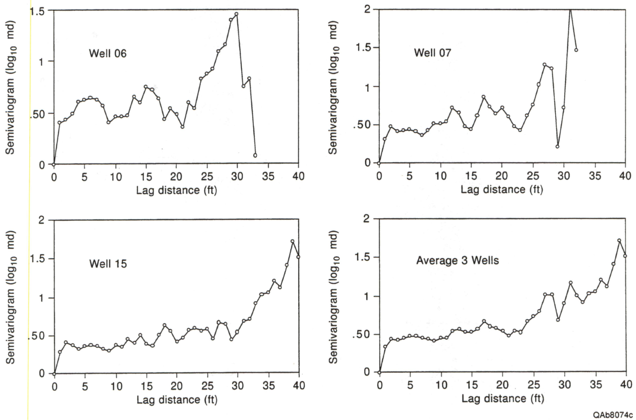
Figure 45. Vertical semivariograms for core-analysis permeability for wells FGU 6, 7, and 15 in the demonstration area, and the average for all three wells. Location of wells shown in figure 46.
