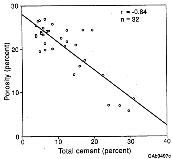
Figure 32. The main controls on porosity and permeability in the Ramsey sandstones are authigenic cements, particularly calcite, and, to a lesser extent, chlorite.
