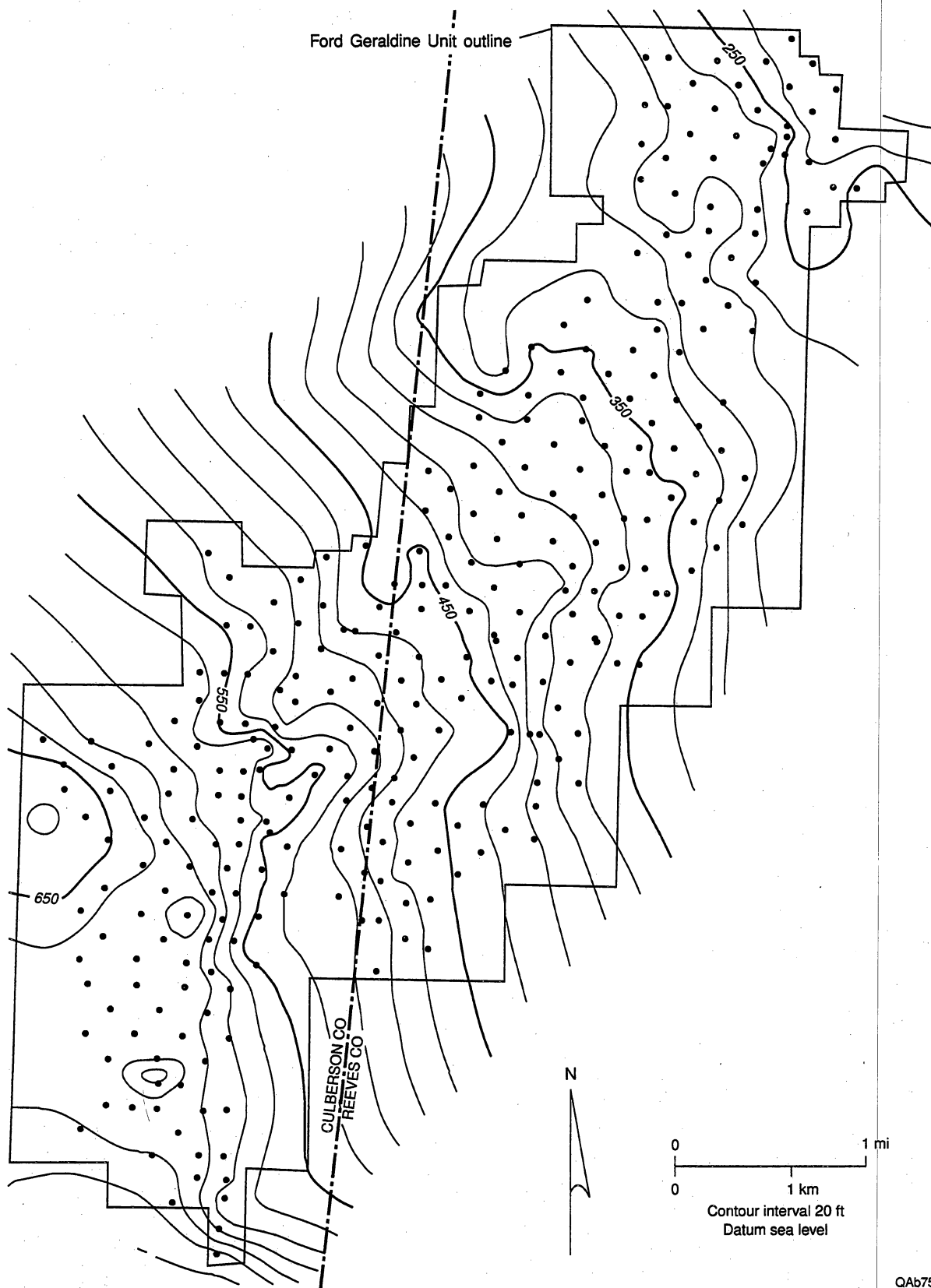
Figure 15. Structure contours on the top of the Lamar limestone dip to the east and northeast. The trap at Geraldine Ford field is formed by pinchout of permeable sandstone into low-permeability siltstone structurally updip. The field has minor structural closure because of differential compaction over the reservoir sandstone body.
