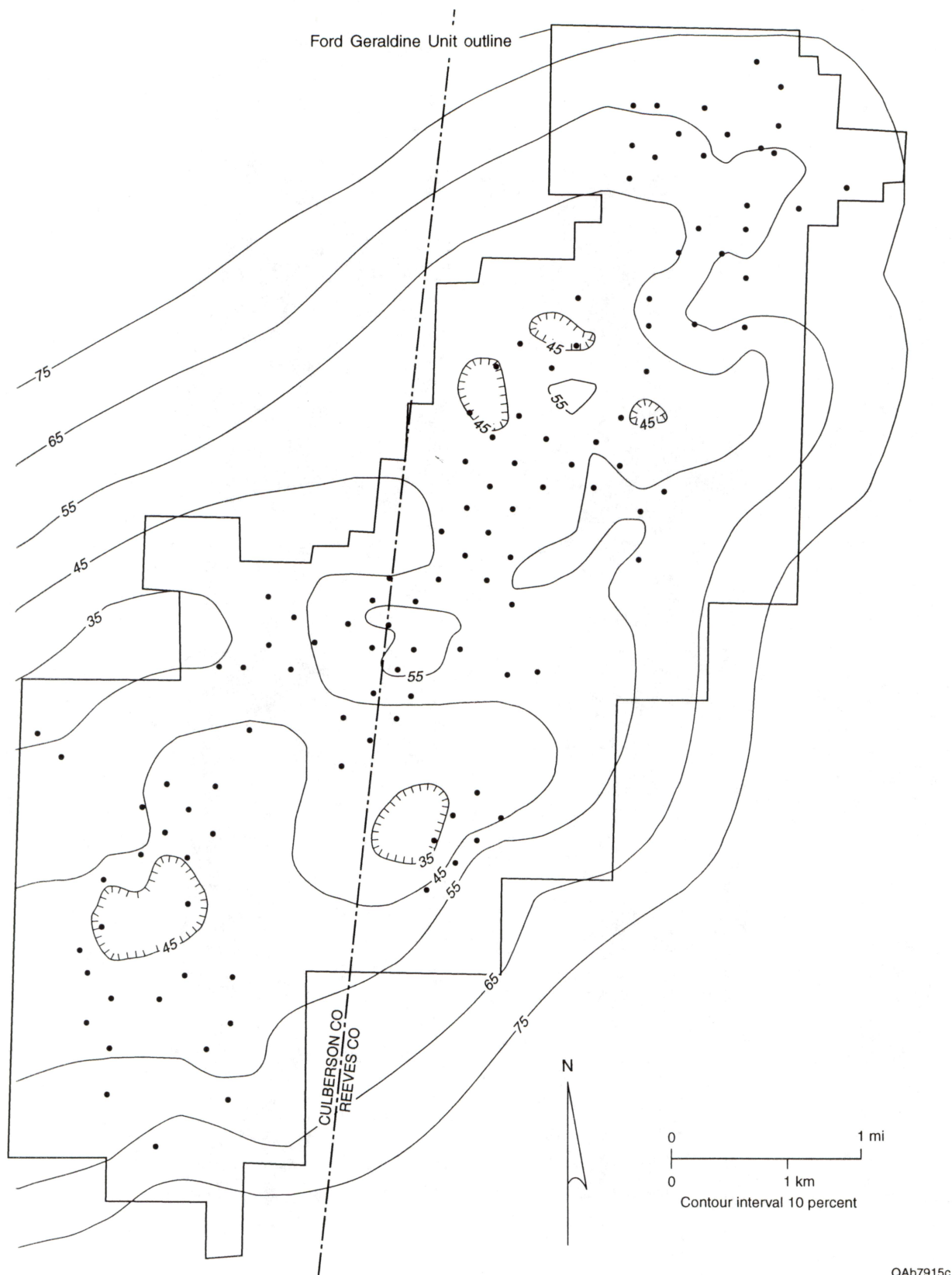
Figure 73. Map of water saturation ( S_w ) for the Ramsey sandstone in the Ford Geraldine unit, Reeves and Culberson Counties, Texas. The water saturations ( S_w ) in the northeast part of the unit were calculated from the average BVW values by the formula S_w = BVW_{avg}/\phi .
