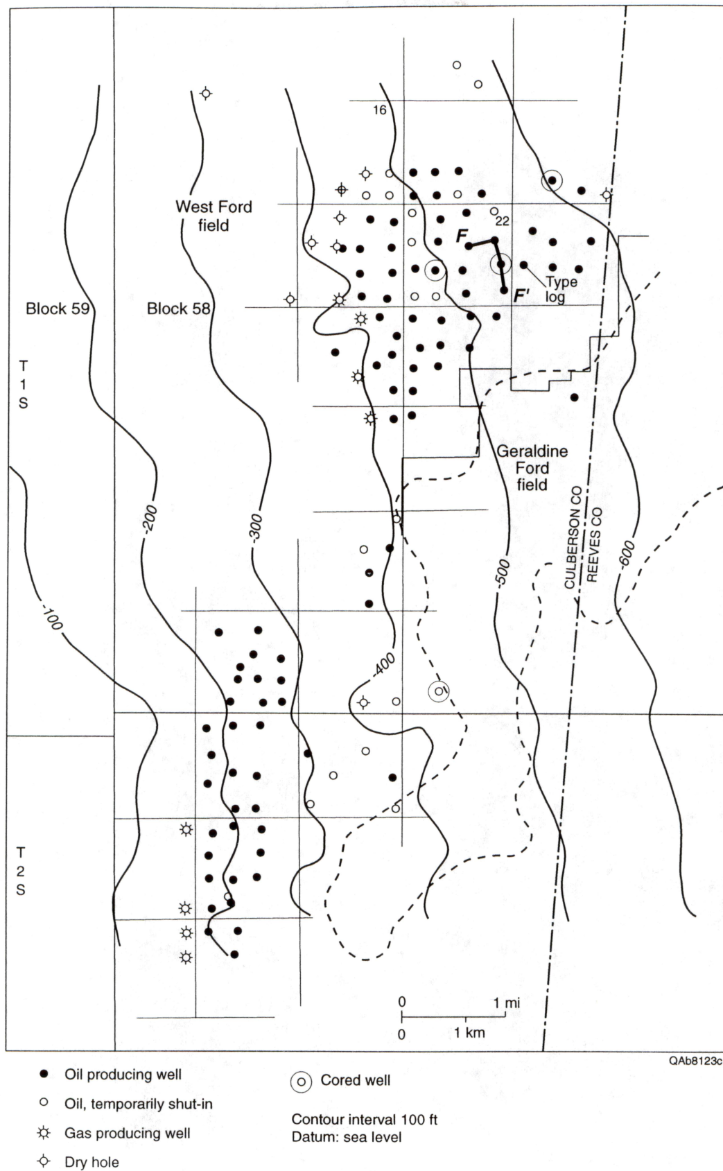
Figure 51. Location map of Ford West field, which produces from the upper Cherry Canyon Formation and lowermost Bell Canyon Formation, Delaware Mountain Group (modified from Linn, 1985). Three cores were described from Ford West field. Cross section F–F' shown in figure 52, and type log shown in figure 7.
