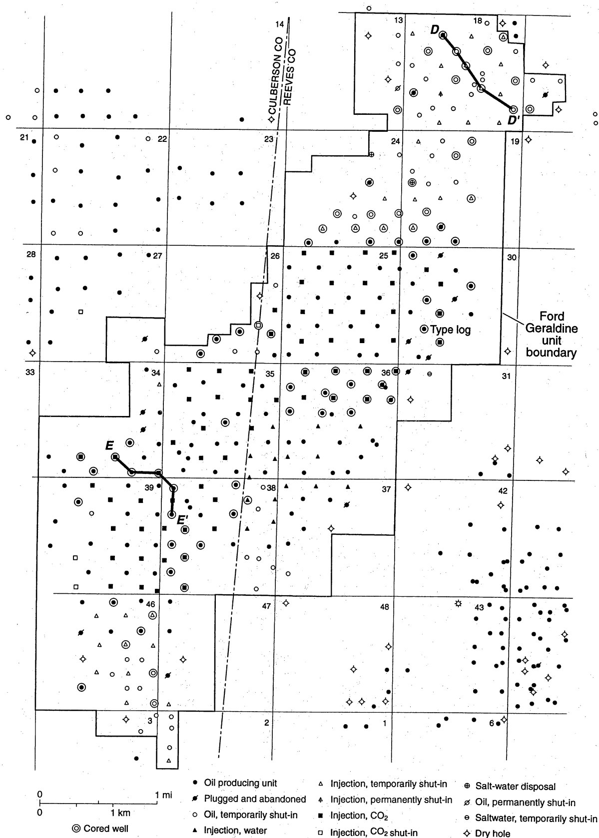
Figure 6. Status of wells in the Ford Geraldine unit and distribution of core control. Type log is shown in figure 5, cross section D–D' in figure 39, and cross section E–E' in figure 40.
