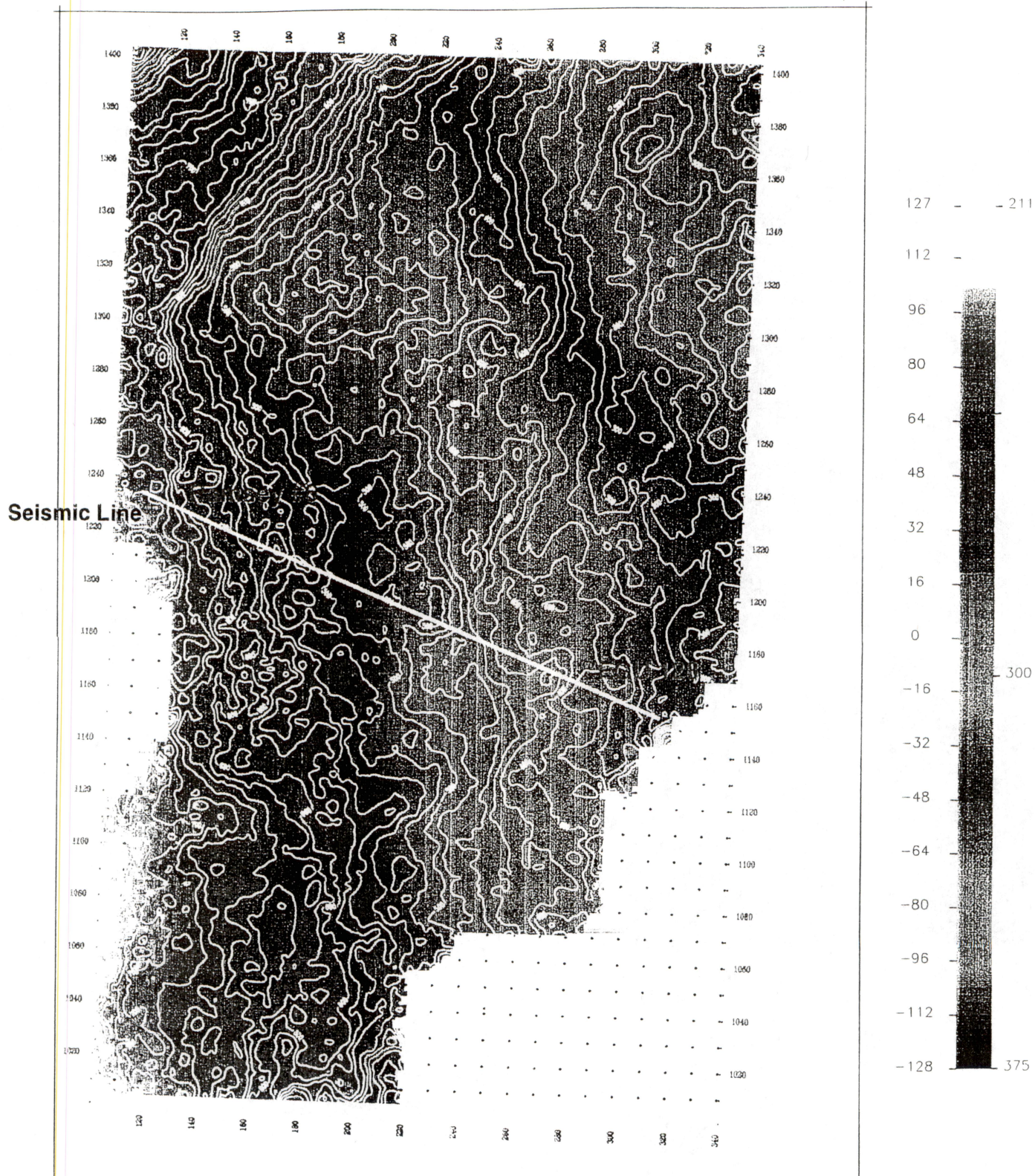
Figure 82. Top of Lamar interval in time showing location of the wells with synthetic seismograms (Conoco G. E. Ramsey No. 6 and FGU-128) and the location of the representative seismic line shown in figure 83.
