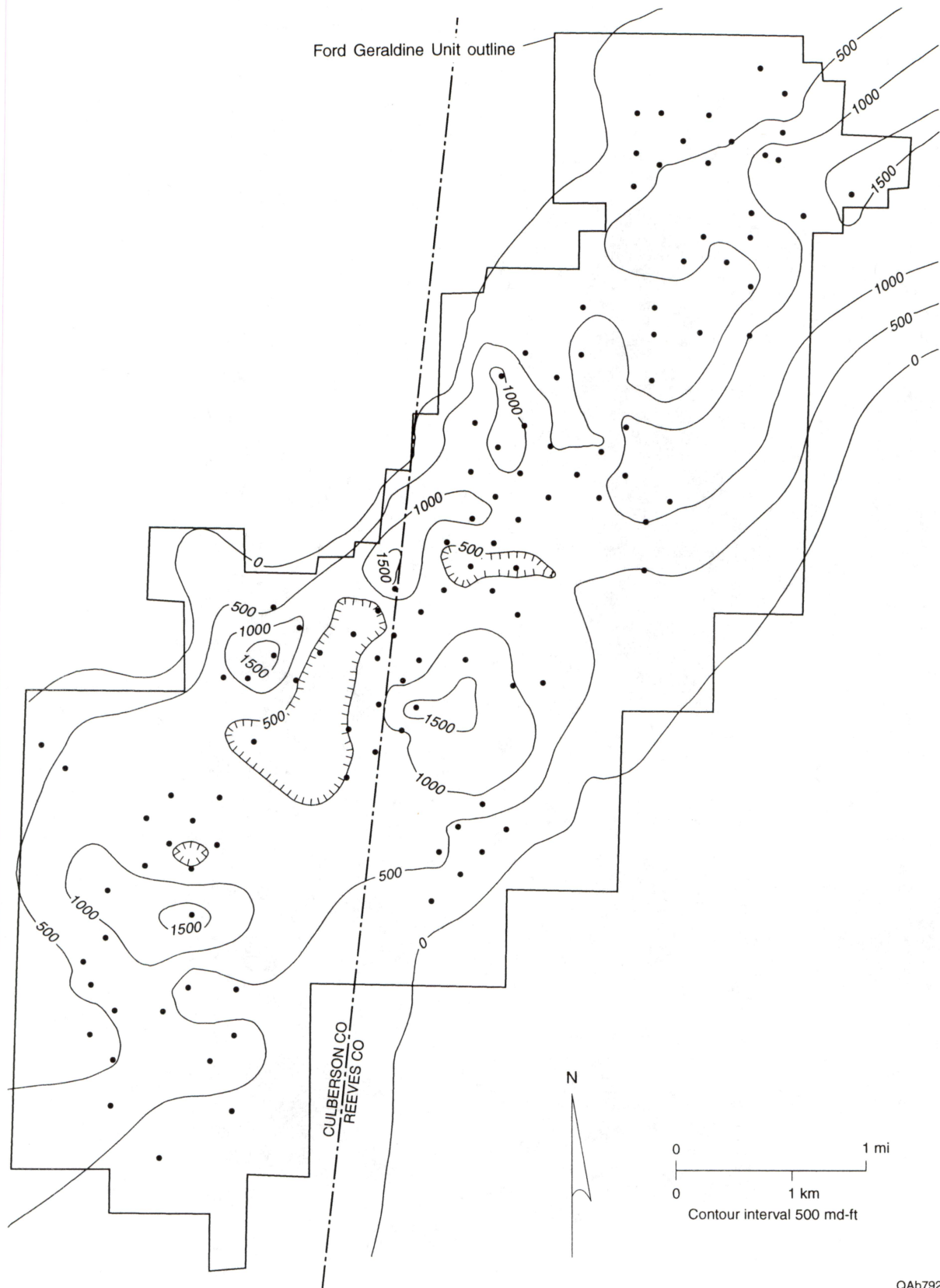
Figure 71. Map of permeability × thickness for the Ramsey sandstone in the Ford Geraldine unit, Reeves and Culberson Counties, Texas. The linear trend of high permeability-feet (>1,000) to the northeast breaks up to isolated "pods" of high permeability-feet to the southwest.
