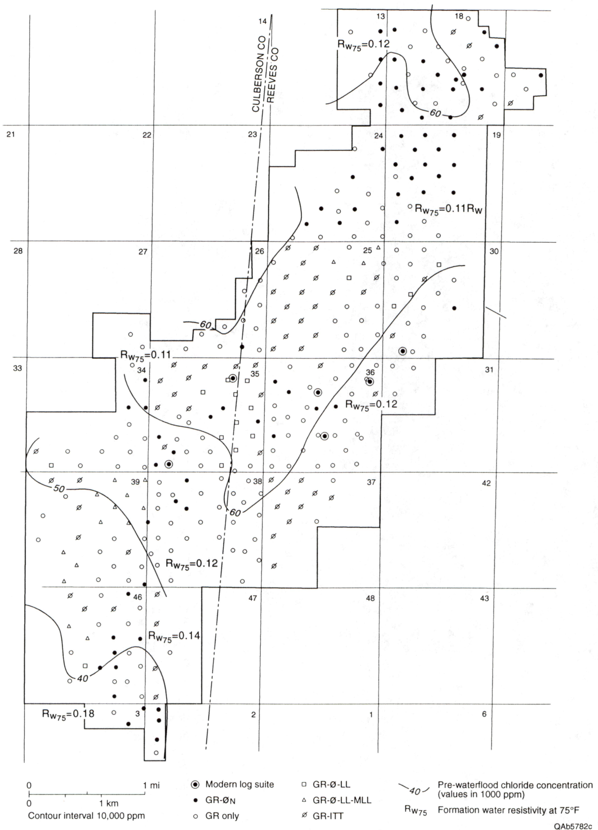
Figure 60. Prewaterflood isosalinity map with formation water resistivities ( R_w ) at 75°F for the Ford Geraldine unit. Modified from Ruggiero (1985).
