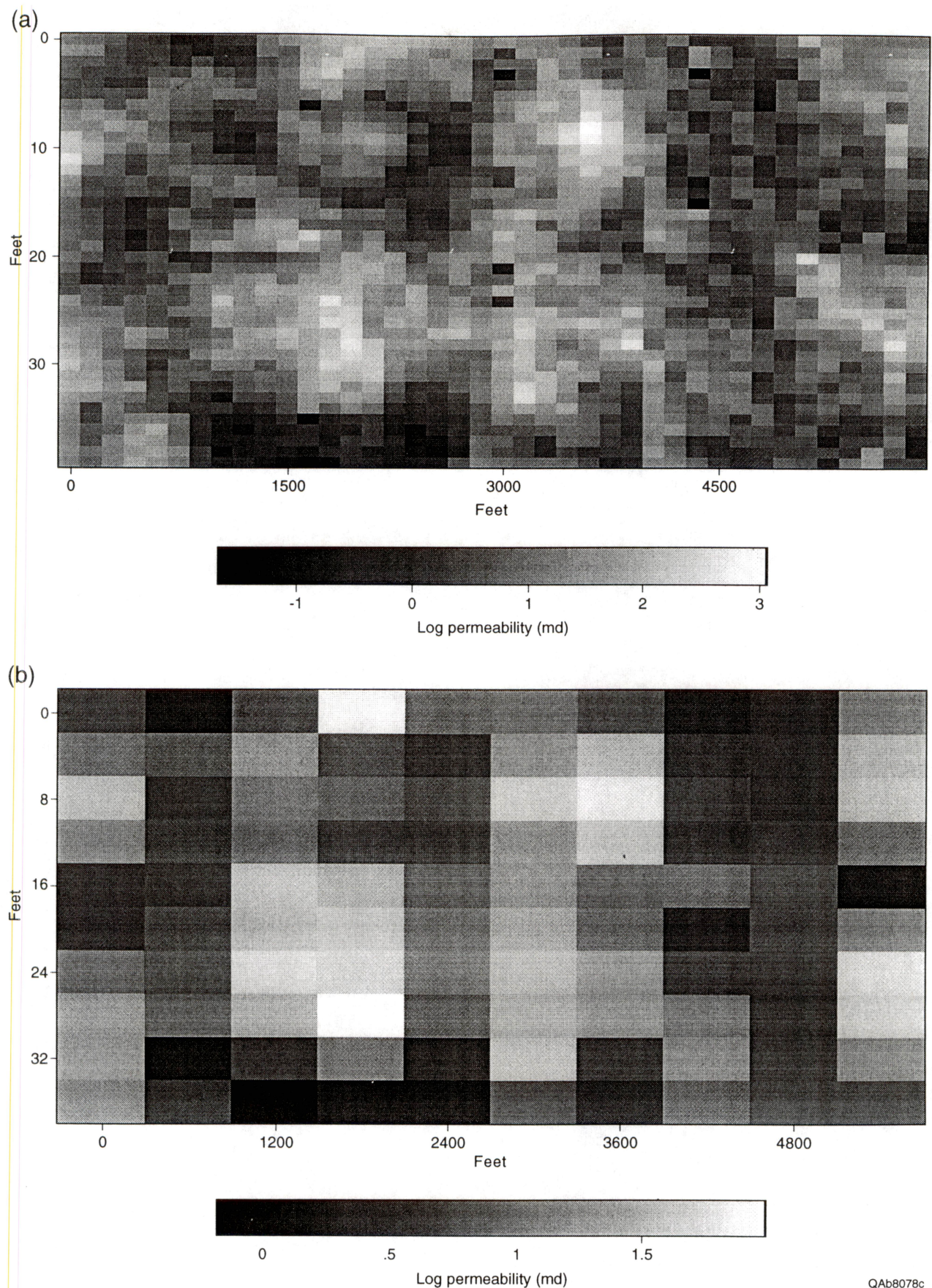
Figure 96. Vertical cross section showing permeability distribution along line of section H-H' (fig. 4); permeabilities are from the 3-D permeability distribution. (a) Fine-scale permeability distribution in a 40 \times 40 block, with a grid-block size of 150 ft in the horizontal direction and 1 ft in the vertical direction. (b) Scaled-up permeability distribution in a 10 \times 10 block after performing a 3-D, 4 \times 4 \times 4 scale-up.
