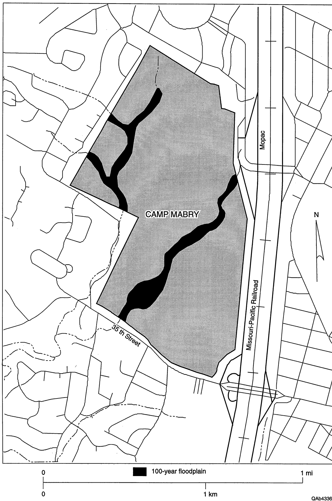
Figure 16. One-hundred-year floodplains of Camp Mabry.
