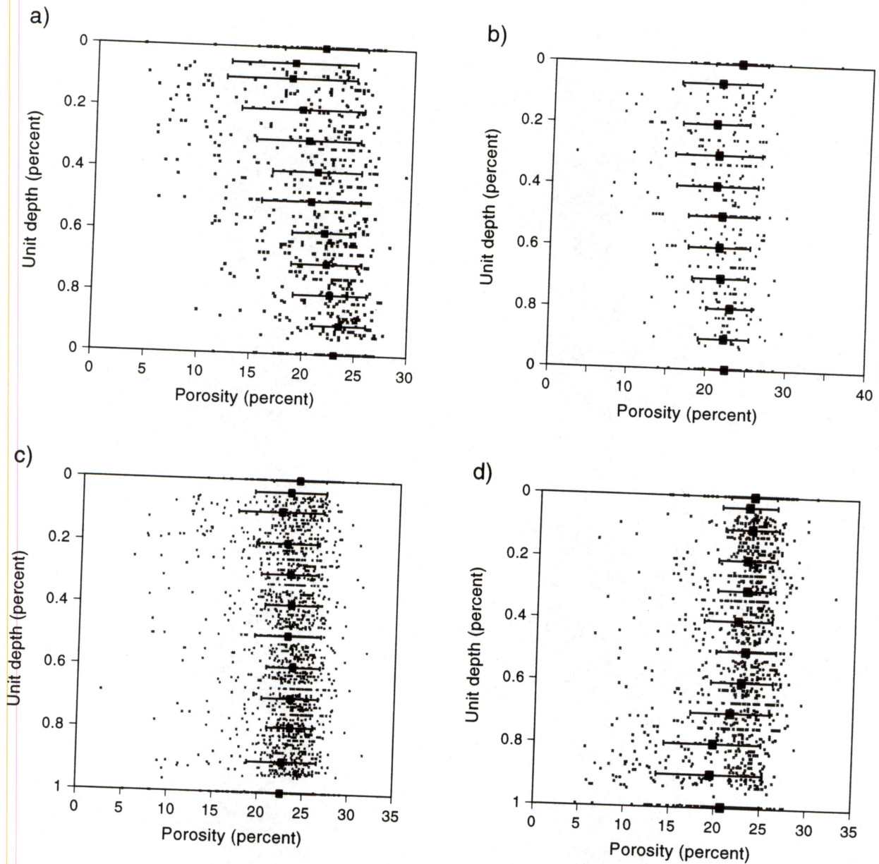
Figure 33. Plots of porosity from core analysis versus relative position in each Ramsey sandstone. Depths were normalized to give each stratigraphic interval a thickness of one. (a) Ramsey 2 sandstone. (b) Ramsey 1C sandstone. (c) Ramsey 1B sandstone. (d) Ramsey 1A sandstone.
