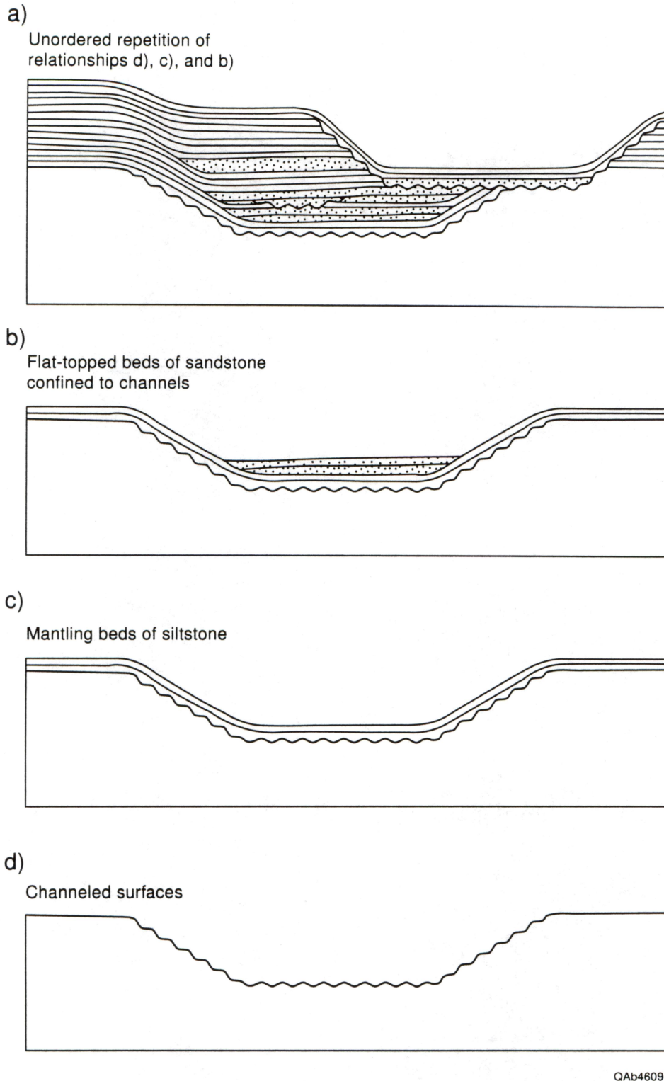
Figure 16. Interpreted sequence of events during deposition of Delaware Mountain Group sediments by saline-density currents (modified from Harms, 1974). In this model, channels (d) were scoured by strong currents of dense water flowing basinward under less dense, deep water. Deposition of silt (c) occurred by settling from intermediate density water flowing basinward into density-stratified, deep water. The final stage of the sequence (b) was deposition within preexisting channels of sand tractionally carried by thin, upper-to-lower flow regime currents of dense, low turbidity water flowing basinward under less dense, deep water.
