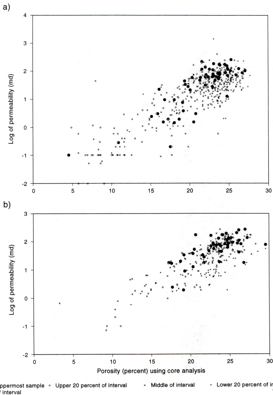
Figure 36. Plots of porosity versus the log of the permeability from core analysis. Symbols show the relative position of the sample in each Ramsey sandstone. (a) Ramsey 2 sandstone. (b) Ramsey 1C sandstone.
