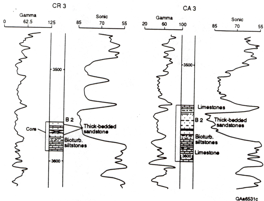
Figure 12. Core descriptions and log responses of the producing Cherry Canyon interval in Ford West field (from Linn, 1985). Location of wells shown in figure 18.
