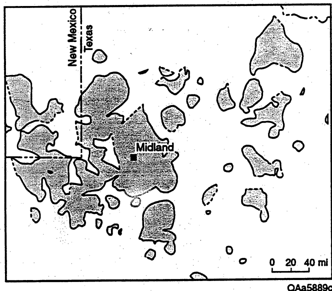
Figure 30. Composite map of all positive residuals in greater Permian Basin; boundaries dashed where inferred.
