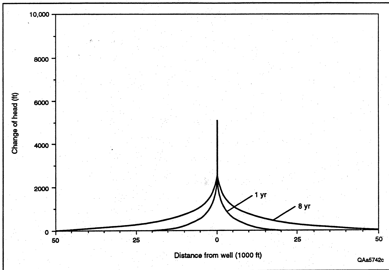
Figure 43. Calculated hydraulic-head buildup around well in enhanced-recovery injection project F0004, South Texas Basin.
