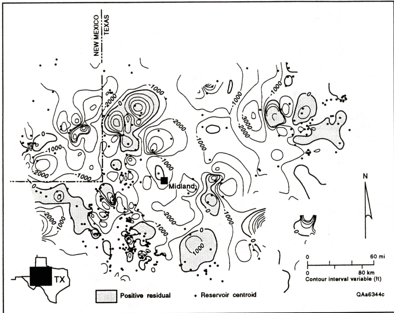
Figure 28. Residual of computer-generated potentiometric surface of Permian reservoirs <10,000 ft (<3,000 m) deep minus computer-generated potentiometric surface of Cenozoic USDWs, greater Permian Basin. Stippled areas represent positive residuals adequately supported by nearby data points.
