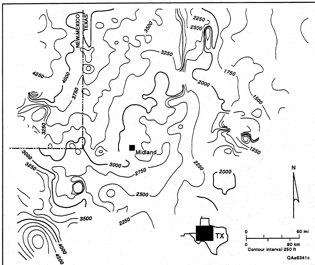
Figure 27. Computer-generated potentiometric surface of combined Cenozoic USDWs, greater Permian Basin.
