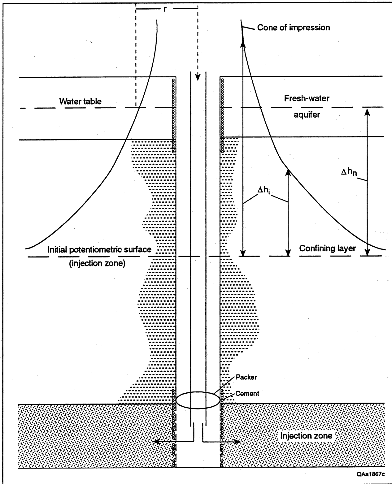
Figure 5. Schematic representation of the cone of impression around an injection well and its influence on the radius (r) of the area of review; \Delta h_n = "natural" (pre-injection) head difference between injection zone and USDW; \Delta h_i = head buildup due to injection (after Engineering Enterprises, Inc., 1988, fig. 3-1).
