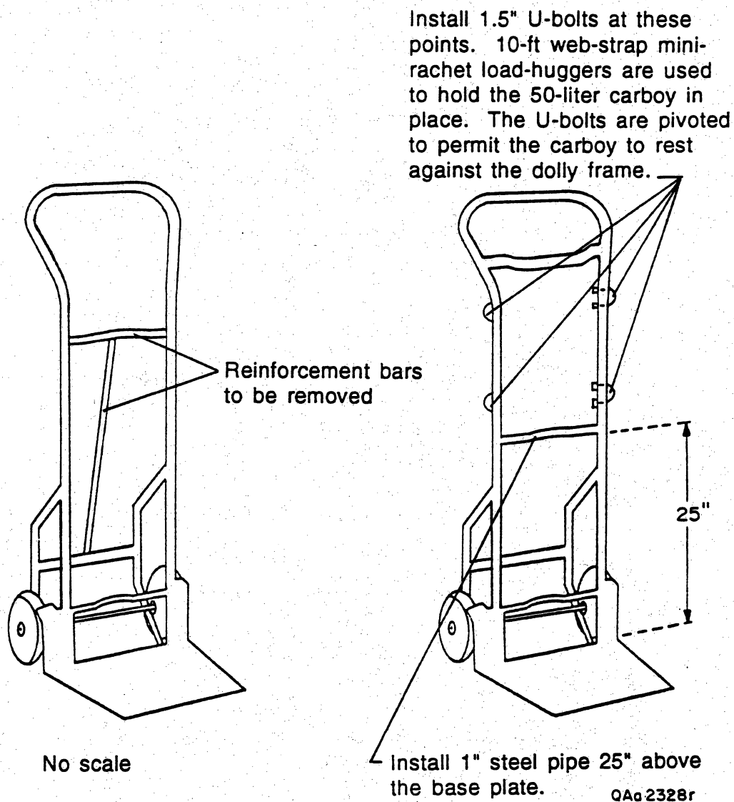
Figure A3. Illustrations of modifications of a heavy-duty hand truck for inverting a 50-L carboy.
