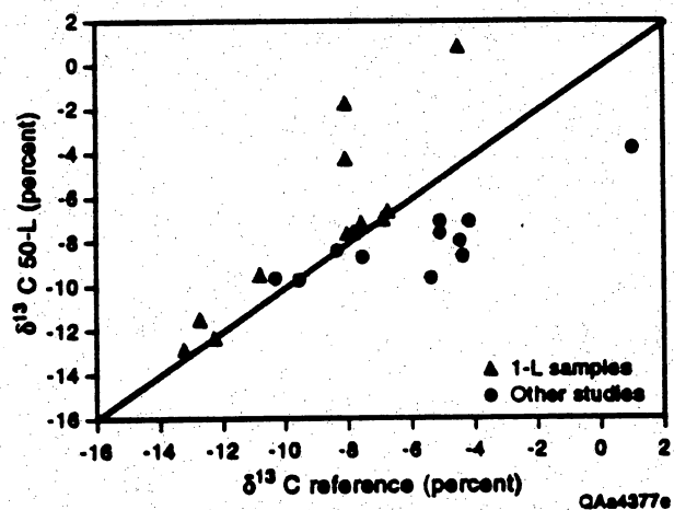
Figure A7. Comparison of \delta^{13}\text{C} in samples collected in 50-L carboys with reference \delta^{13}\text{C} data—samples collected during this study in 1-L glass bottles using direct precipitation and samples collected during other studies in a 200-L steel tank using direct precipitation and in 1-L glass bottles without field treatment.
