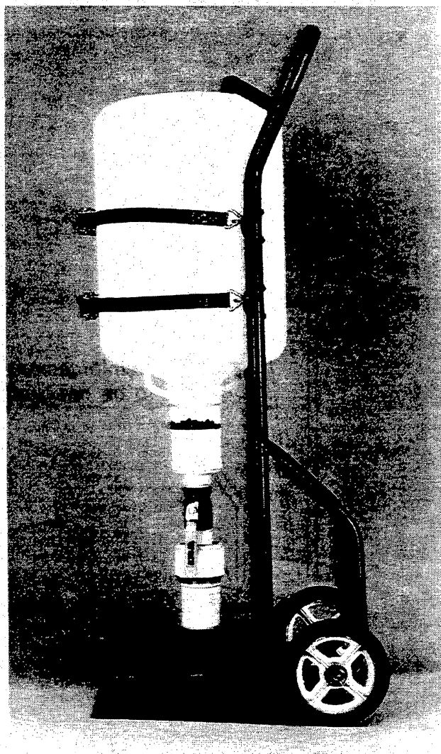
Figure A4. (a) Front and (b) side views of a heavy-duty hand truck holding an inverted 50-L carboy with sample jar.
