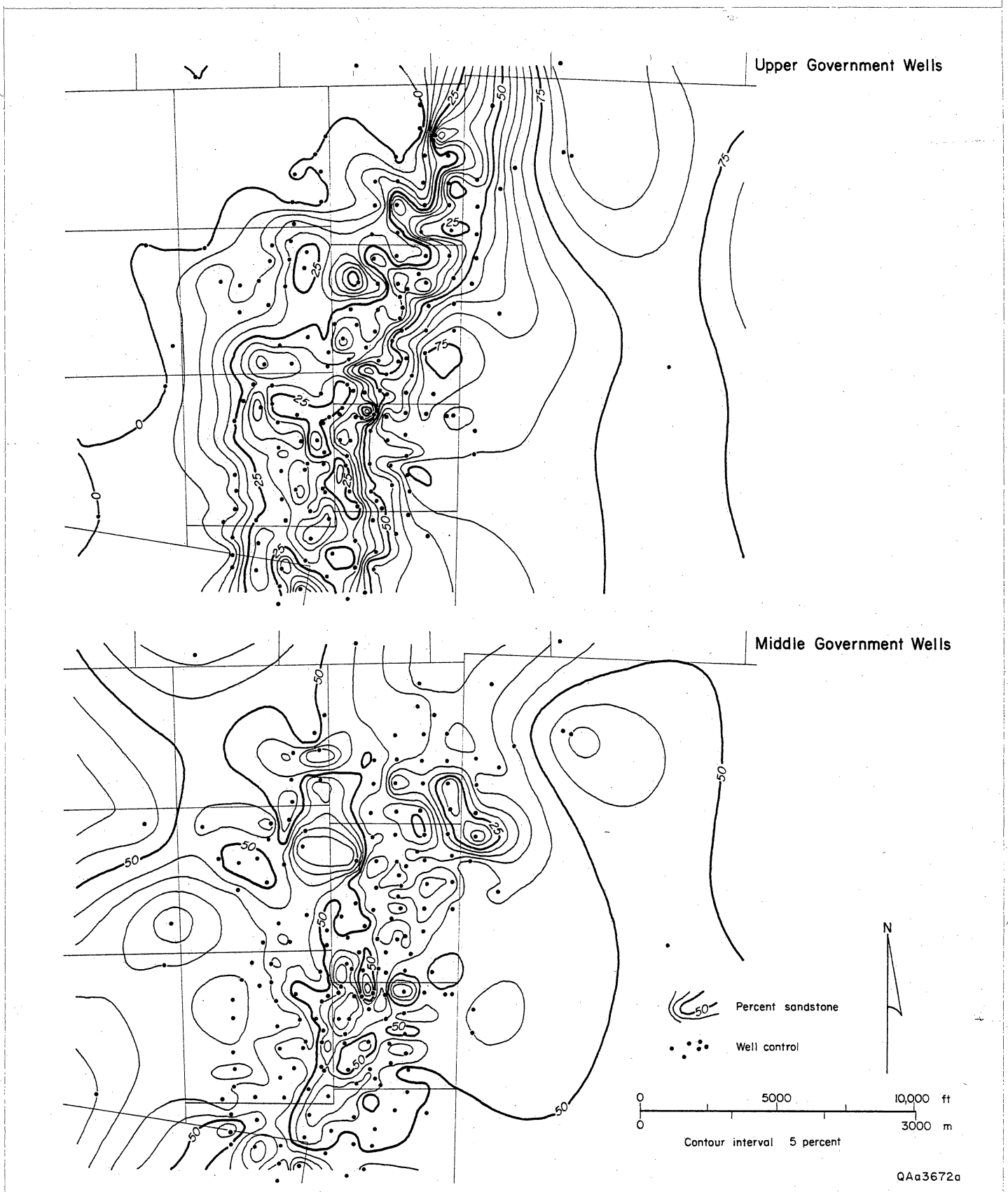
Figure 13. Percentage-sandstone maps for Upper Government Wells, Middle Government Wells, Upper Loma Novia, and Middle Loma Novia reservoir sandstones, Prado field. Maximum percentage sandstone for all intervals trends north-northeast. The area of greater than 75 percent sandstone prograded downdip from the Middle Loma Novia to the Upper Government Wells.
