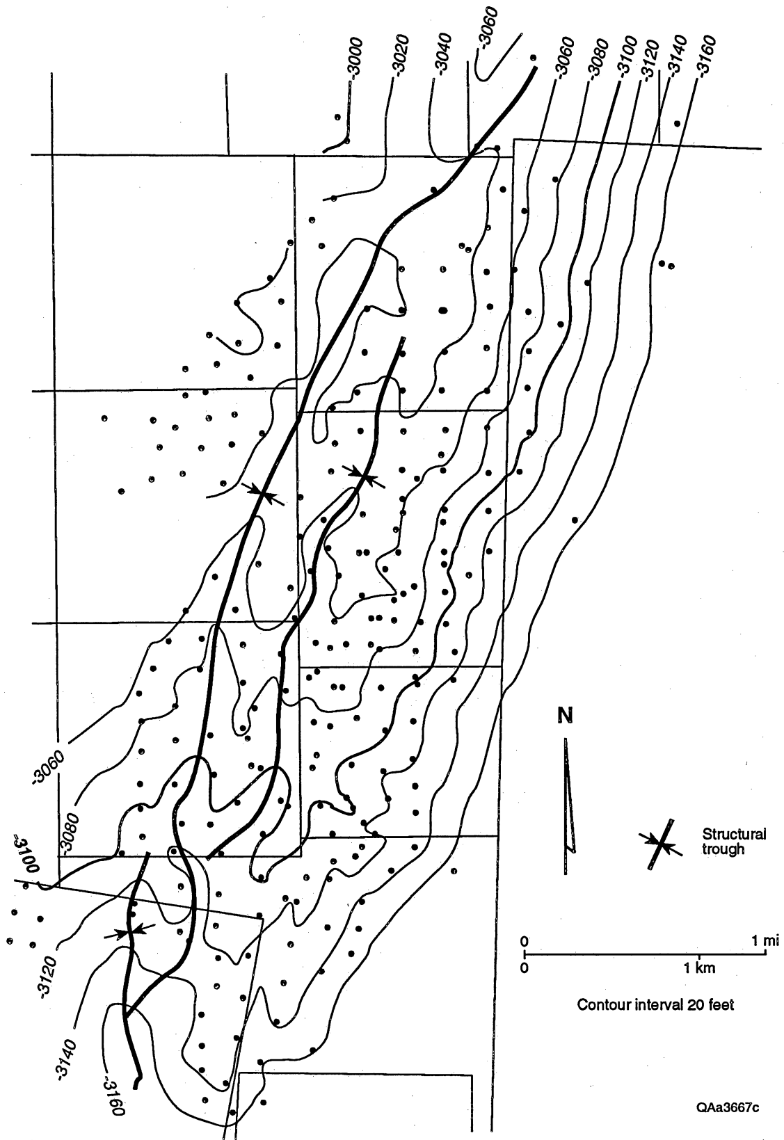
Figure 8. Structure-contour map of top Middle Loma Novia II sandstone. A structural trough on the updip margin of the field is another example of drape compaction over zone between mud-rich lagoonal facies updip and sand-rich barrier facies downdip. Modified from Railroad Commission of Texas docket no. 4-55,323.
