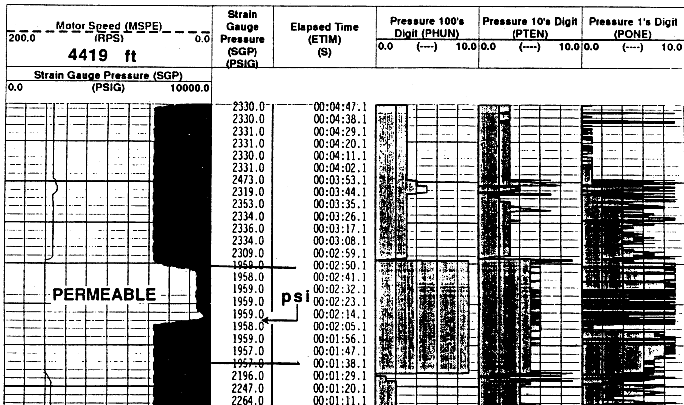
Figure 41. Response of well log pressure tester for permeable and tight intervals.
