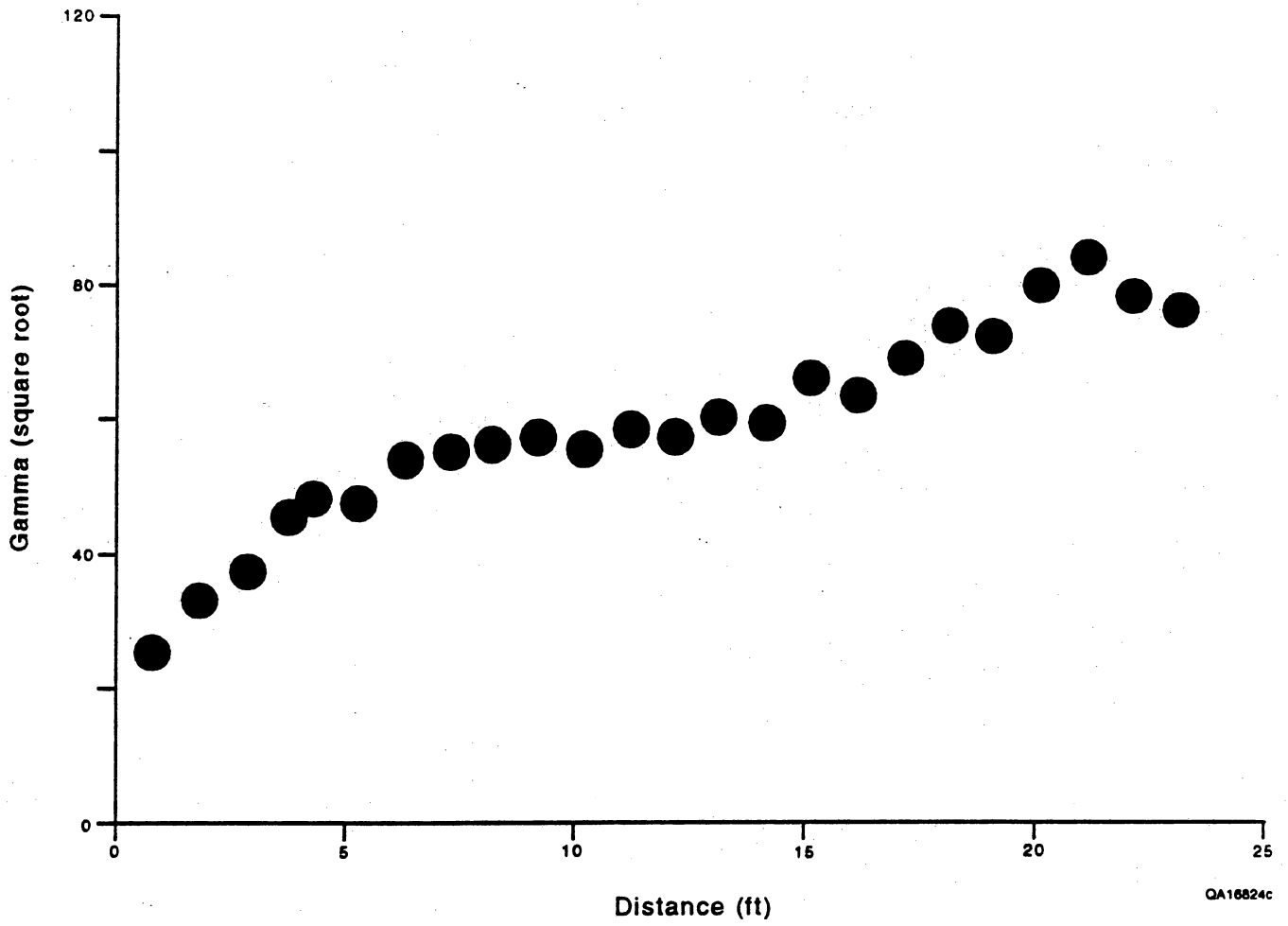
Figure 31. Vertical variogram within distributary-channel facies from South Muddy Creek.
