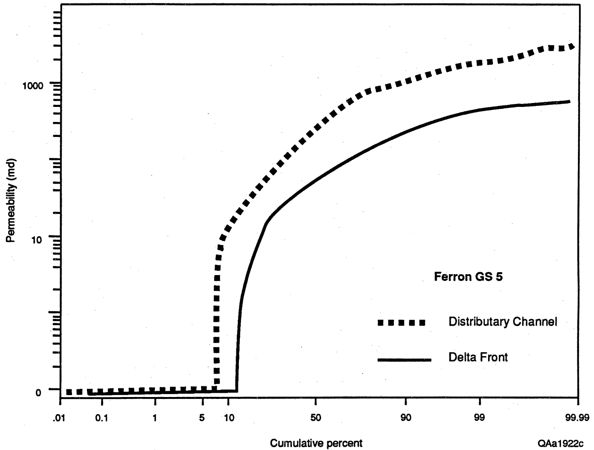
Figure 10. Cumulative percent plot of permeability comparing distributary-channel and delta-front deposits. Data from a log normally distributed population would plot as a straight line in these coordinates.
