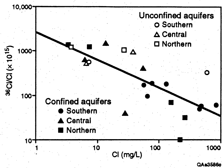
Figure 7. Variation of ^{36}\text{Cl}/\text{Cl} ratio with chloride ionic concentration in ground waters beneath the High Plains.
