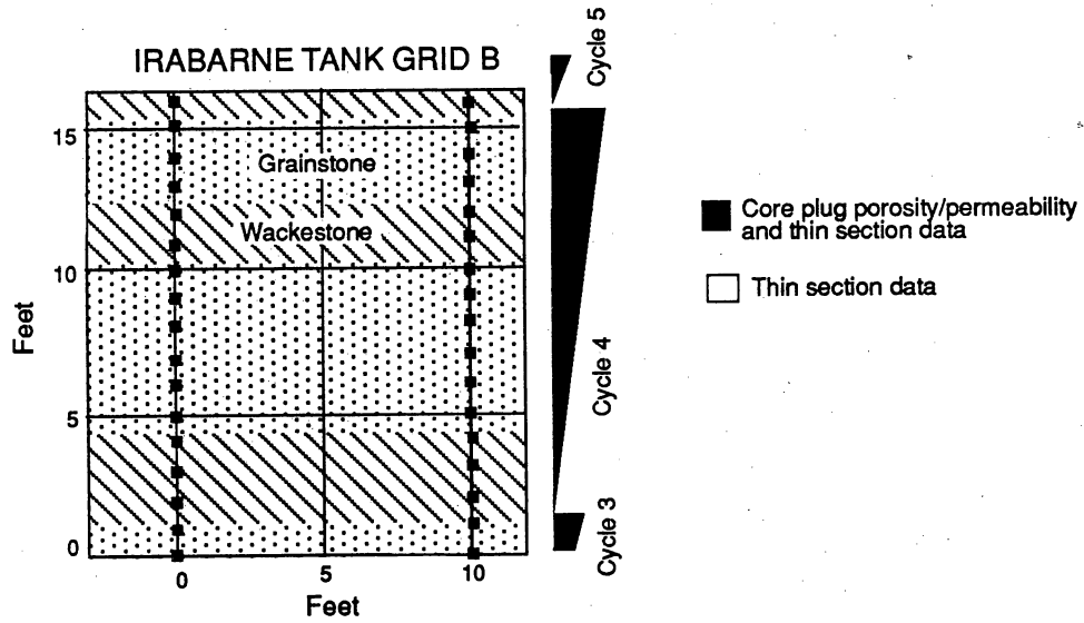
Figure 53. Sampling grids for core plugs at Irabarne Tank Canyon (see fig. 52). Lithology is based on outcrop descriptions. Lithology in figure 54 is based on thin-section descriptions.
