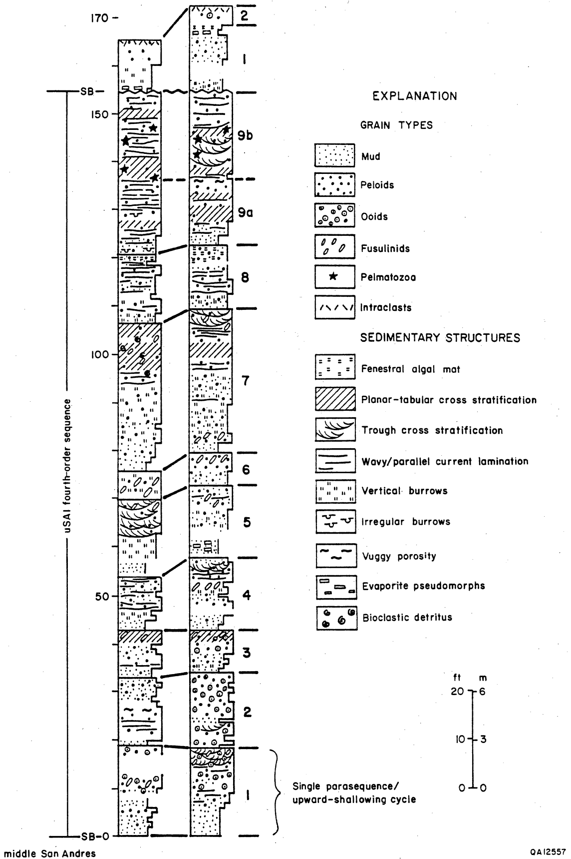
Figure 14. Detailed vertical sections showing the depositional cyclicity of the ramp-crest parasequences, Lawyer Canyon uSA1 ramp-crest parasequence window.
