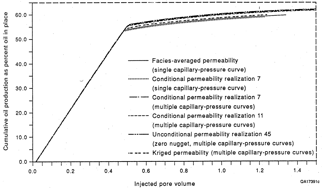
Figure 40. Cumulative oil production as percentage of original oil in place for waterflood simulations in parasequence 1 (ps1).
