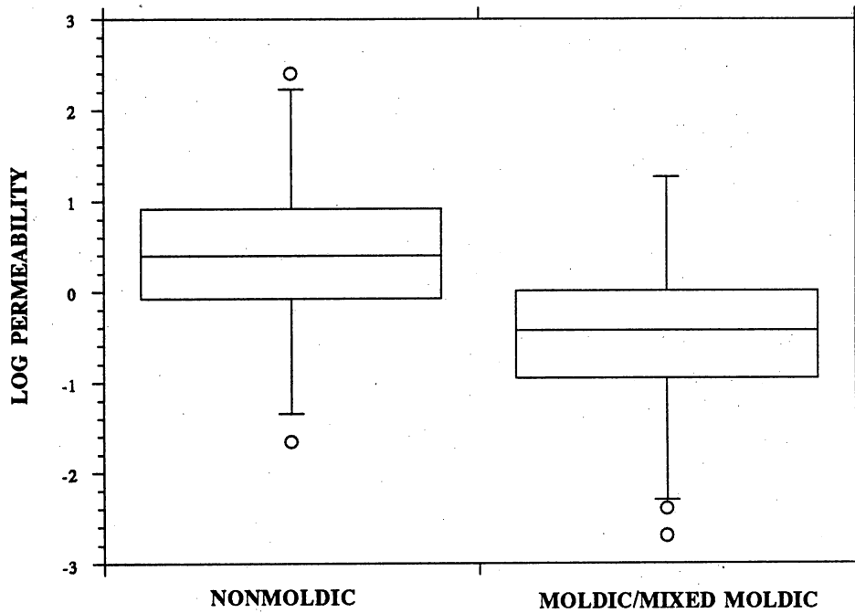
Figure 64. Comparison of geometric means of permeability between nonmoldic and moldic facies from cycles 10 and 11, Seminole San Andres Units.
