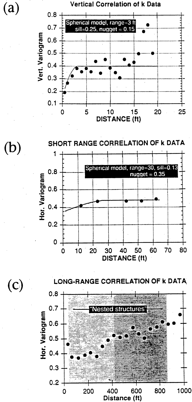
Figure 29. Sample variograms for the permeability transects from the grainstone facies in parasequence 1 (ps1): (a) vertical variogram based on all transects, (b) short-range horizontal variogram, based on the 5-ft grid between sections A and Z, and (c) long-range horizontal variogram, based on all transects spaced 25 and 100 ft.
