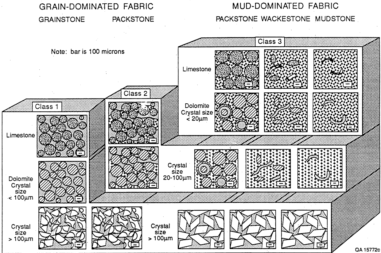
Figure 7. Petrophysical rock-fabric classes.
