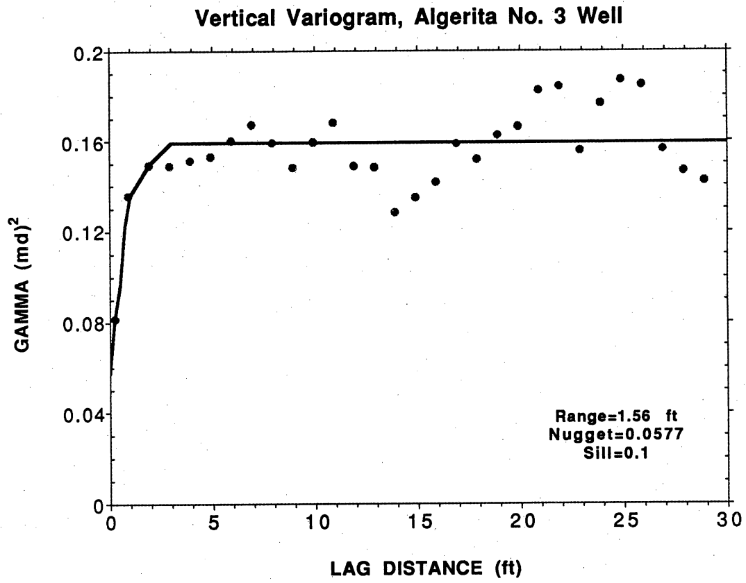
Figure S9. Vertical variogram model for the interval from 460 to 520 ft in the core from Algerita No. 3 well.
