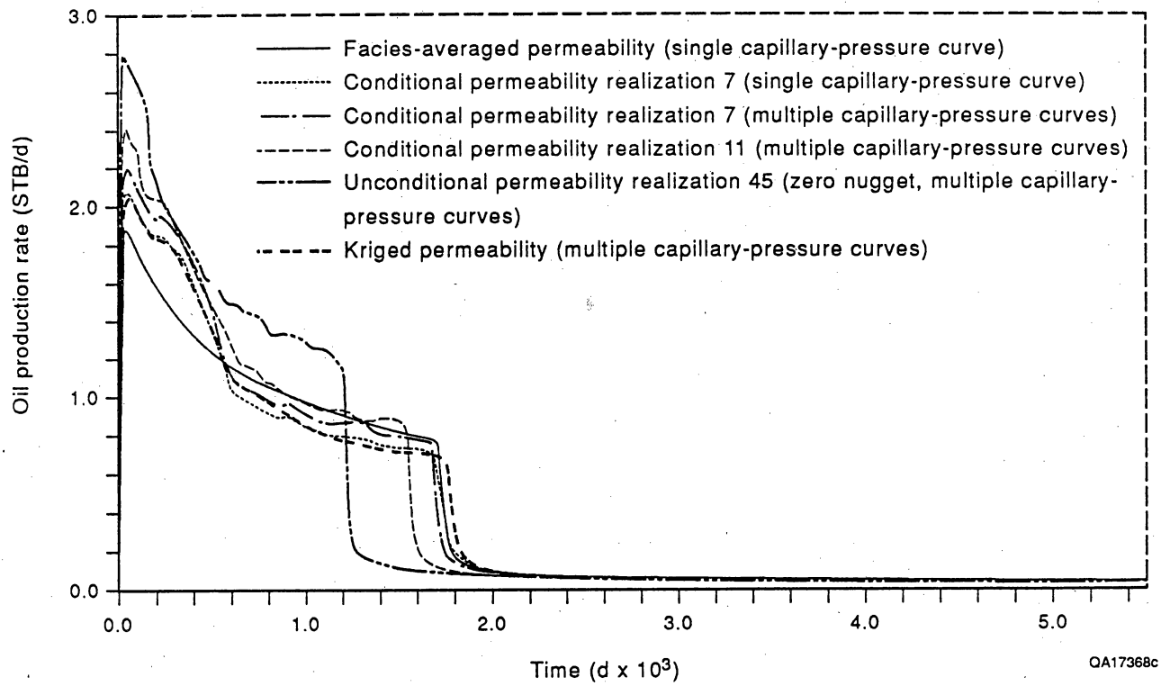
Figure 38. Oil-production rate versus time for waterflood simulations in parasequence 1 (ps1).
