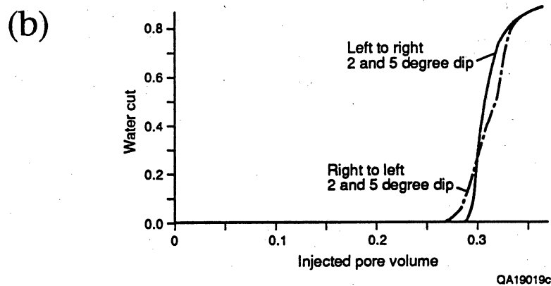
Figure 66. Results of computer simulation of Irabarne Tank Canyon flow model. (a) Oil-production rate versus rate assuming 2^\circ and 5^\circ dip (curves overlie each other) and injecting from right and from left side of model. (b) Water cut versus injected pore volume assuming 2^\circ and 5^\circ dip (curves overlie each other) and injecting from right and from left side of model.
