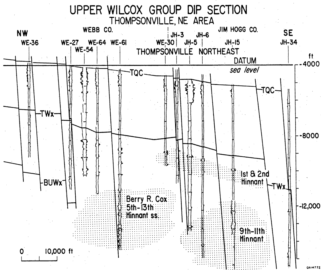
FIGURE 11. Structural dip-oriented cross section in Thompsonville, NE field, Webb and Jim Hogg Counties, Texas. Thick productive sandstones include first and fifth through thirteenth Hinnant sandstones in Berry R. Cox and Thompsonville, NE fields. Major gas reservoir at Thompsonville, NE field is first Hinnant.
