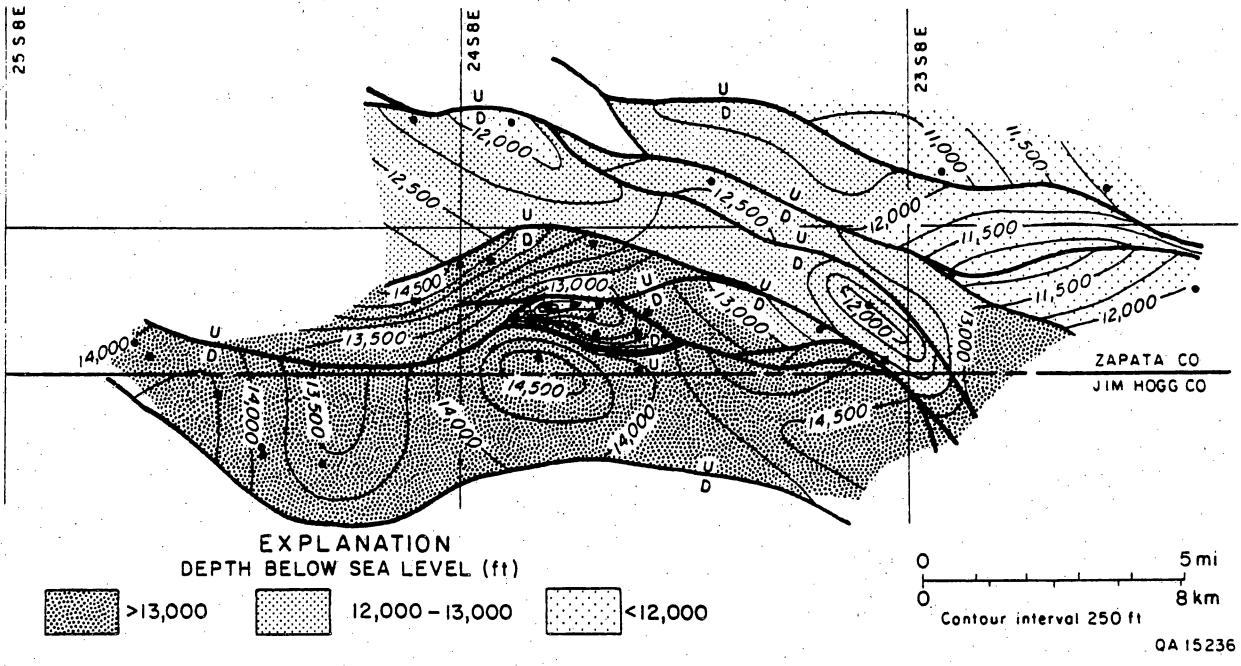
FIGURE 12. Structure map of tenth Hinnant, or R sandstone, in Fandango field, Zapata and Jim Hogg Counties, Texas.
