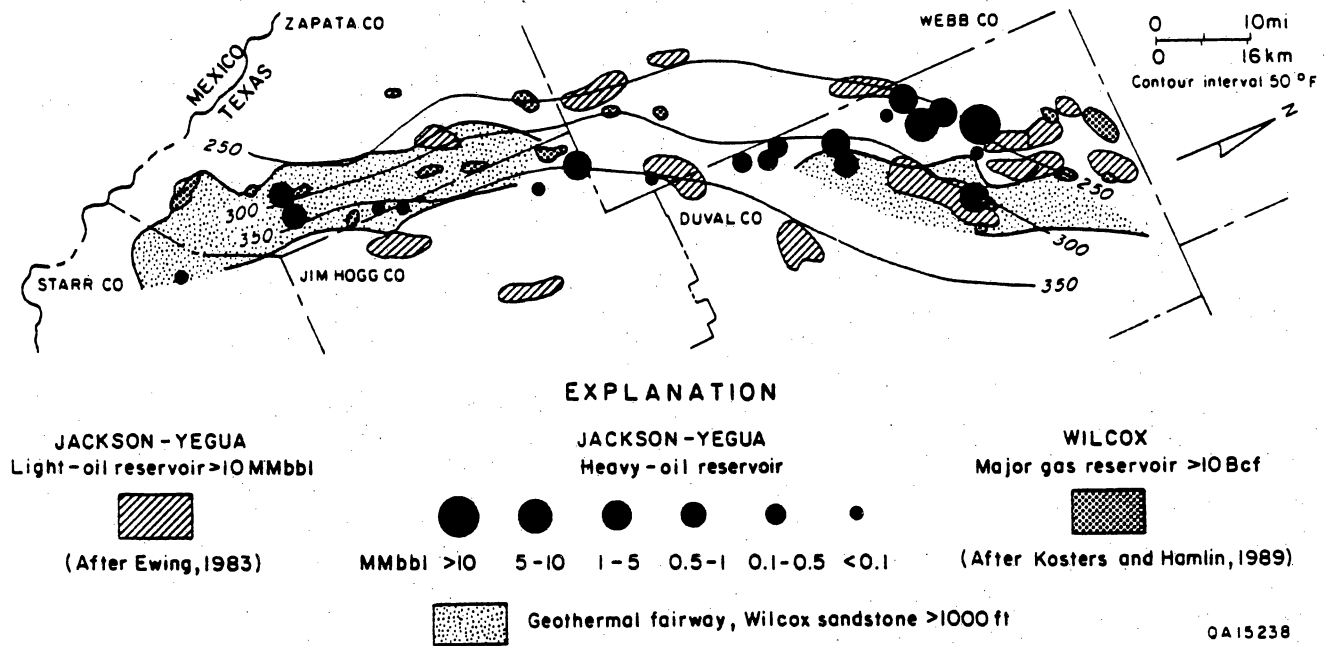
FIGURE 1. Colocation of geopressed geothermal fairways and Jackson Group heavy-oil reservoirs. Patterned area of geothermal fairway includes regions where calculated temperature of middle part of upper Wilcox exceeds 250°F (121°C) and where thickness of net sandstone in the upper Wilcox exceeds 1,000 ft (300 m). Size of circles is relative to the cumulative oil production of heavy-oil reservoirs through 1988.
