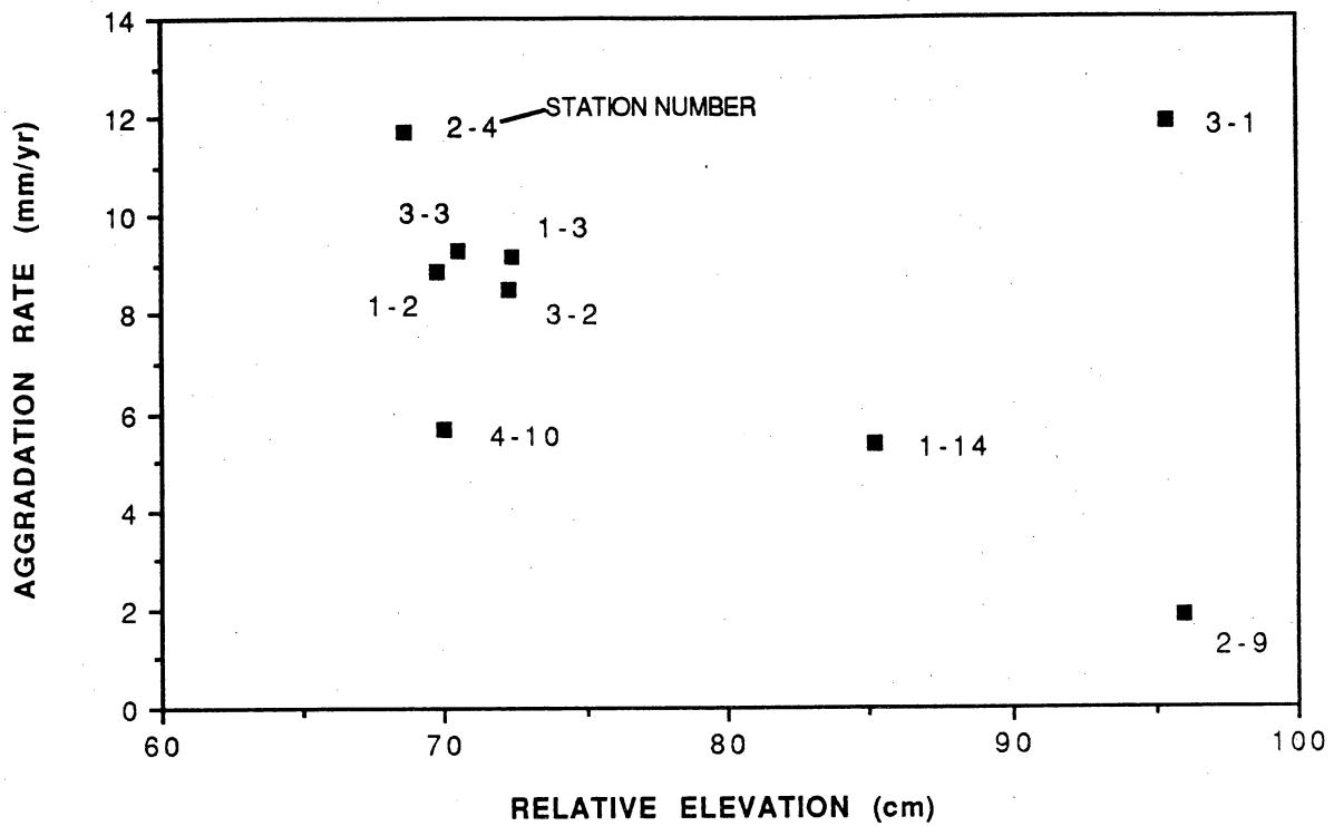
Figure 10. Comparison of sedimentation rates at stations in the Colorado River Delta with relative elevations of marshes at those stations. In general, marshes at lower elevations had higher sedimentation rates than those at higher elevations. This indicates that there is an inverse relationship between elevation and sedimentation, at least during storm-free periods. Storms and flood events can deposit sediments at the higher elevations, nullifying this relationship.
