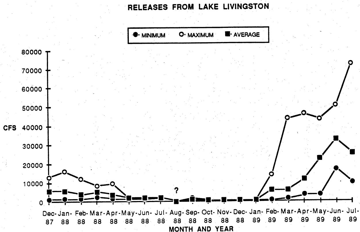
Figure 11. Water releases from Lake Livingston in \text{ft}^3/\text{sec} (CFS) from December 1987 through July 1989. It has been estimated that all of the Trinity River delta is completely flooded at river discharges exceeding 30,000 \text{ ft}^3/\text{sec} during high tide. Near record flooding occurred during July 1989. (Data from Trinity River Authority.)
