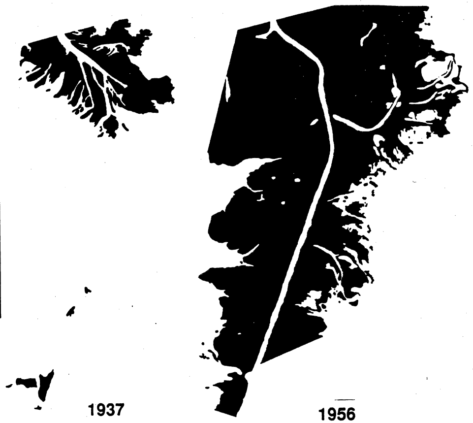
Colorado River delta index map and historical sequence of vegetated areas (in black) for the years 1937, 1956, 1974, and 1982.
