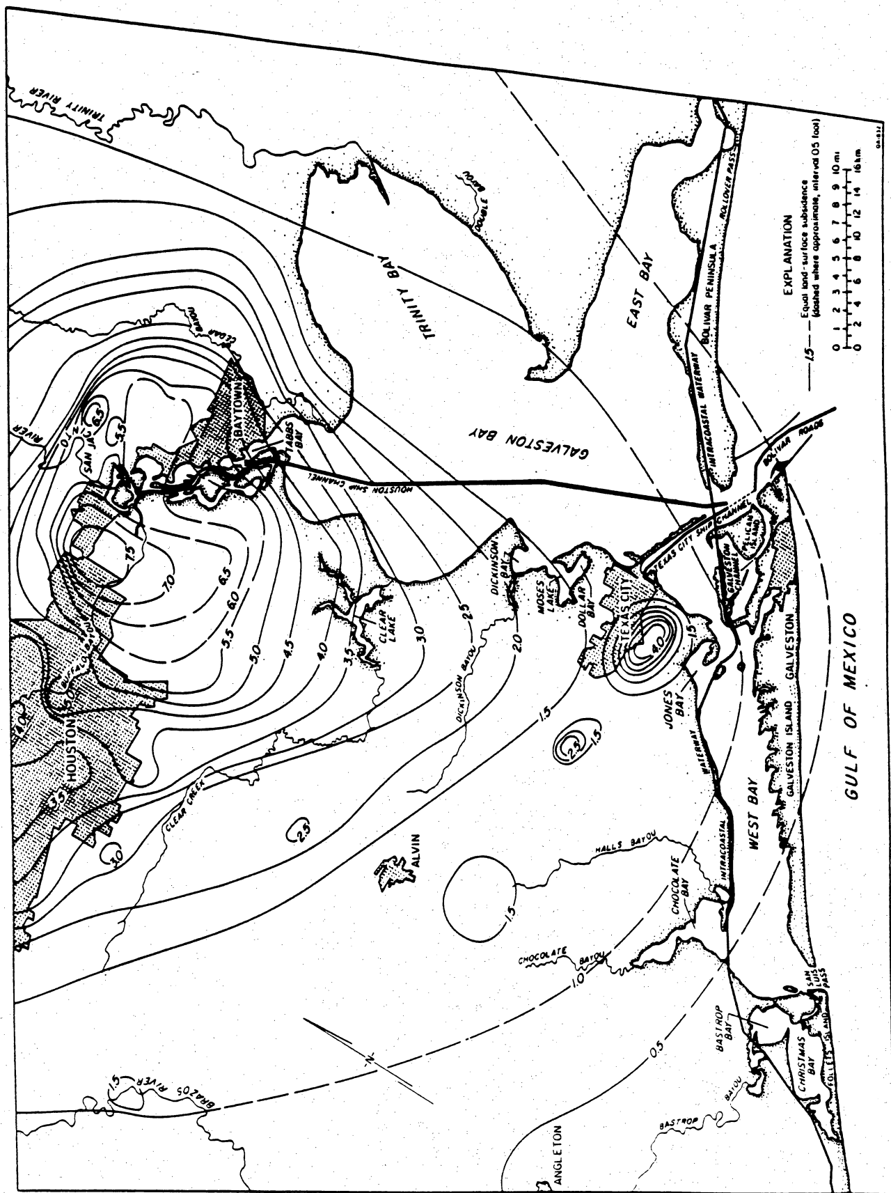
Figure 3. Land-surface subsidence in the Houston-Galveston area, 1943-1973. (From Gabrysch and Bonnel, 1975.)
