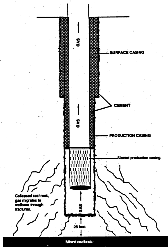
Figure 88. Schematic of a gob well.
