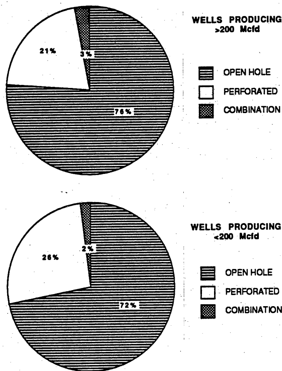
Figure 96. Comparison of completion methods used in wells producing more and less than 200 Mcfd.
