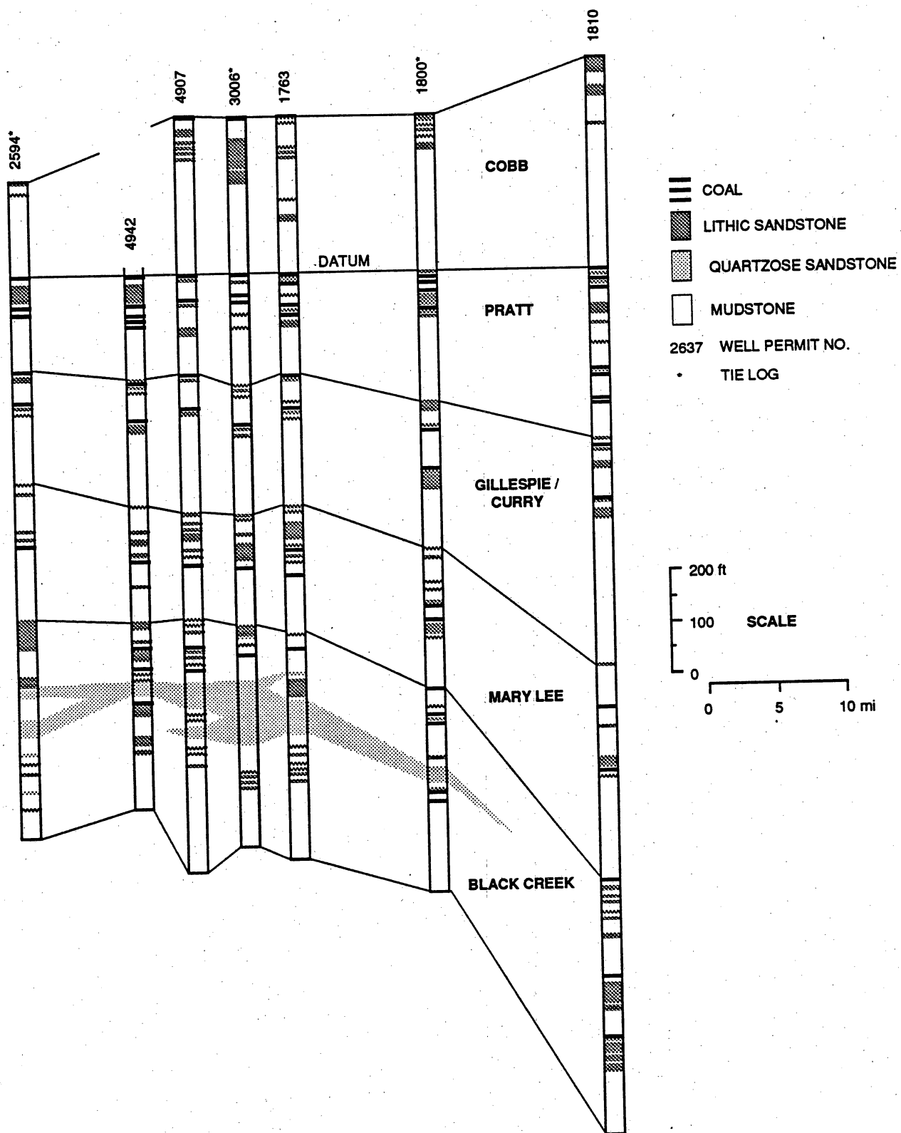
Figure 42. Stratigraphic cross section C-D. See figure 4 for location of cross section.
