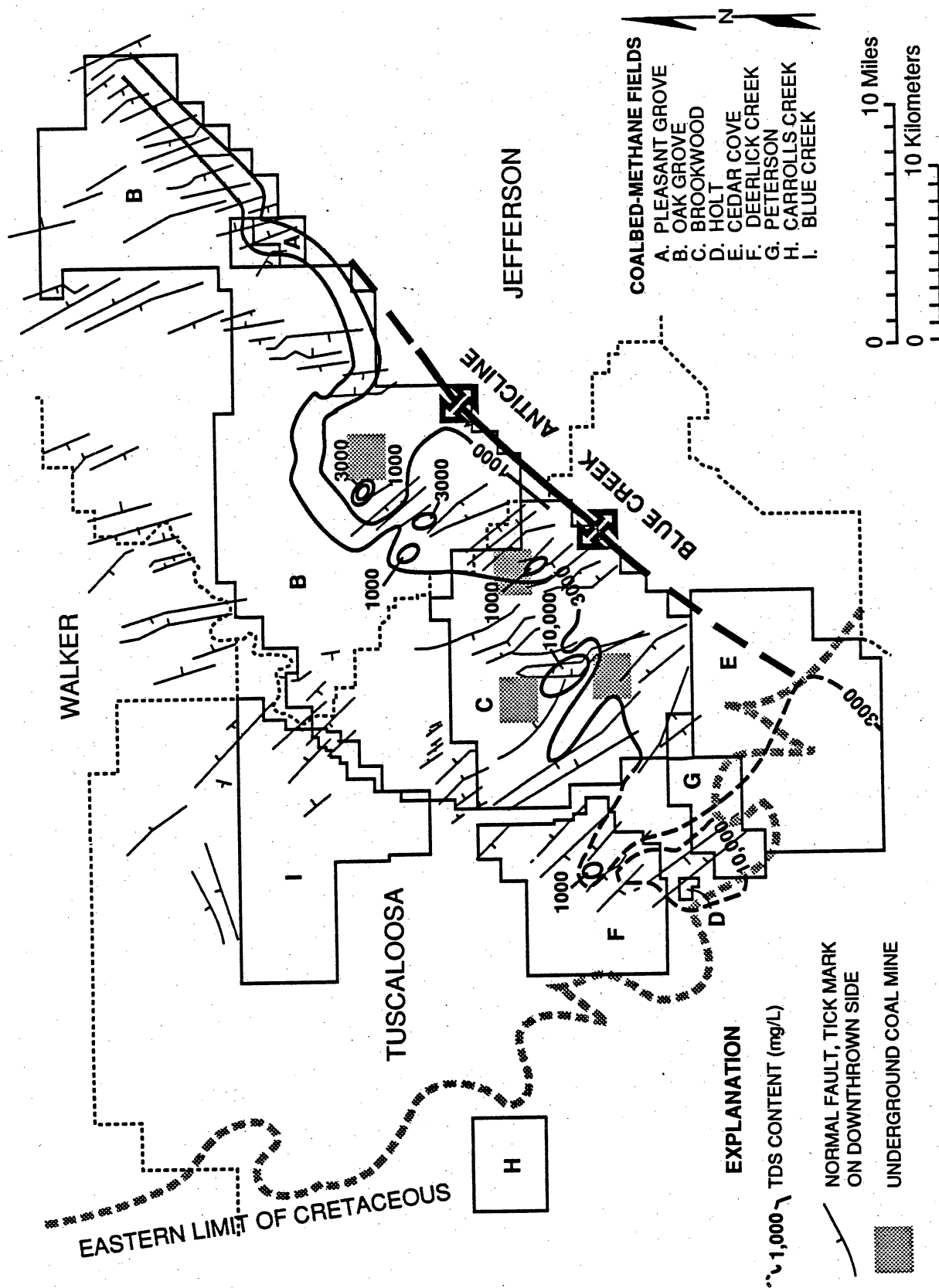
Figure 85. Relationships among water salinity, structural features, and underground mines.
