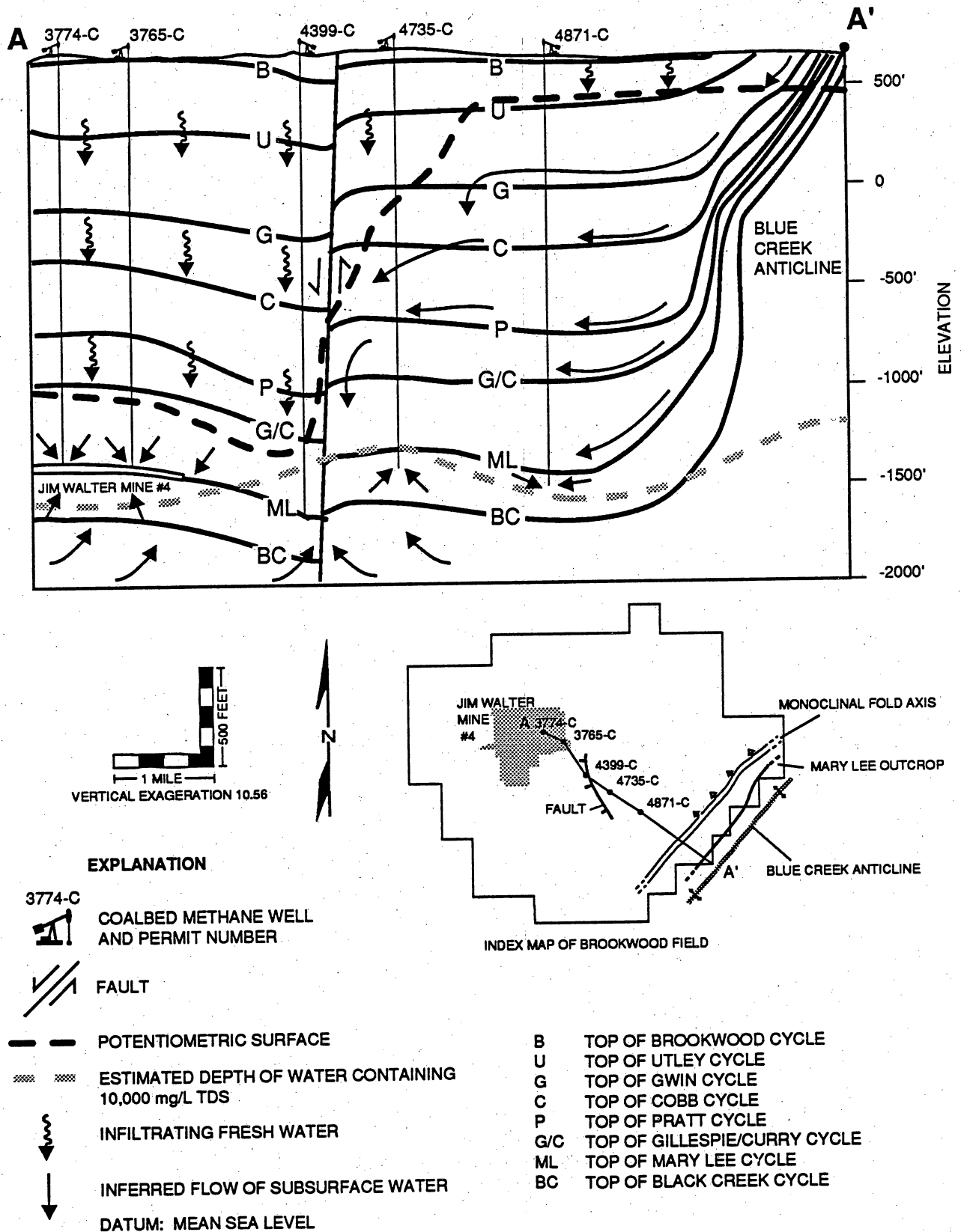
Figure 68. Idealized hydrogeologic cross section for an Alabama coalbed-methane field.
