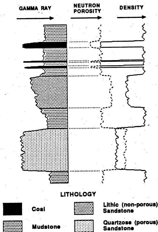
Figure 38. Sample geophysical log depicting the relationship between log signature and lithology.
