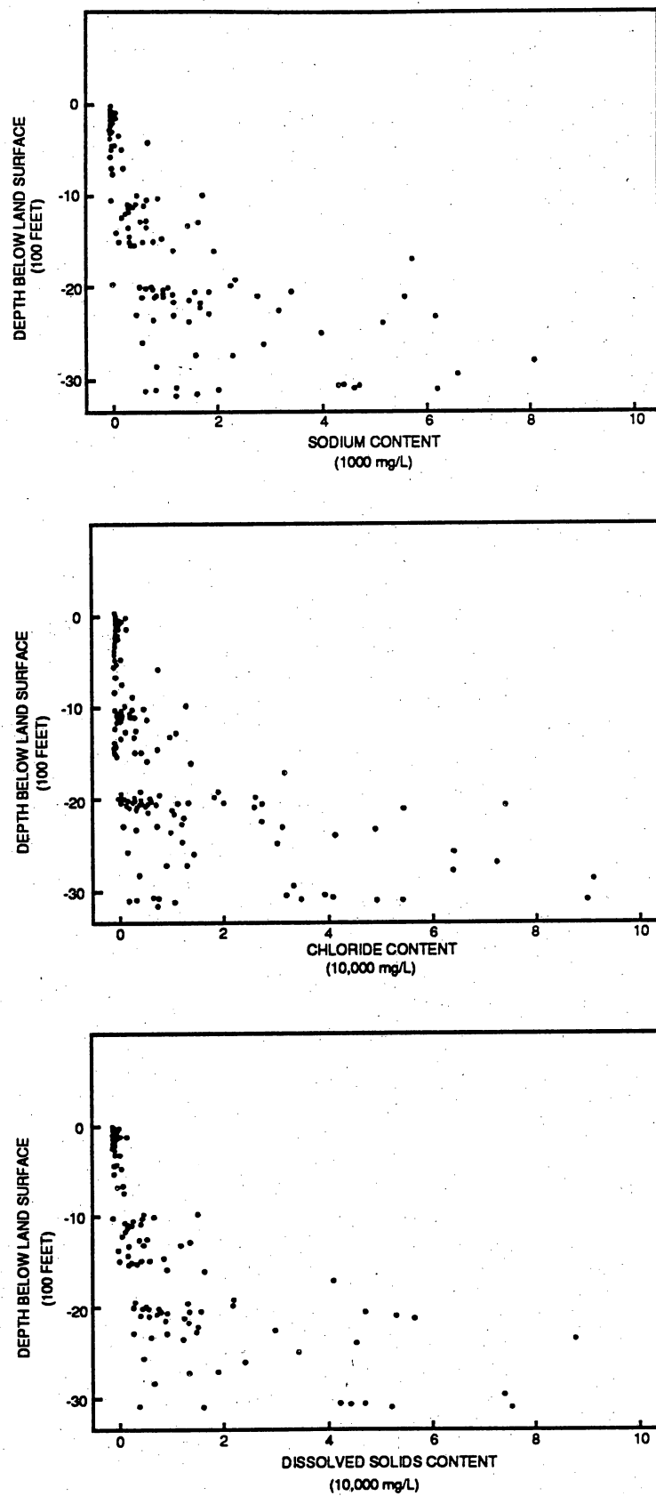
Figure 77. Selected scattergrams showing relationship between salinity and depth.
