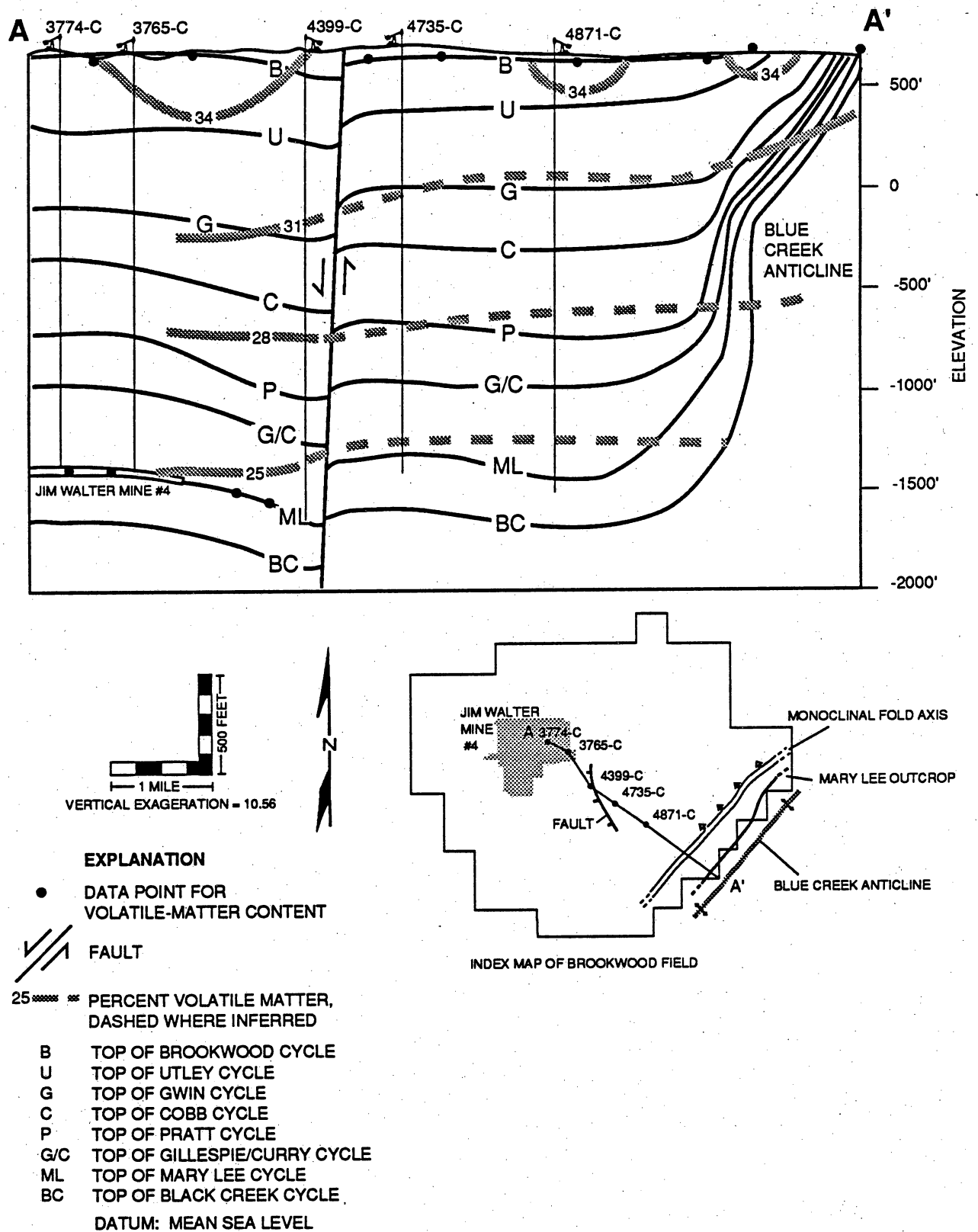
Figure 7. Structural cross section of upper Pottsville strata in Brookwood field showing approximately horizontal isovols. Monoclinical fold axis from Epsman and others (1988). See figure 1 for location of Brookwood field.
