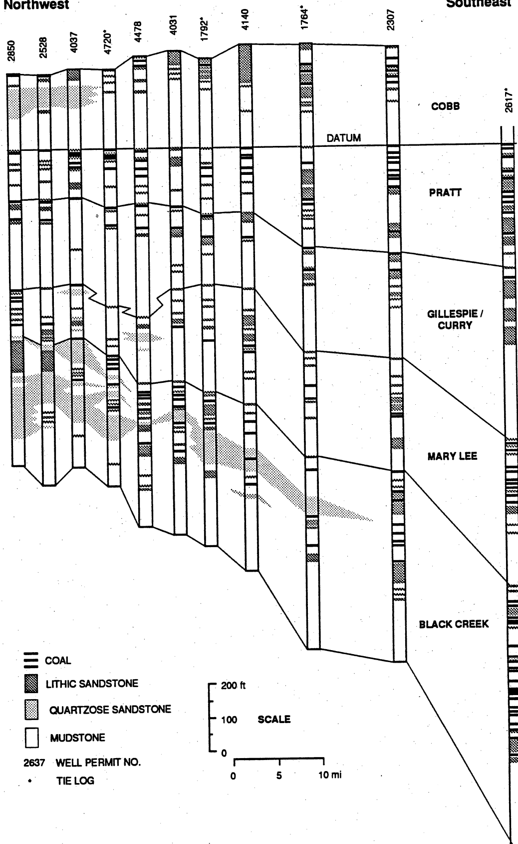
Figure 43. Stratigraphic cross section E-E'. See figure 4 for location of cross section.
