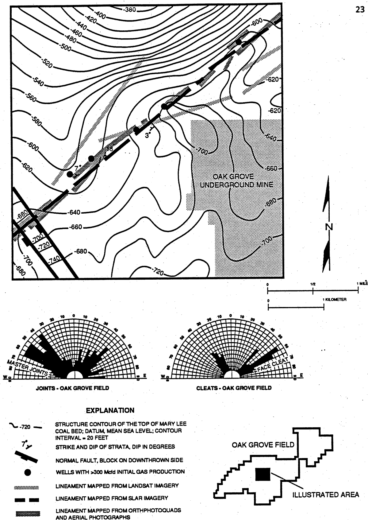
Figure 12. Structural configuration of the top of the Mary Lee coal bed and surface-fracture orientation in a selected part of Oak Grove field, Jefferson County, Alabama (structure contours from Epsman and others, 1988). See figure 11 for location of Oak Grove field.
