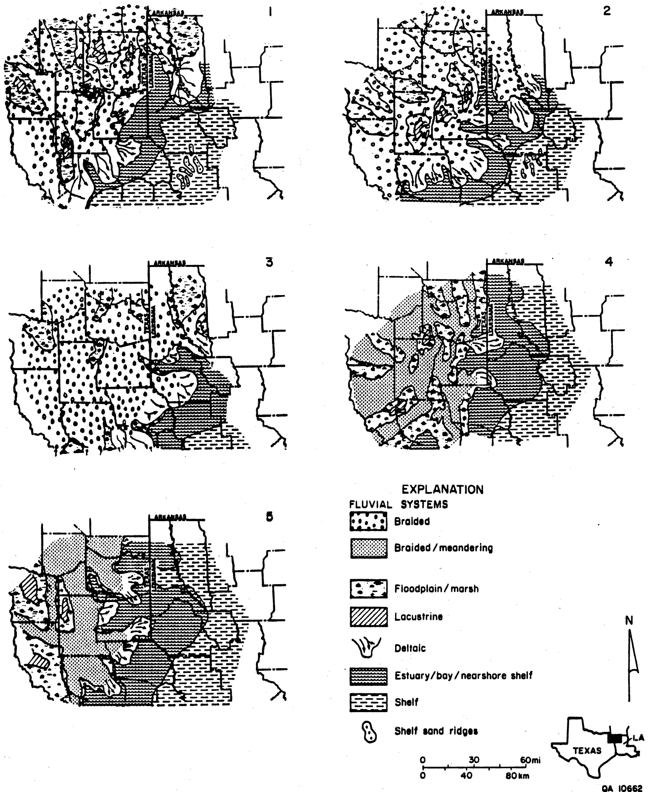
Figure 15. Hypothetical paleogeographic reconstructions of five time periods during Travis Peak deposition. Note initial development and progradation of fluvial-deltaic systems, followed by shoreline transgression. Interpretations are based on sedimentary patterns observed in isopach, net-sandstone, and percent-sandstone maps of lithostratigraphic units 1 through 5 (Tye, 1989) and core from wells shown in figure 5. Actual timespan represented by each period is variable and unknown.
