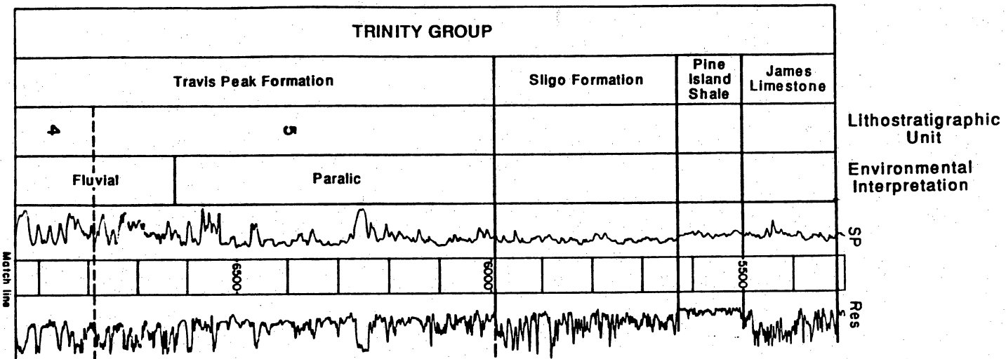
Figure 6. Type log of Travis Peak Formation from eastern Panola County, Texas. Lithostratigraphic unit divisions and environmental interpretations are illustrated. Location shown in figure 5.
