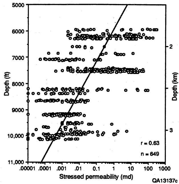
Figure 37. Plot of stressed permeability versus depth for 649 Travis Peak sandstones.
