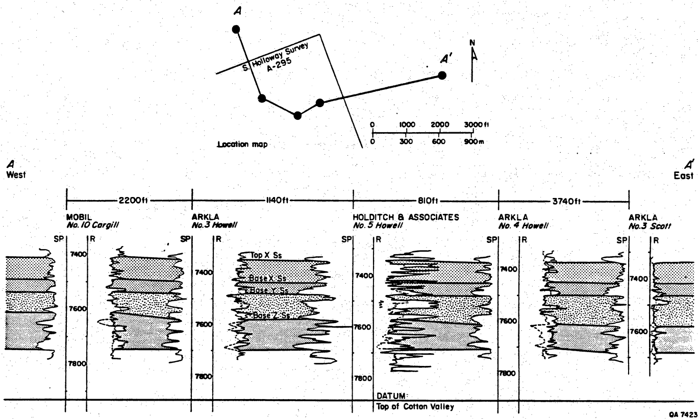
Figure 18. Cross section of lower Travis Peak producing sandstones in area around the SFE No. 1 well.
