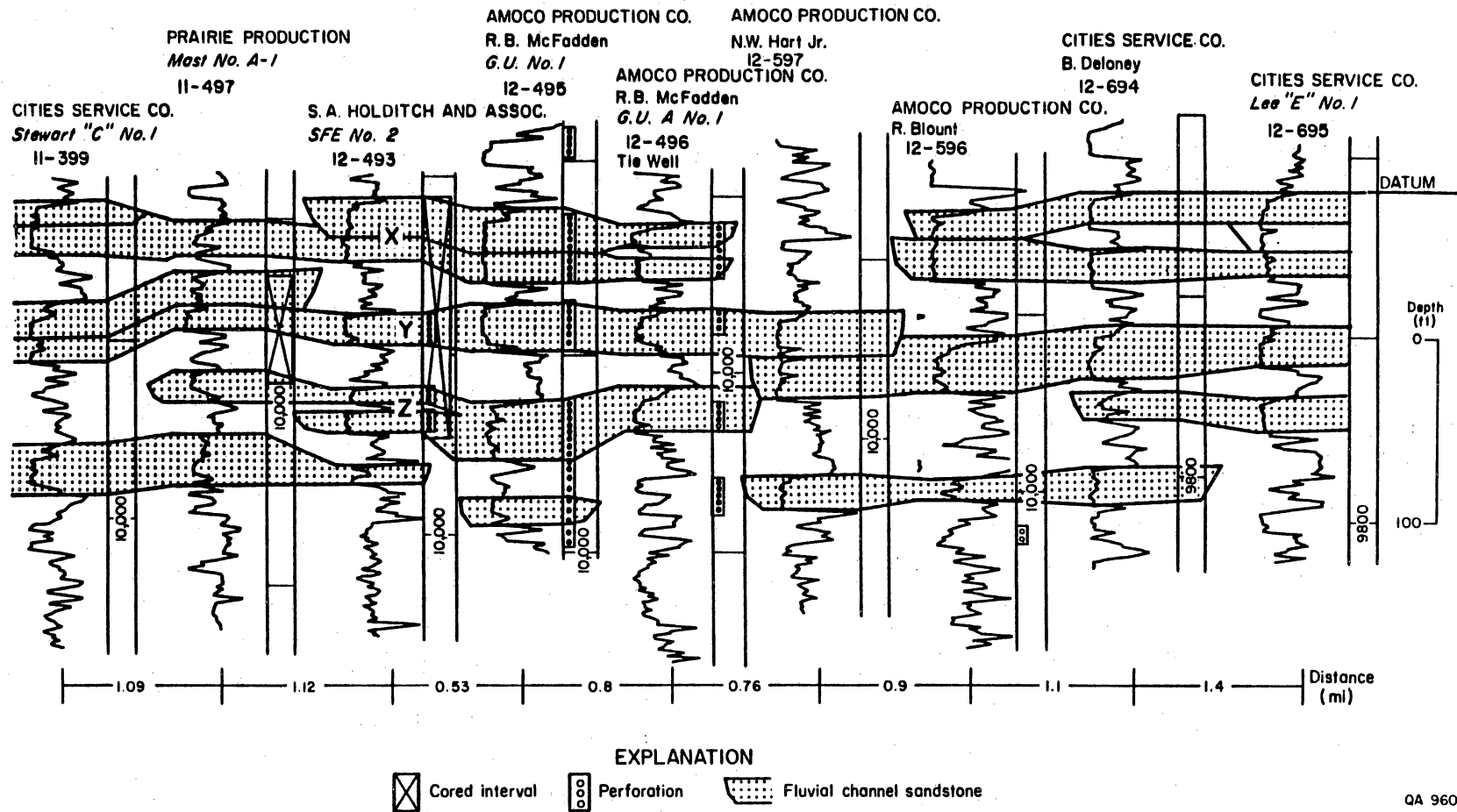
Figure 24. Stratigraphic cross section D-D' illustrating the occurrence and geometry of channelbelt sandstones in lower Travis Peak Zone 4, North Appleby field. Note the relative increase in multilateral fluvial channel sandstones in Zone 4 as compared to Zone 1 (fig. 23). Erosional juxtaposition of discrete sandstone lenses is greater in Zone 4 than in Zone 1, thus indicating a higher degree of channel scour and lateral migration. Gamma-ray log curves are shown. Line of section shown in figure 21.
