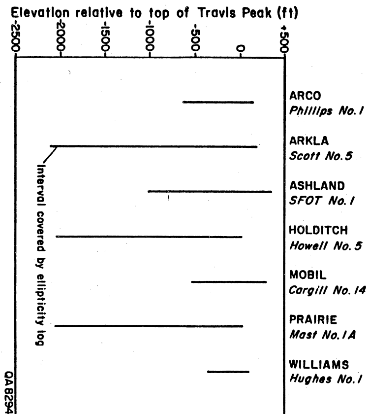
Figure 59. Plot of wells showing intervals in Travis Peak Formation covered by ellipticity logs in this study.
