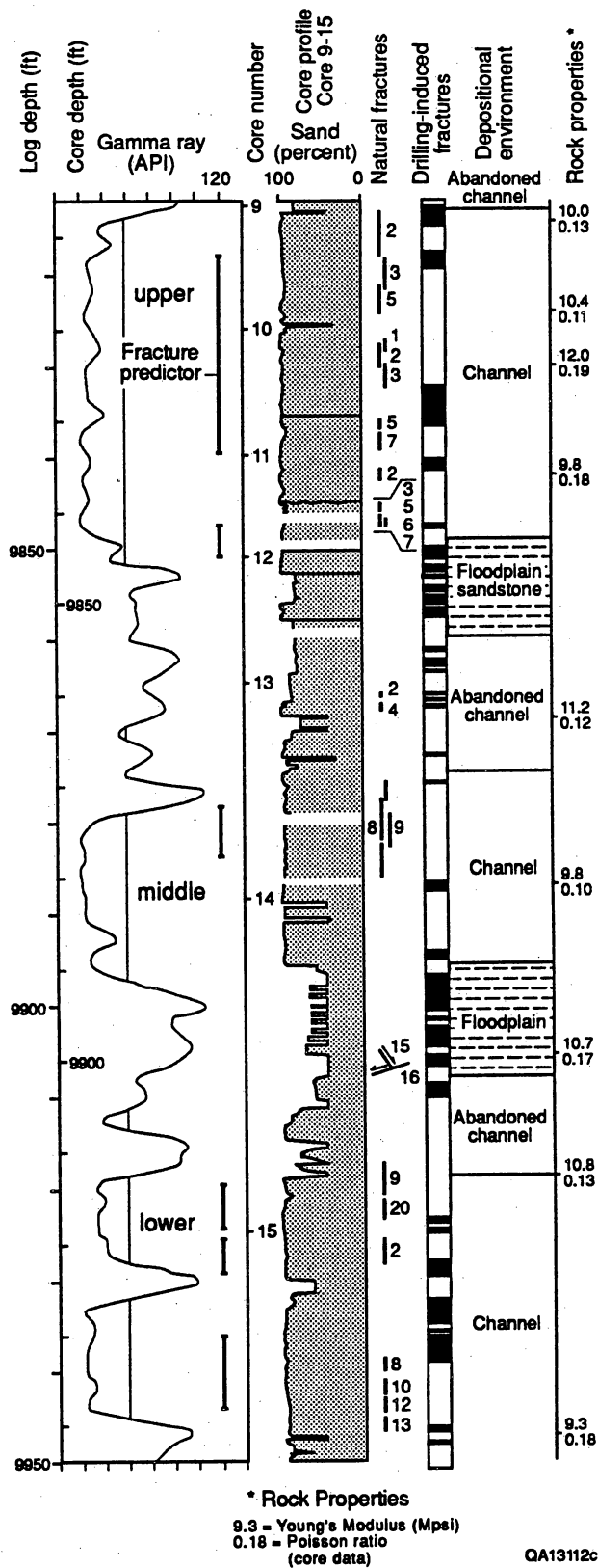
Figure 46. Core gamma-ray log, core profile, fracture distribution, and environmental interpretation, core 9-15, SFE No. 2 well. Static rock property measurements from core plugs in this interval are also indicated. This core interval illustrates numerous fractures in lower Travis Peak Formation. Intervals labeled "Fracture predictor" indicate where zones of favorable rock types for natural fracture development were predicted from geophysical log data (Ercill Hunt, personal communication, 1988).
