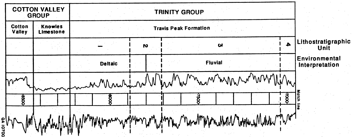
Figure 6. Type log of Travis Peak Formation from eastern Panola County, Texas. Lithostratigraphic unit divisions and environmental interpretations are illustrated. Location shown in figure 5.
