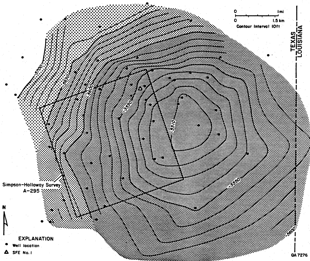
Figure 16. Structure map of top of lowest carbonate bench in Sligo Formation, Waskom field, Harrison County, Texas. Location of SFE No. 1 (Holditch & Associates Howell No. 5) is shown.
