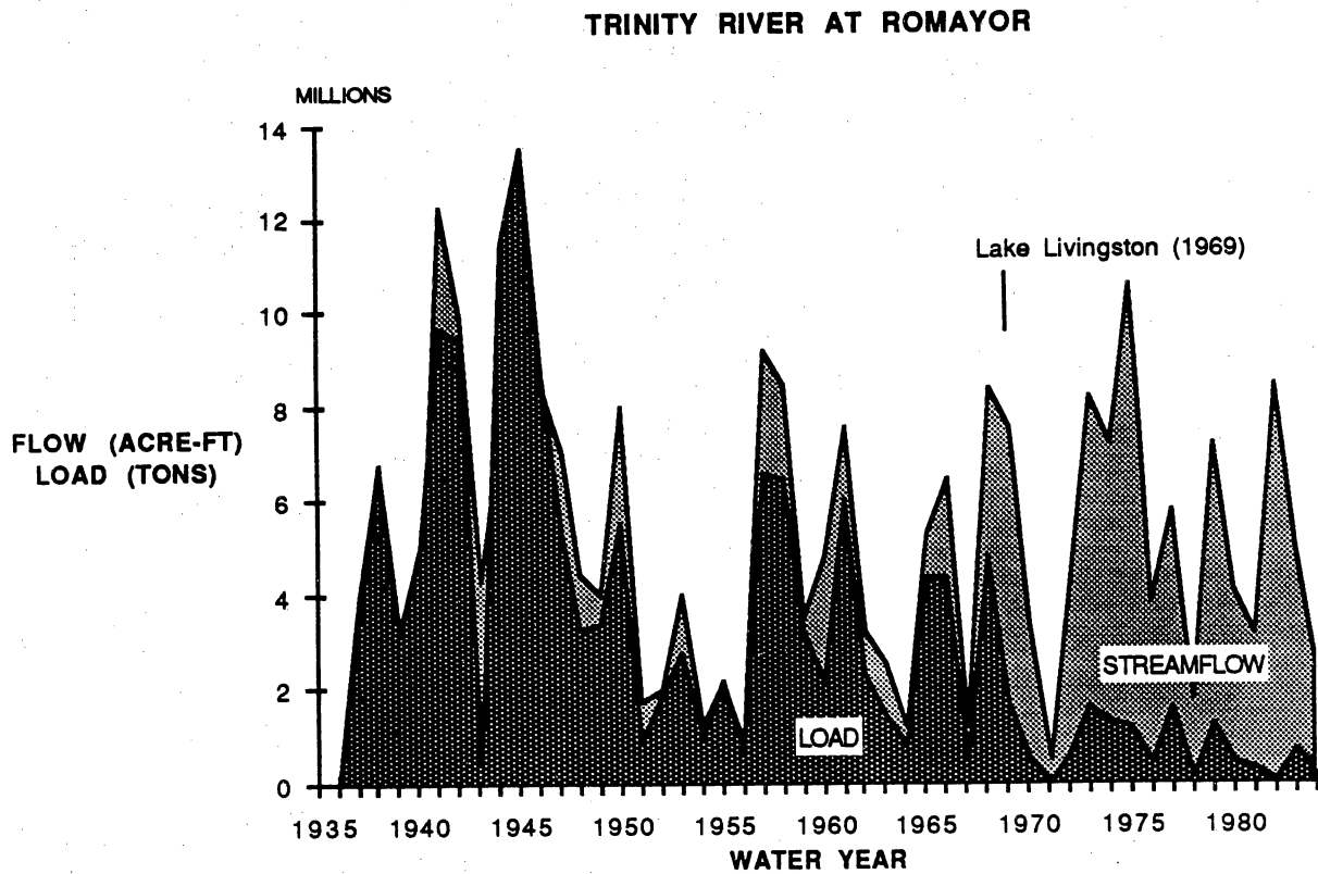
Figure 4. Annual streamflow and suspended sediment load of the Trinity River. (Compiled from Texas Water Development Board reports.)
