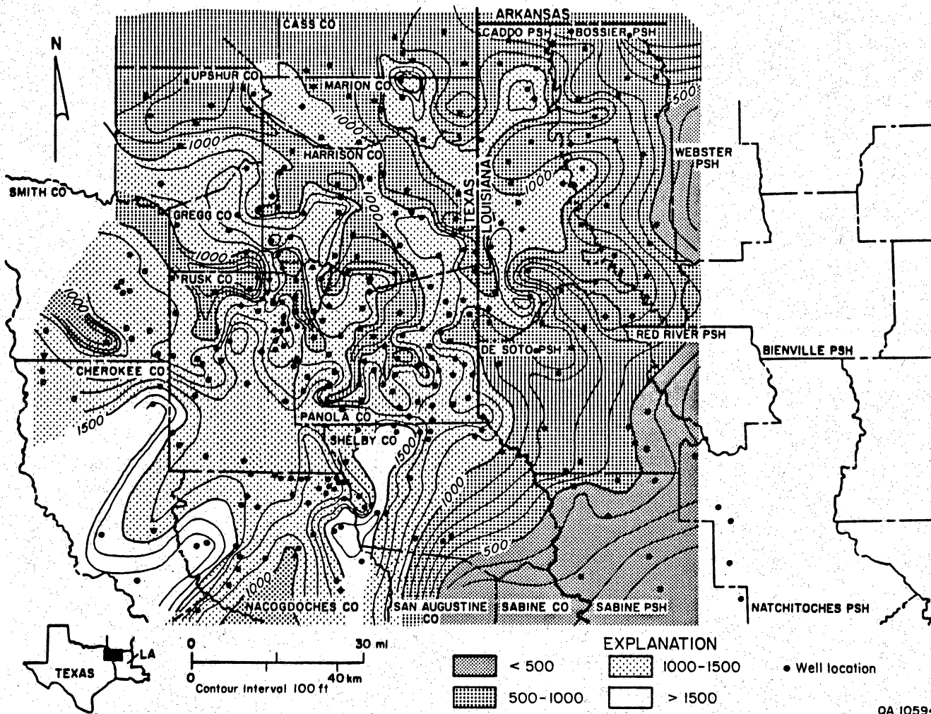
Figure 9: Regional net-sandstone map of the Travis Peak Formation in the East Texas-West Louisiana study area.
