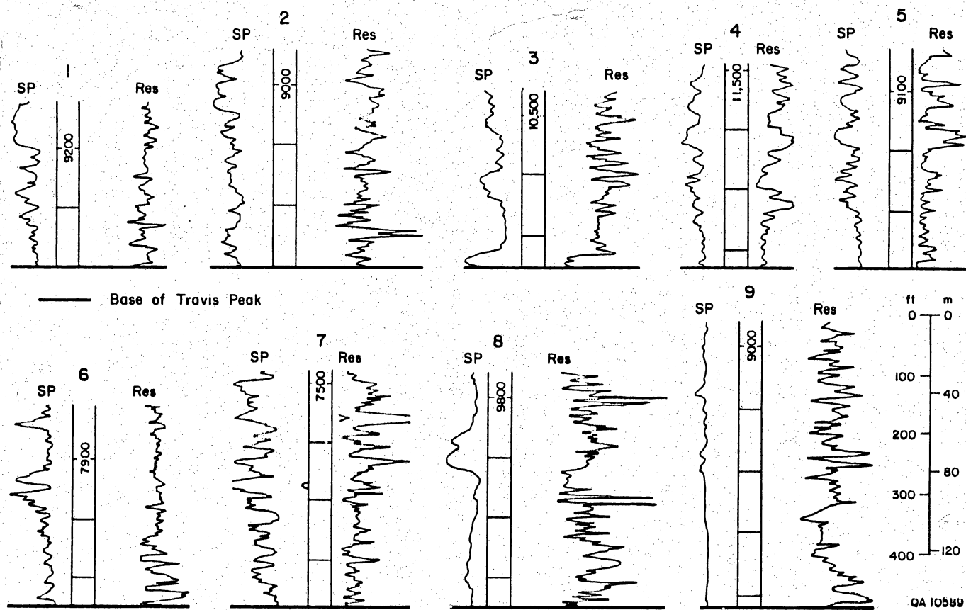
Figure 29: Representative spontaneous potential (SP) and resistivity (Res) curves for lithostratigraphic unit 1. Location of wells is given in figure 4.
