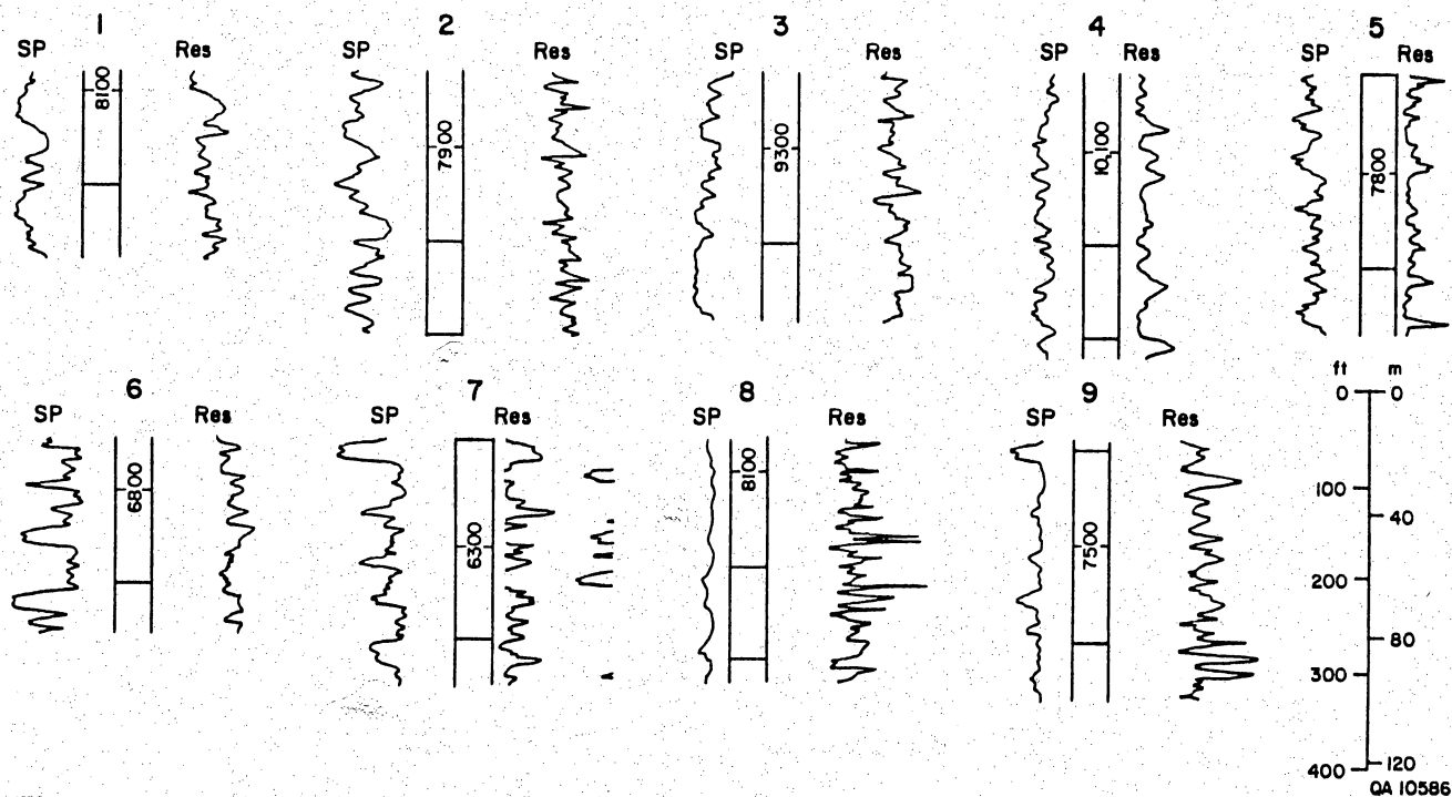
Figure 32: Representative SP and resistivity curves for lithostratigraphic unit 4. Location of wells is given in figure 4.
