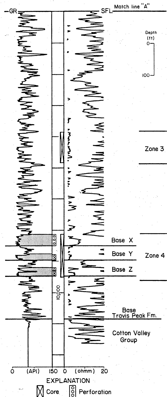
Figure 37: Gamma-ray and resistivity (SFL) logs for the Travis Peak Formation in the SFE No. 2 well. Zones 1 through 4 refer to cored stratigraphic intervals that were studied in detail. Three sandstones separated by mudstones are present in Zone 1, and these sediments are interpreted as poorly developed braided-channel sandstones, levee, splay, and lacustrine sandstones, and floodplain (swamp) mudstones. The three sandstones separated by mudstones in Zone 4 are interpreted as well-developed braided-channel sandstones, levee, splay, and lacustrine sandstones, and floodplain (swamp) mudstones.
