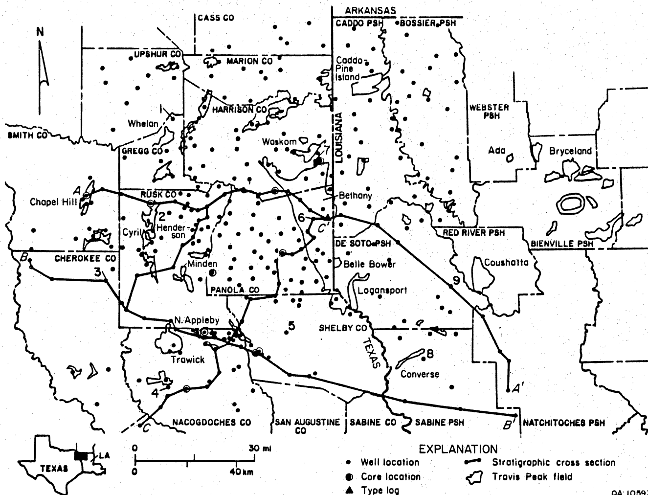
Figure 4: Location of East Texas counties and West Louisiana parishes included in the study of low-permeability, gas-bearing sandstones in the Travis Peak Formation. Major Travis Peak fields, well locations, and lines of cross sections are shown. Numbered wells correspond to well logs shown in figures 29-33.
