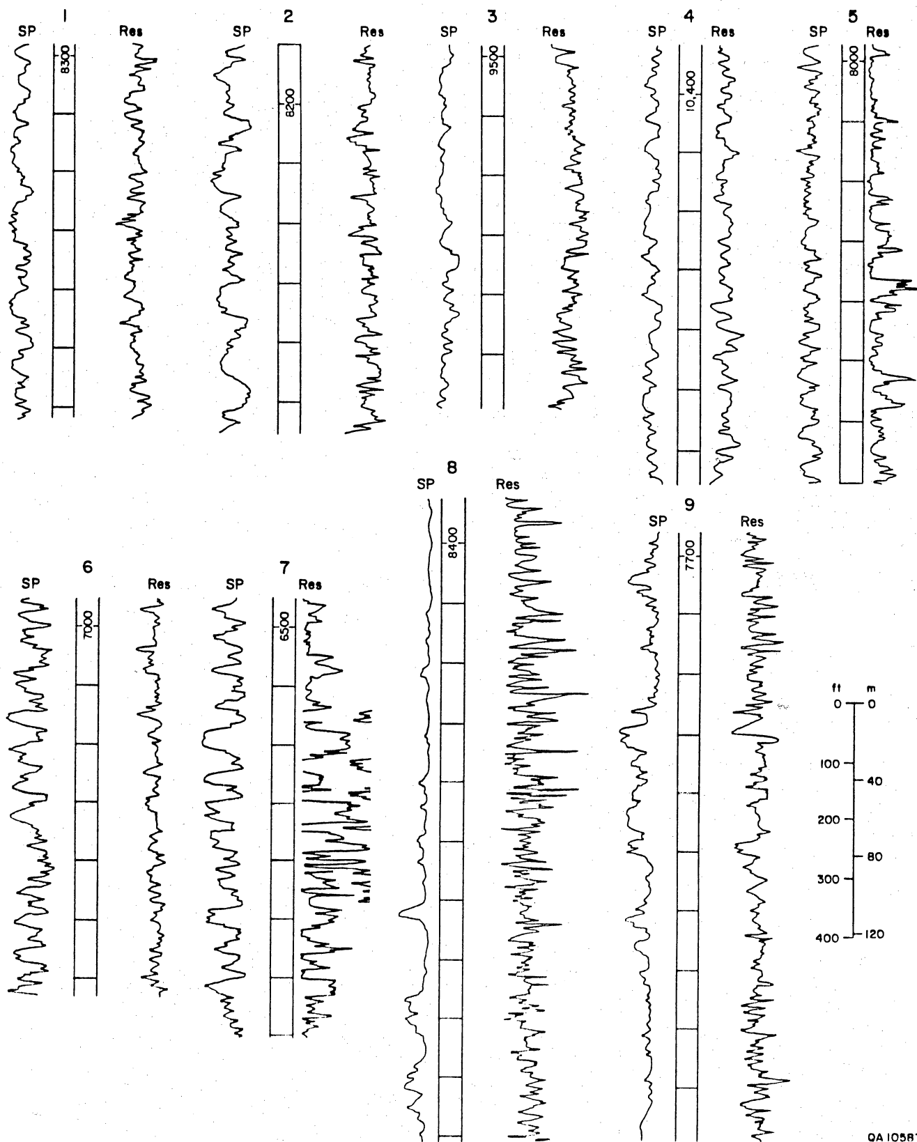
Figure 31: Representative SP and resistivity curves for lithostratigraphic unit 3. Location of wells is given in figure 4.
