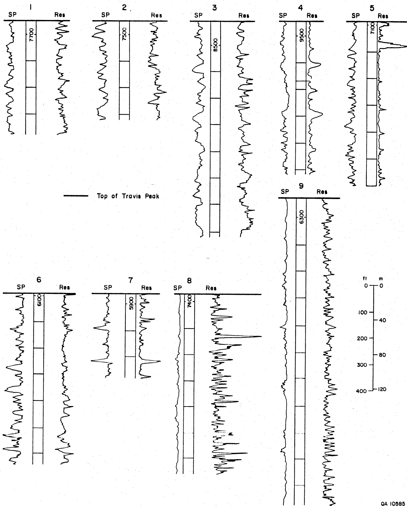
Figure 33: Representative SP and resistivity curves for lithostratigraphic unit 5. Location of wells is given in figure 4.
