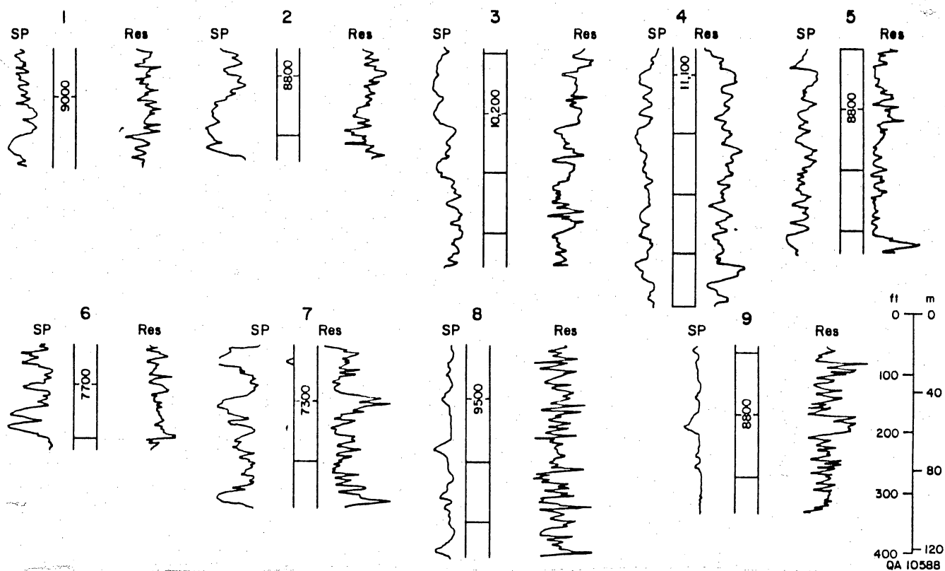
Figure 30: Representative SP and resistivity curves for lithostratigraphic unit 2. Location of wells is given in figure 4.
