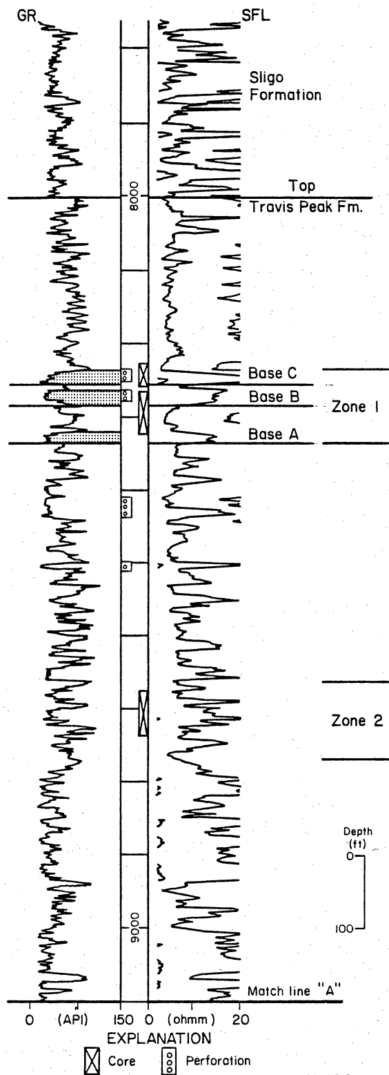
Figure 37: Gamma-ray and resistivity (SFL) logs for the Travis Peak Formation in the SFE No. 2 well. Zones 1 through 4 refer to cored stratigraphic intervals that were studied in detail. Three sandstones separated by mudstones are present in Zone 1, and these sediments are interpreted as poorly developed braided-channel sandstones, levee, splay, and lacustrine sandstones, and floodplain (swamp) mudstones. The three sandstones separated by mudstones in Zone 4 are interpreted as well-developed braided-channel sandstones, levee, splay, and lacustrine sandstones, and floodplain (swamp) mudstones.
