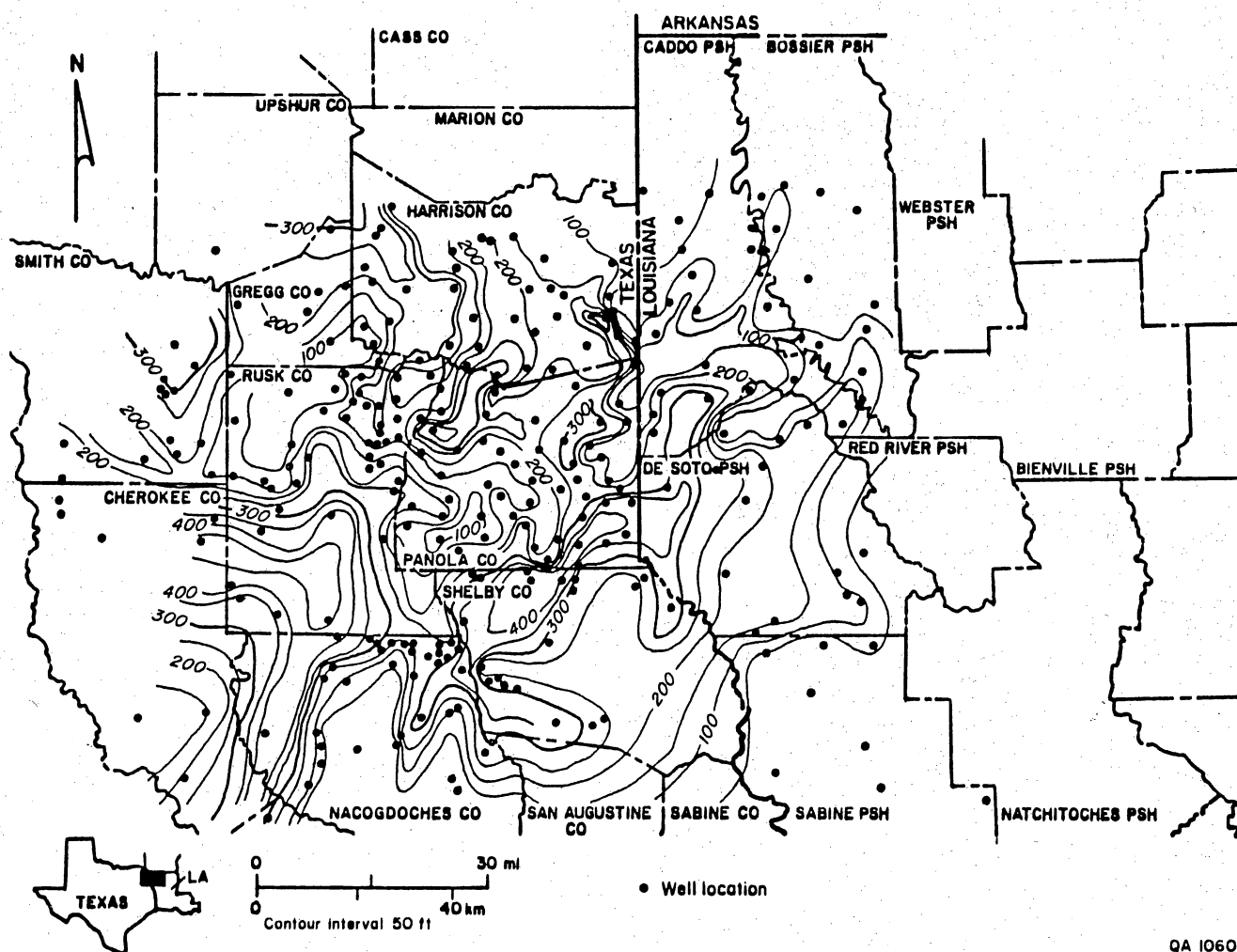
Figure 21: Net-sandstone map of lithostratigraphic unit 5.
