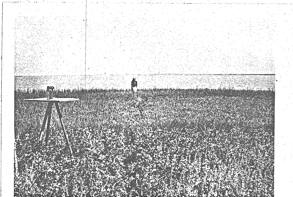
Figure 3. Plane table and telescopic alidade set up at station 1MA on marsh transect 2.
