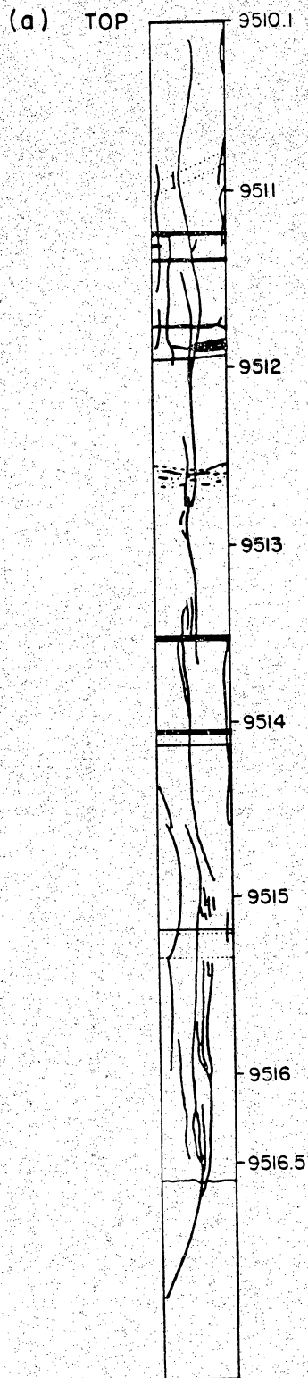
Figure 12. Field sketch of the hydraulic fracture induced by open-hole stress test 2, core 7. (a) Overall sketch of the fractured interval showing multiple fracture strands. The fracture strands occur in very fine grained sandstone, occasionally gradational to muddy sandstone, with local thin beds of dark gray shale and shale rip-up clasts. (b) Detail of part of the stress test fracture set, showing the three dimensional relation of individual fracture planes. Inset shows map of the top of the core in this interval.
