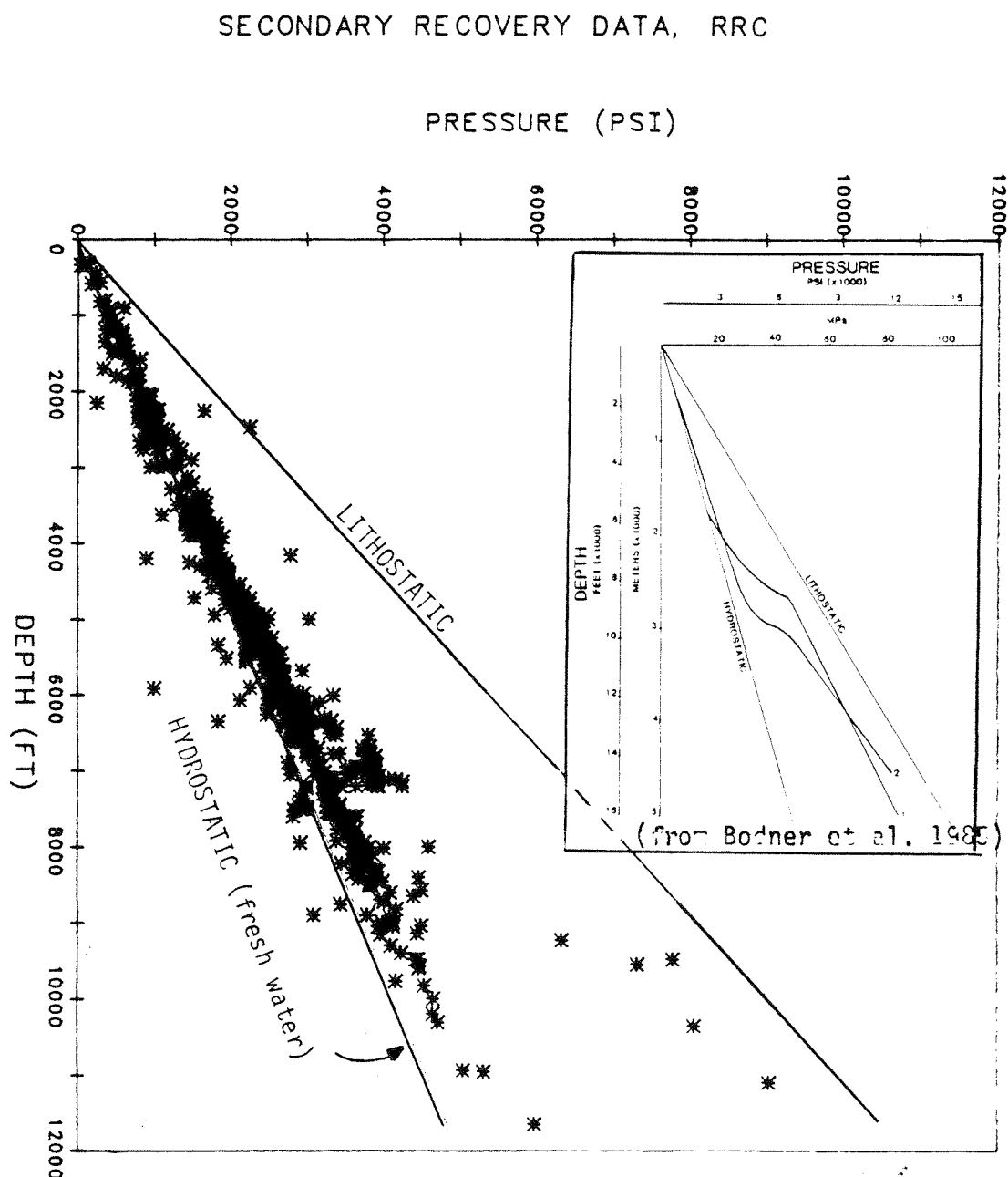
Figure 61. Pressure-depth plot of formation water, Texas Gulf Coast (data from Railroad Commission of Texas, 1978). Data follow hydrostatic conditions of fresh water and fall within the range of pressures reported by Dickinson (1953) and Jones (1968) (inset plot from Bodner and others, 1985).
