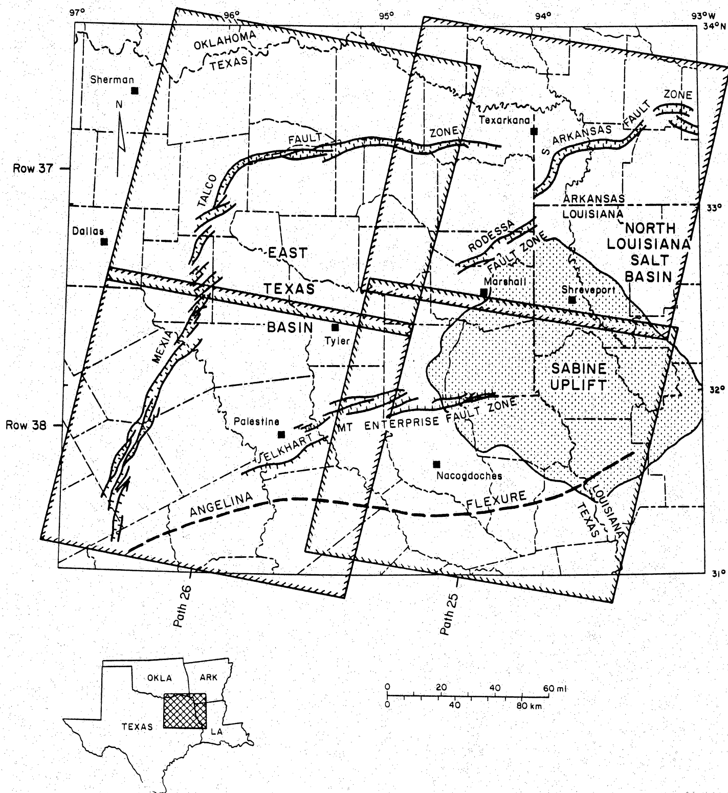
Figure 1. Location map of study area showing major tectonic elements and boundaries of Landsat images. Note area of sidelap between images in Paths 25 and 26. Fault zones in Texas are from Ewing (in preparation).
