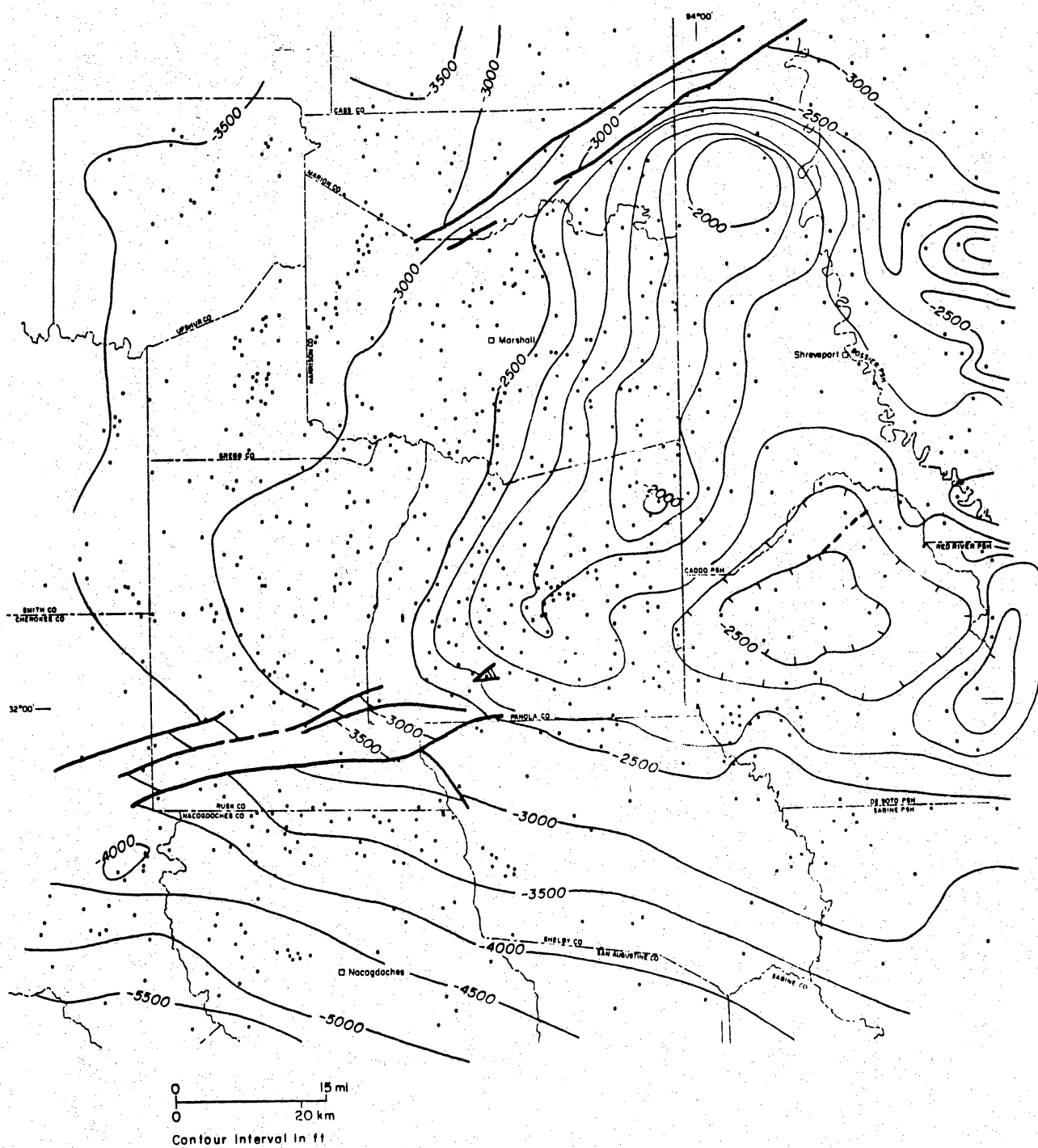
Structure Map Base of Austin Group
