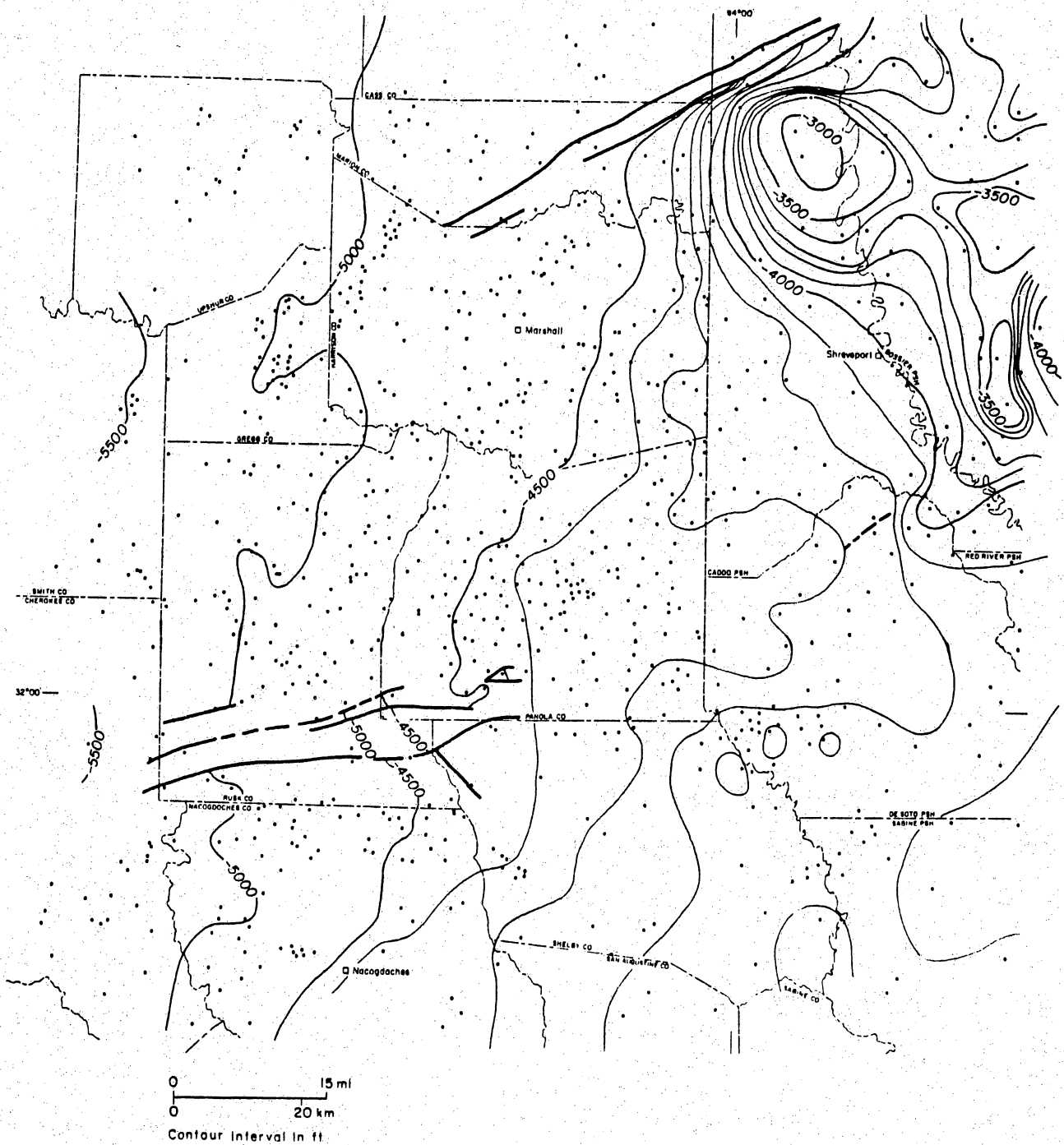
Figure 39. Palinspastic map on the base of the Massive Anhydrite, Sabine Uplift area.
