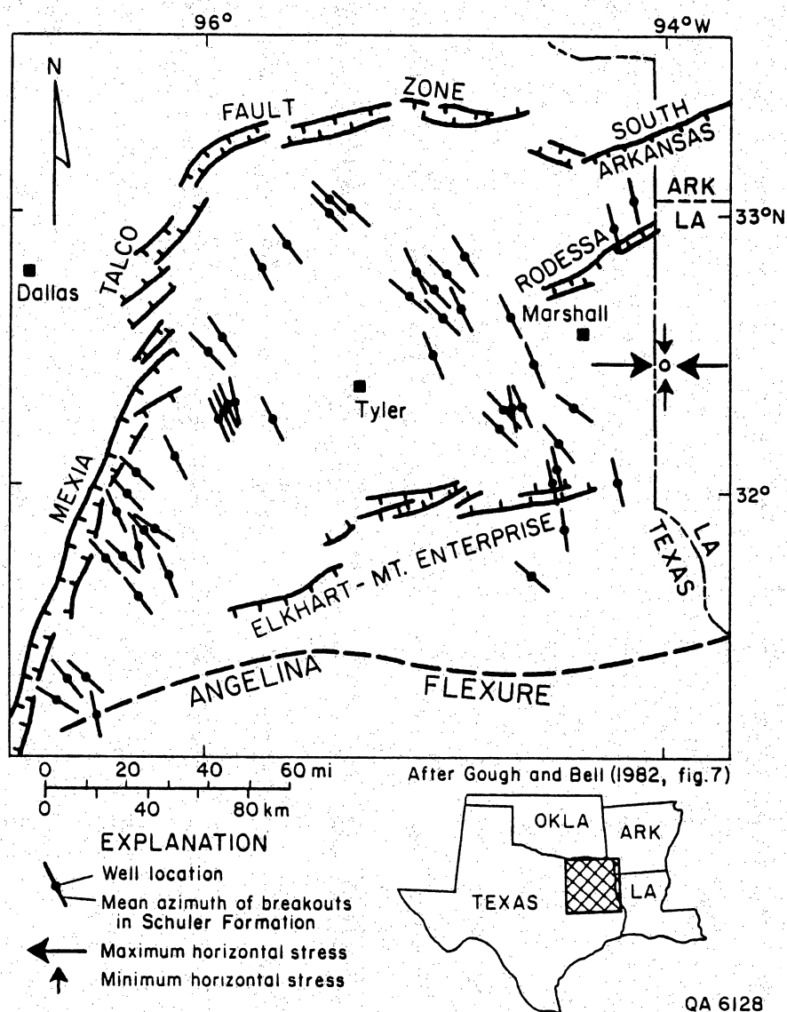
Figure 18. Map of breakouts in wells in the Schuler Formation, East Texas. Mean azimuth of all breakouts in 50 wells is 325^{\circ} . This is exactly the same as the significant northwest regional azimuth for lineament data in the study area (fig. 7C). Well data from Brown and others (1980), cited in Gough and Bell (1982, their fig. 7). Data for horizontal stresses from well near Texas-Louisiana border are from Strubhar and others (1975). Maximum horizontal stress is oriented east-west.
