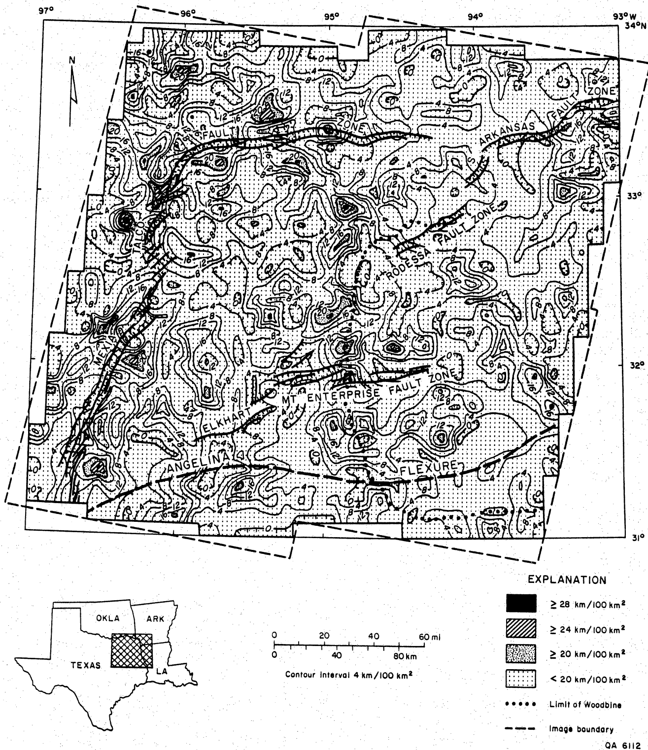
Figure 12. Map of lineament density (km/100 km 2 ). High values demarcate the Mexia-Talco Fault Zone, as well as other structural features. Limit of Woodbine from Ewing (in preparation).
