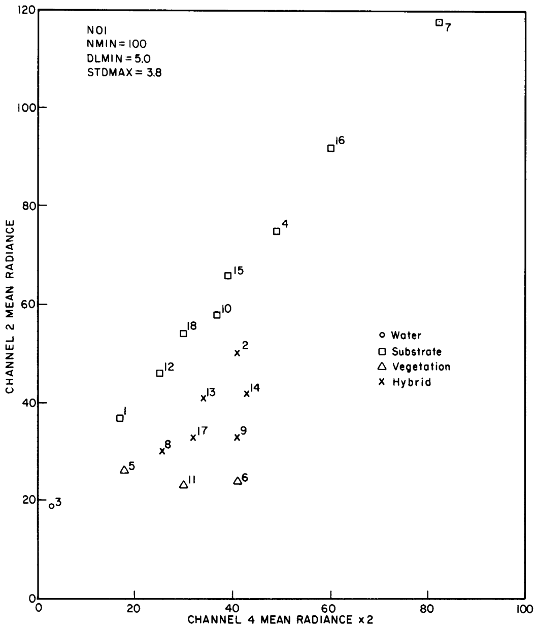
Figure 9. Mean radiance values of Landsat data in channels 2 and 4 (Landsat MSS bands 5 and 7) for the NO1 window (fig. 4). NMIN, DLMIN, and STDMAX are parameters used in ISOCLS processing. Compare figure 8.
