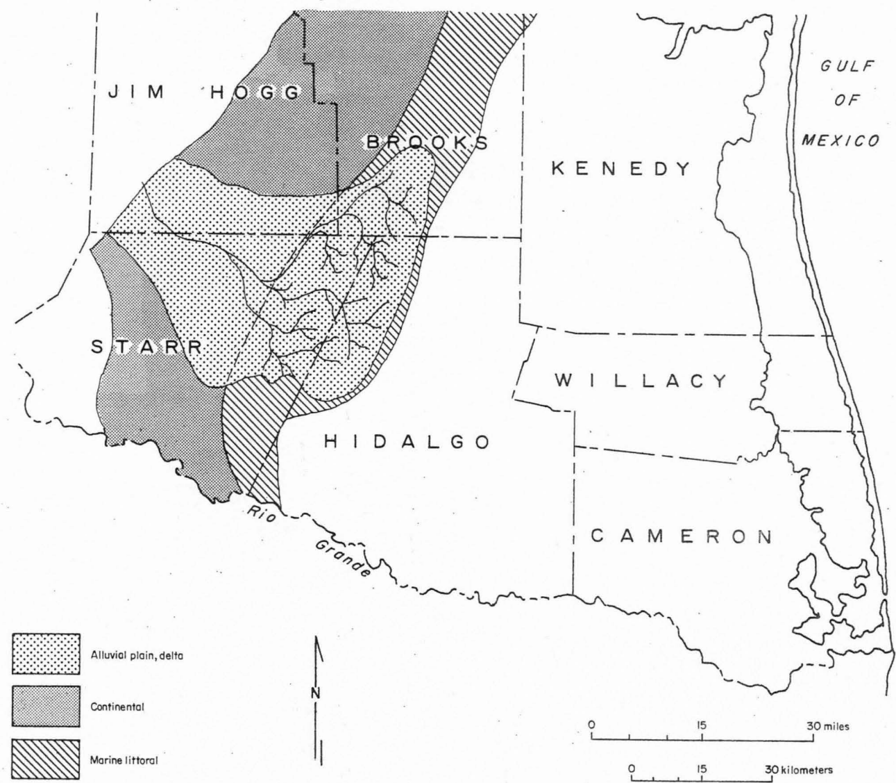
Figure 35. Lower Vicksburg depositional environments. Modified from Ritch and Kozik (1966).
