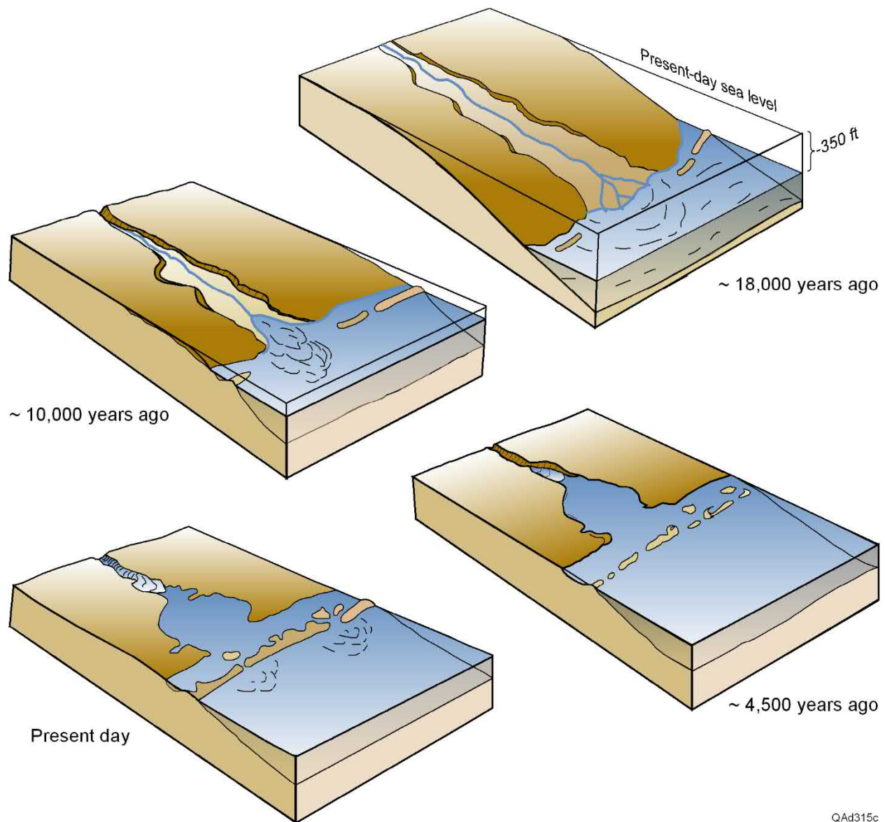
Figure 15. Schematic illustrations showing the effects of rising sea level on the evolution of ancient river valleys into the modern-day coastal environment.
