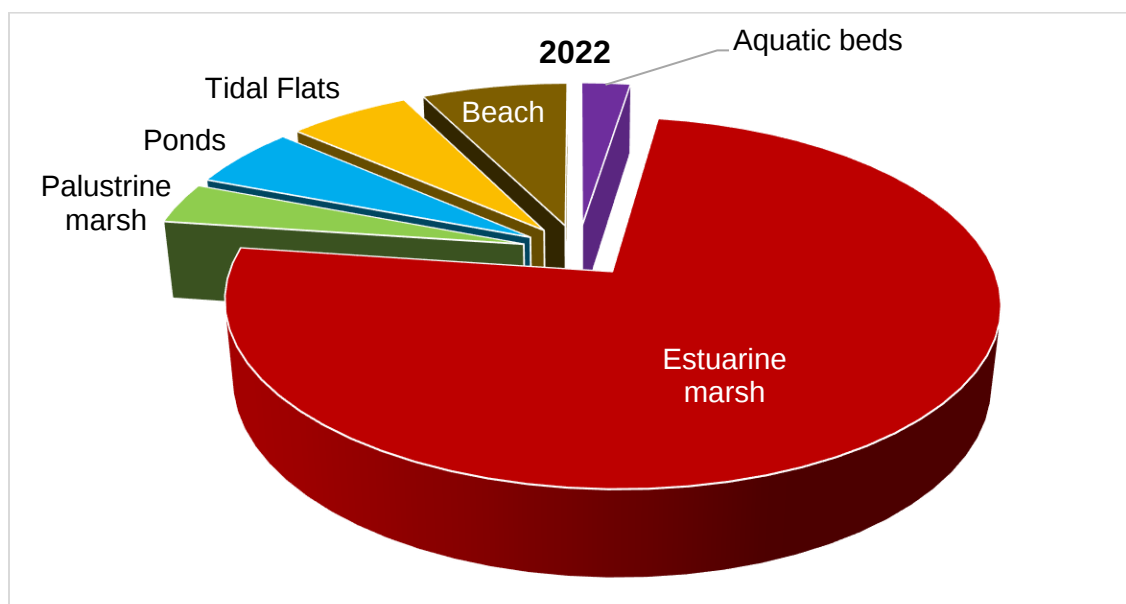
Figure 17. Areal extent of mapped wetland and aquatic habitats in 2022.
