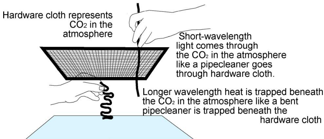
Figure 3. Model of the interaction of the atmosphere with light and heat.
