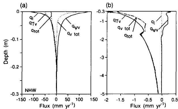
Figure 13. Variations in annual cumulative liquid ( q_l ), isothermal vapor ( q_{qv} ), thermal vapor ( q_{Tv} ), total vapor ( q_{v tot} ), and total (liquid plus vapor, q_{tot} ) flux for (a) the upper 0.3 m and for (b) 0.3–5 m for NHW.
