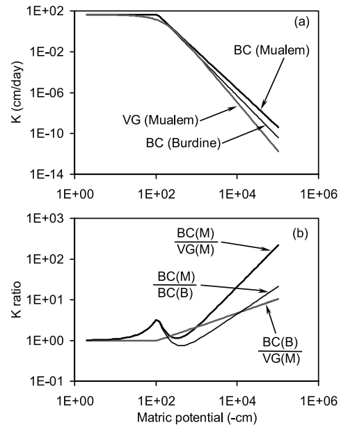
Figure 6. (a) Unsaturated hydraulic conductivities and (b) ratios of hydraulic conductivities calculated from van Genuchten (VG) and Brooks and Corey (BC) water retention functions and from Mualem (M) and Burdine (B) hydraulic conductivity functions. The various ratios are used to show differences in unsaturated hydraulic conductivity on the basis of different water retention functions (BC versus VG), different hydraulic conductivity functions (M versus B), or both.
