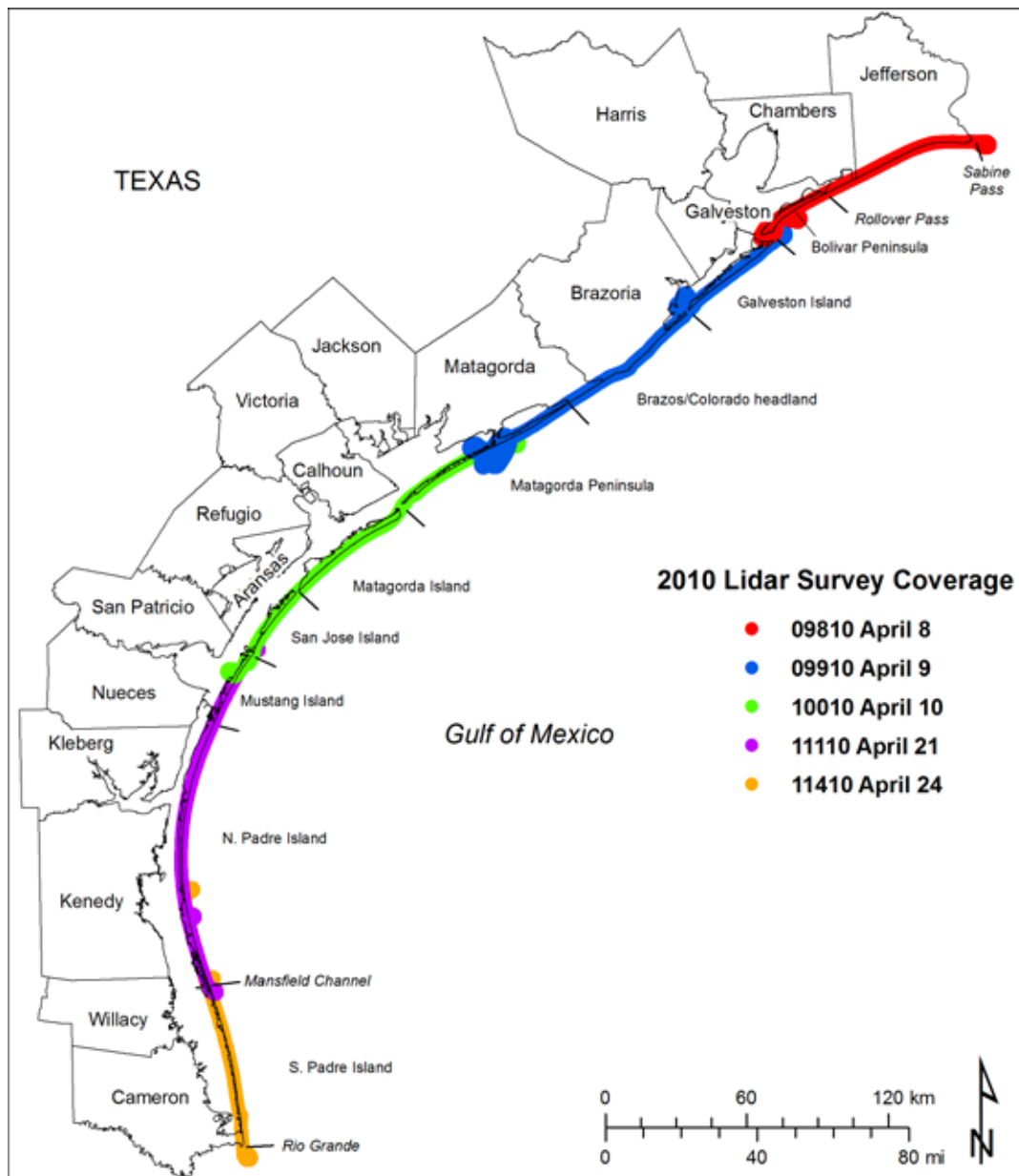
Figure 4. Coverage map of the 2010 lidar survey.
