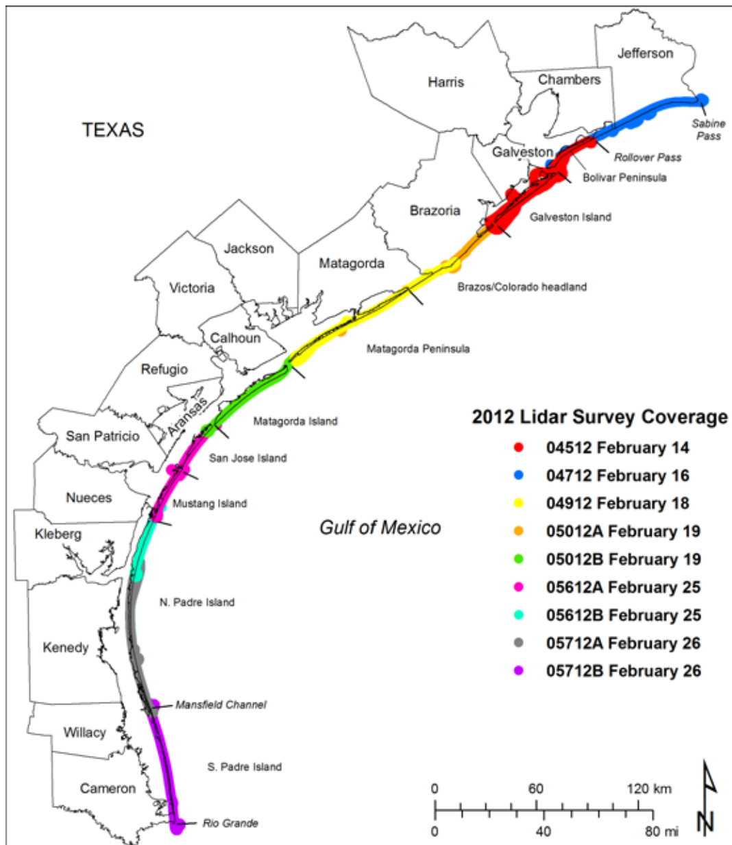
Figure 6. Coverage map of the 2012 lidar survey.
