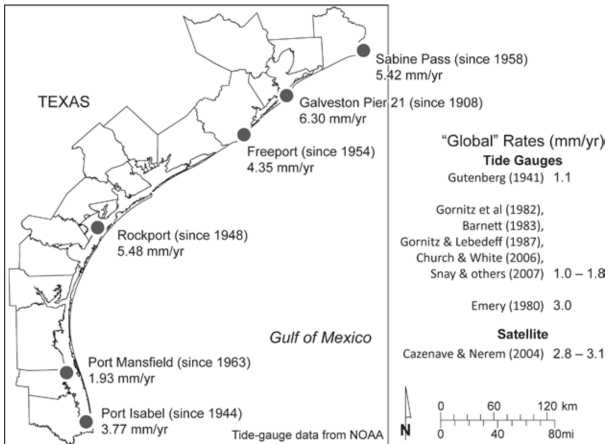
Figure 2. Sea-level trend at selected Texas tide gauges through 2012 and “global” rates determined from tide gauges and satellite data. Texas tide-gauge data from National Oceanic and Atmospheric Administration.
