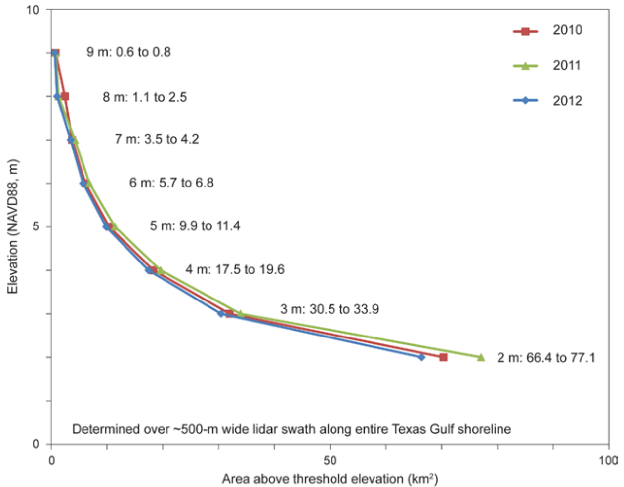
Figure 12. Total area above threshold elevations in 2010, 2011, and 2012 along the Texas Gulf shoreline.
