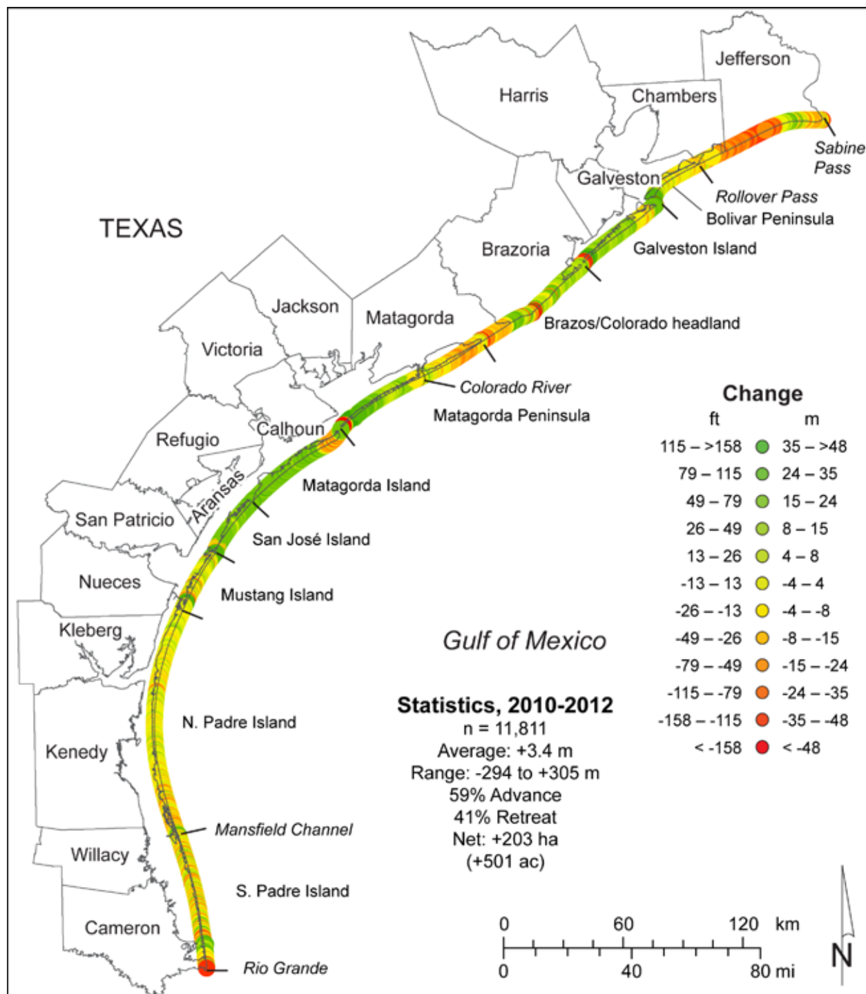
Figure 11. Net shoreline change between April 2010 and February 2012 from Sabine Pass to the Rio Grande. Change calculated from shoreline positions determined from airborne lidar surveys. Positive values indicate shoreline advance; negative values indicate shoreline retreat.
