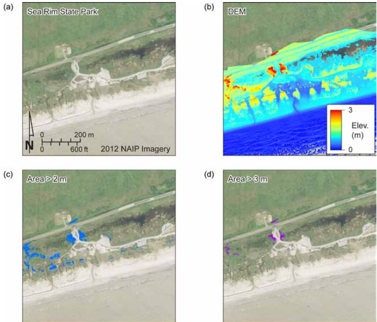
Figure 14. Sea Rim State Park DEM (b) and area slices at threshold elevations of (c) 2 m and (d) 3 m.
