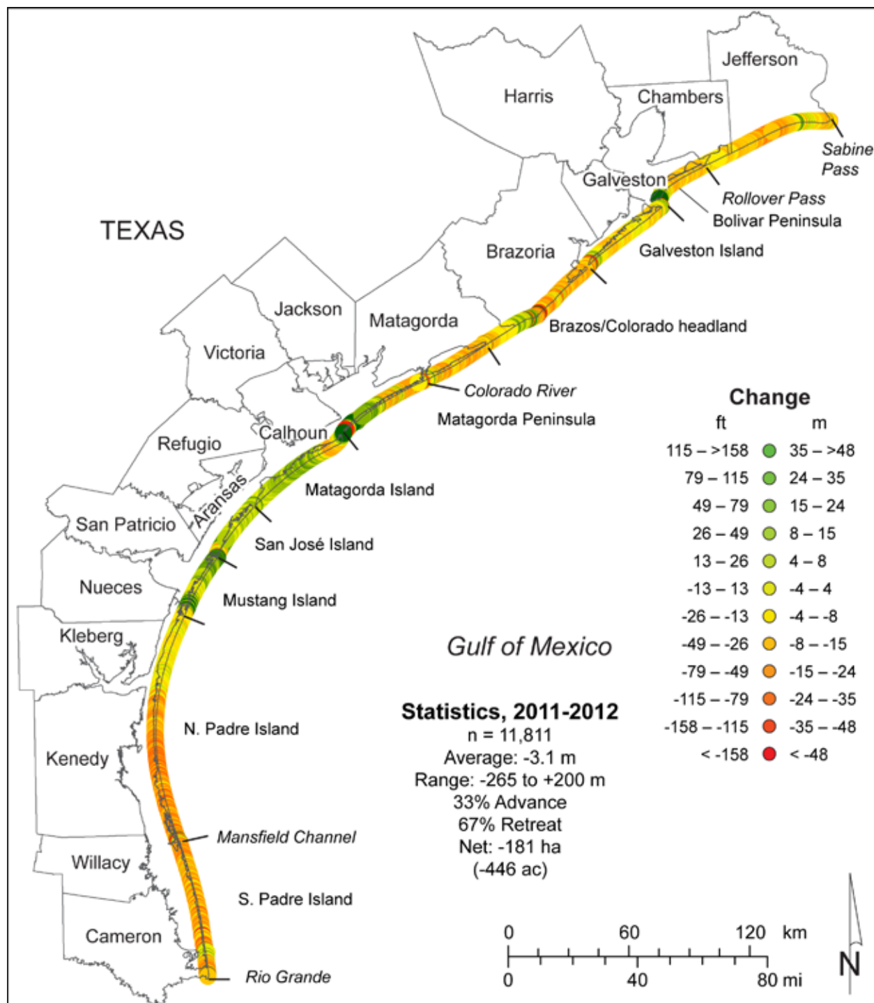
Figure 10. Net shoreline change between April 2011 and February 2012 from Sabine Pass to the Rio Grande. Change calculated from shoreline positions determined from airborne lidar surveys. Positive values indicate shoreline advance; negative values indicate shoreline retreat.
