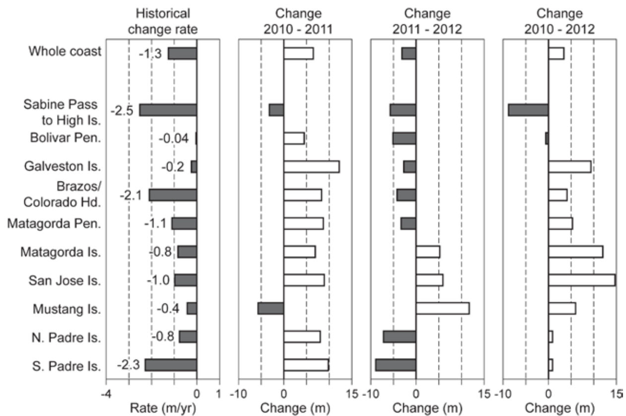
Figure 9. Comparison of incremental shoreline change measured between 2010 and 2012 with long-term shoreline change along the Texas Gulf shoreline.
