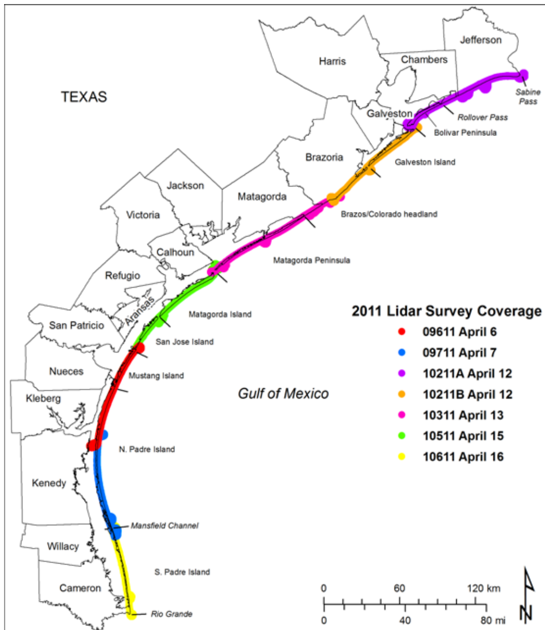
Figure 5. Coverage map of the 2011 lidar survey.
