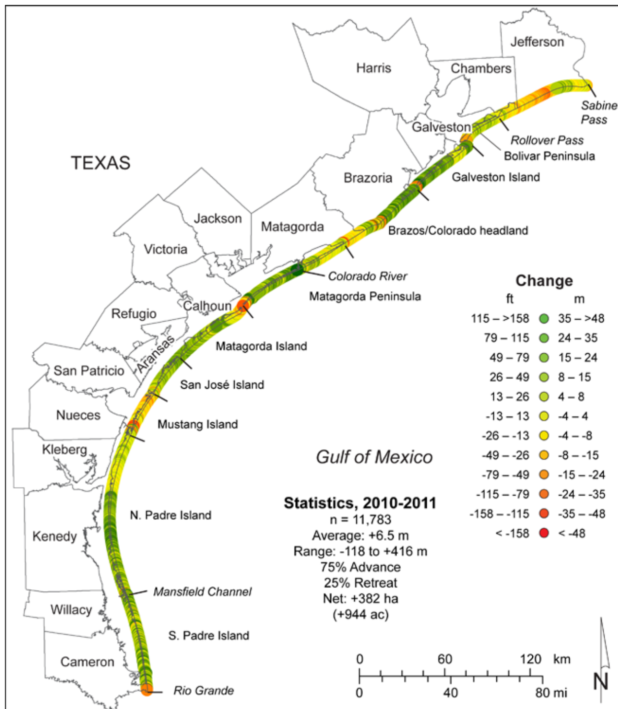
Figure 8. Net shoreline change between April 2010 and April 2011 from Sabine Pass to the Rio Grande. Change calculated from shoreline positions determined from airborne lidar surveys. Positive values indicate shoreline advance; negative values indicate shoreline retreat.
