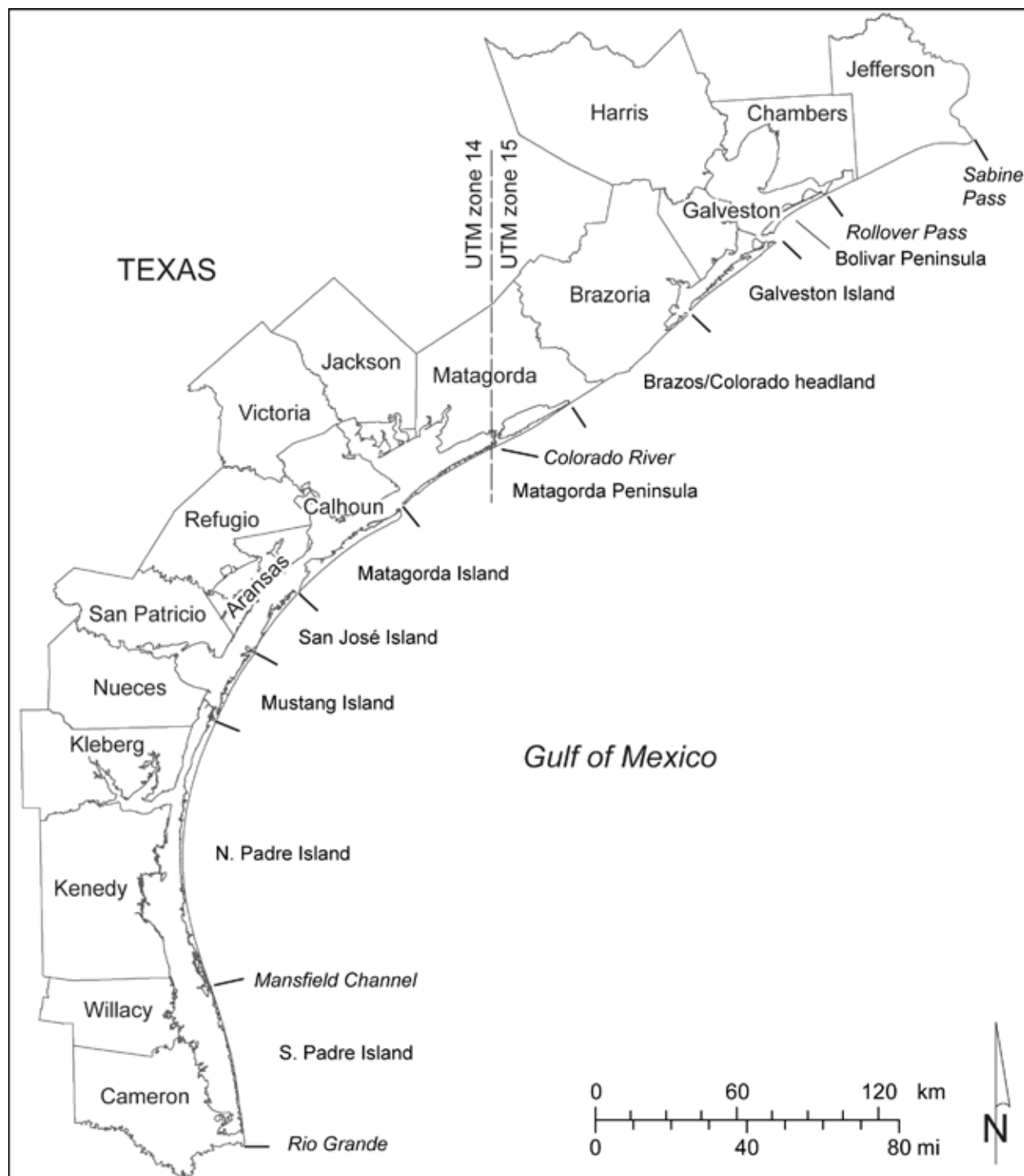
Figure 1. Map of the Texas coastal zone showing principal geomorphic features and coastal counties. Line segments extending seaward from the shoreline mark boundaries between major geomorphic features (barrier islands, peninsulas, deltaic headlands, and strandplains).
