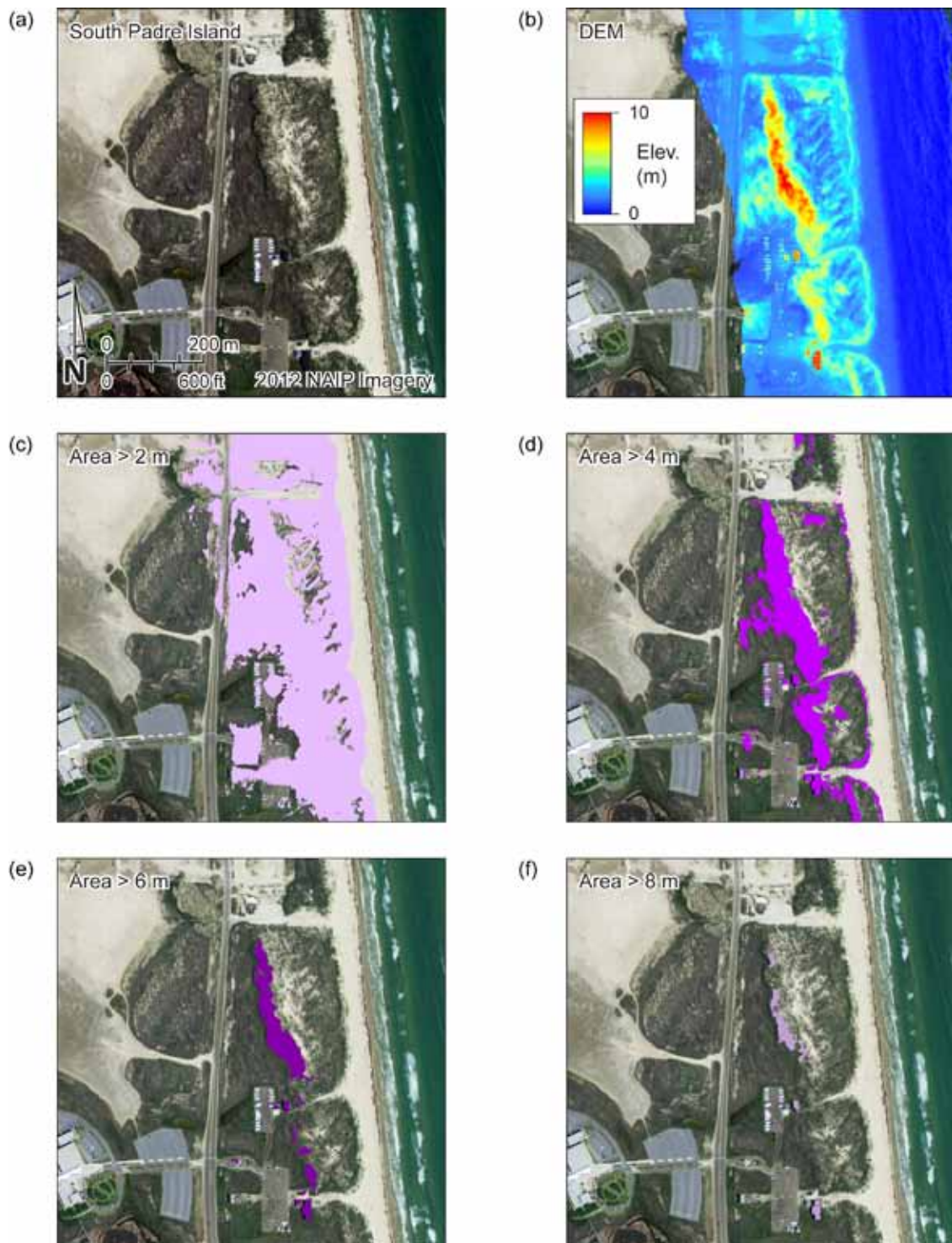
Figure 16. South Padre Island DEM (b) and area slices at threshold elevations of (c) 2 m, (d) 4 m, (e) 6 m, and (f) 8 m.
