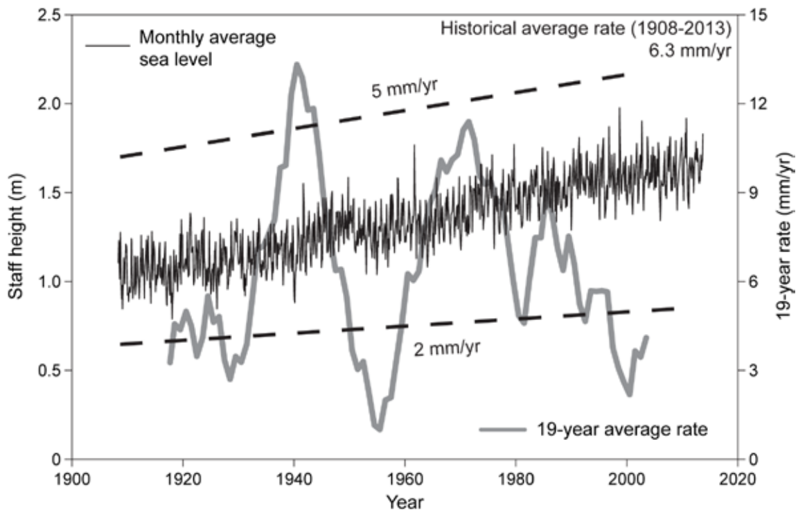
Figure 3. Sea-level trend at Galveston Pier 21, 1908 to 2013. Black line is monthly average sea level. Gray line is the average sea level measured over a 19-year period (the tidal datum epoch) and plotted at the center date of the period. Dashed lines indicate the slope of long-term rise at 2 mm/yr and 5 mm/yr. Data from National Oceanic and Atmospheric Administration.
