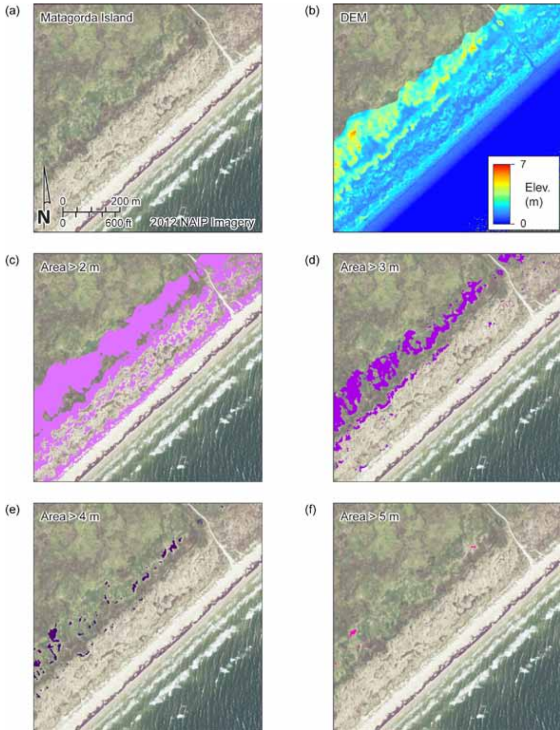
Figure 15. Matagorda Island DEM (b) and area slices at threshold elevations of (c) 2 m, (d) 3 m, (e) 4 m, and (f) 5 m.
