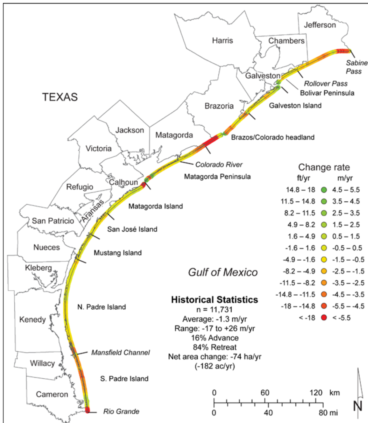
Figure 7. Net rates of long-term change for the Texas Gulf shoreline between Sabine Pass and the Rio Grande calculated from shoreline positions through 2007 (updated from Paine and others, 2011, 2012). Rates of change were calculated at 11,731 measurement sites spaced at 50-m intervals along the Gulf shoreline.
