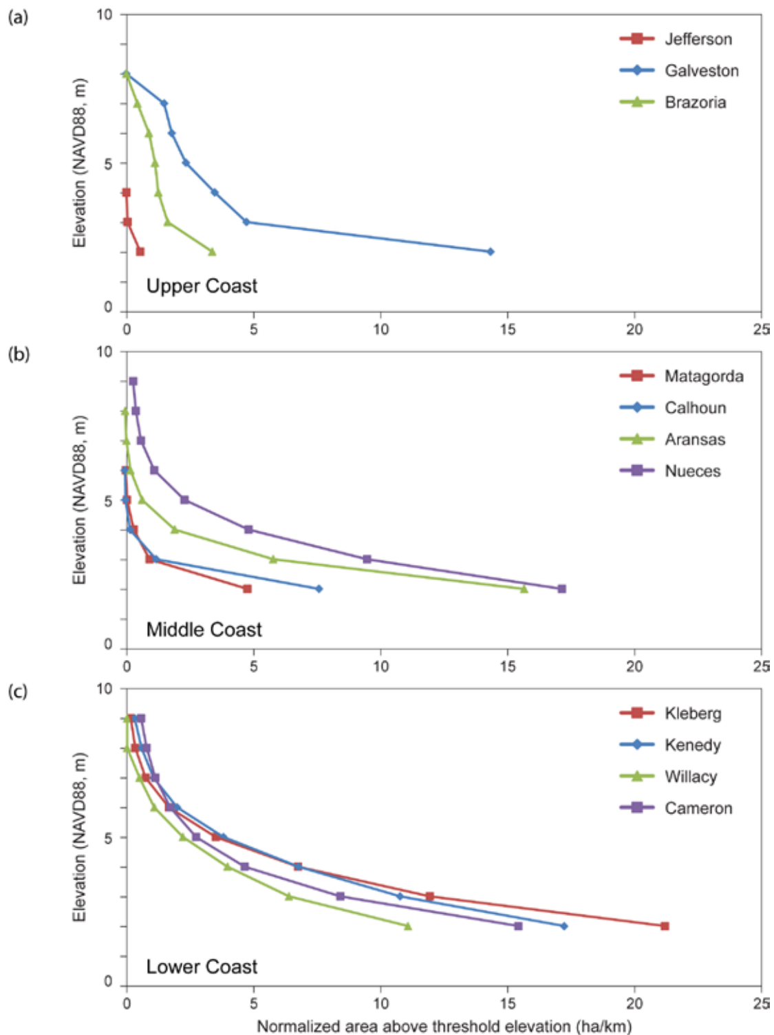
Figure 13. Normalized area above threshold elevations for upper, middle, and lower coast counties, Texas Gulf coast. ETA curves calculated from 2012 lidar-derived DEMs. Areas are normalized by dividing the total area above a given threshold elevation in a county by the length of shoreline in the county.
