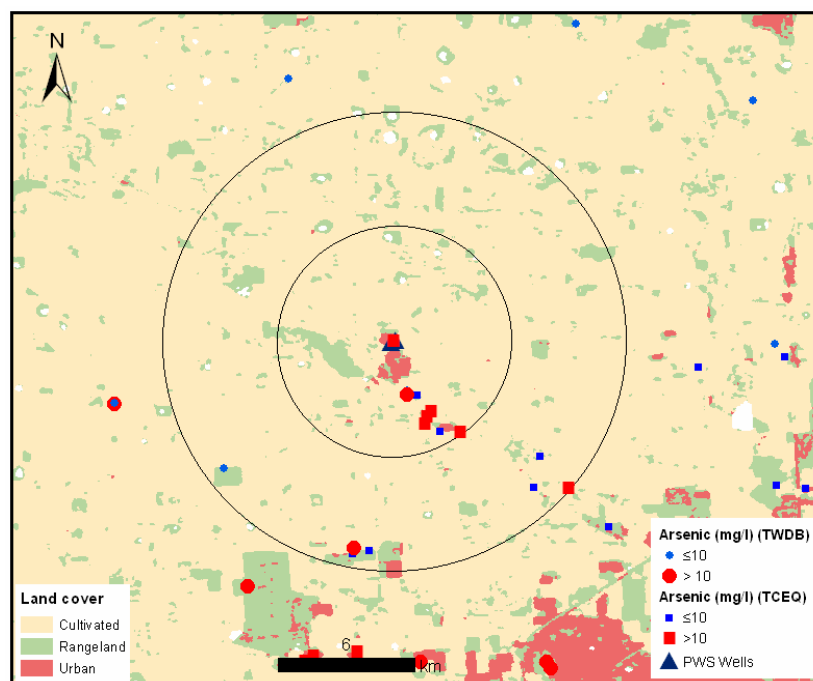
Figure 3.16 Arsenic Concentrations Within 5- and 10-Km Buffers of the Town North Village Water System PWS Wells
