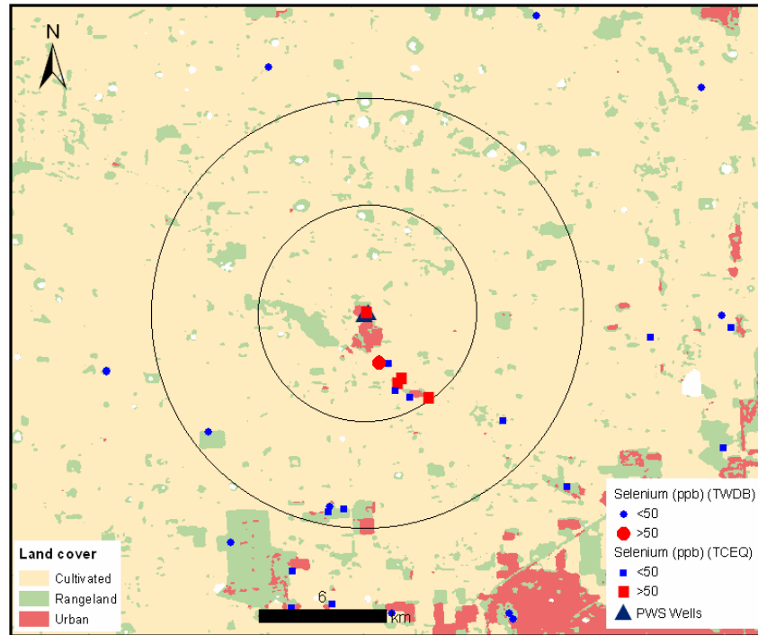
Figure 3.17 Selenium Concentrations Within 5- and 10-Km Buffers of the Town North Village Water System PWS Wells
