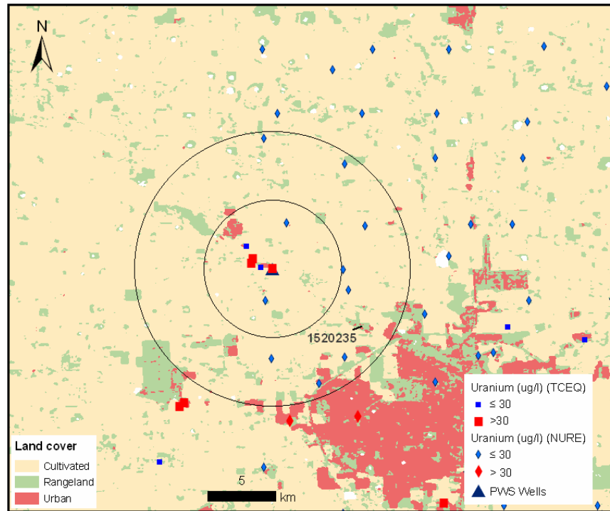
Figure 3.18 Uranium Concentrations Within 5- and 10-Km Buffers of the Town North Estates PWS Wells
