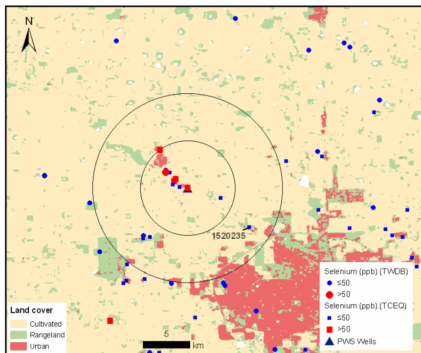
Figure 3.17 Selenium Concentrations Within 5- and 10-Km Buffers of the Town North Estates PWS Wells
