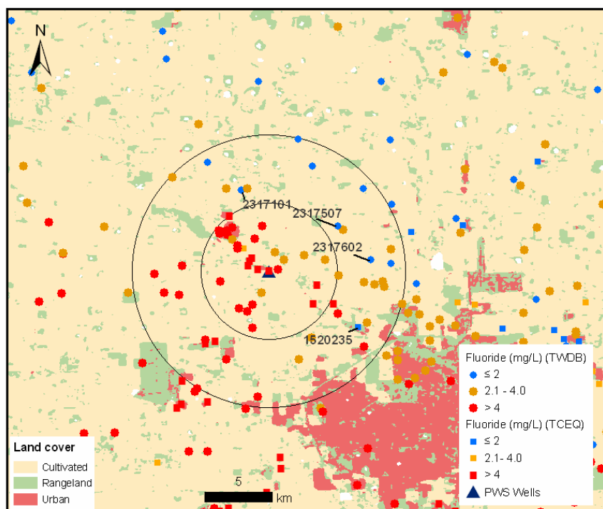
Figure 3.15 Fluoride Concentrations Within 5- and 10-Km Buffers of the Town North Estates PWS Wells
