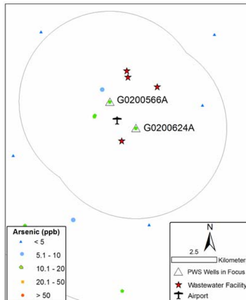
Figure 3.13 Arsenic Potential Sources of Contamination and Arsenic Concentrations in Wells Within a 5-km Buffer of the Oak Meadows Estates and Stoneridge Lake PWSs
