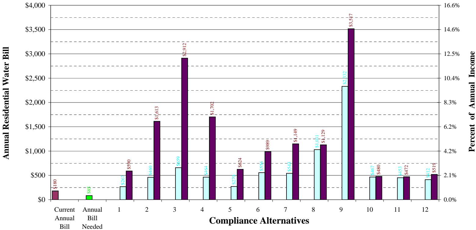
Figure 4-2 Lubbock RV Park - Alternative Cost Summary
