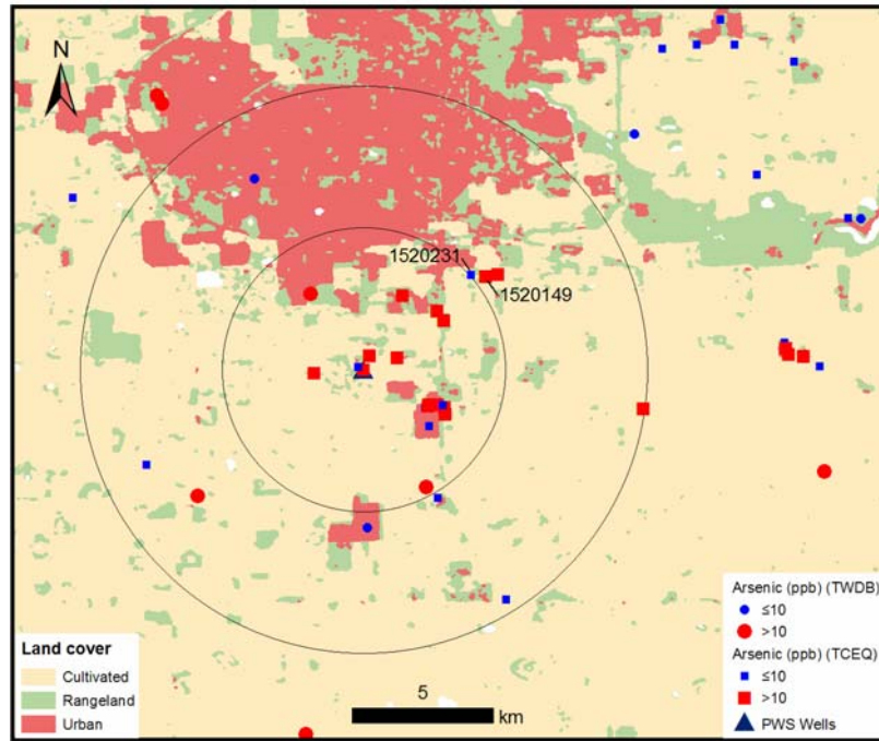
Figure 3.16 Arsenic Concentrations Within 5- and 10-Km Buffers of the Green Mobile Home Park PWS Wells
