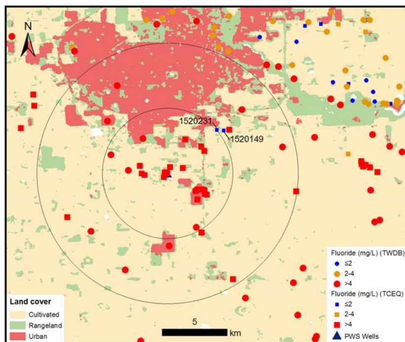
Figure 3.15 Fluoride Concentrations Within 5- and 10-Km Buffers of the Green Mobile Home Park PWS Wells
