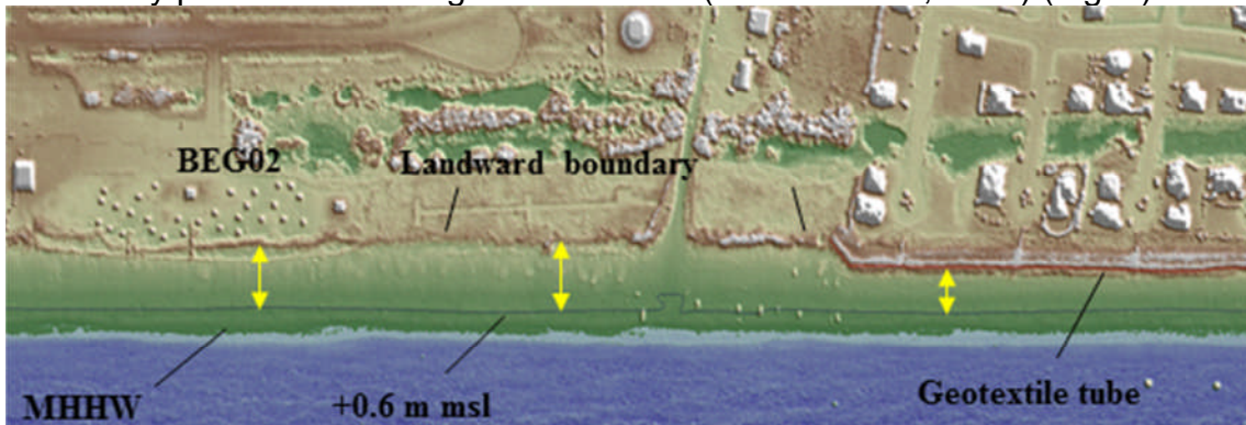
Figure 9. Lidar topographic-relief image of Galveston Island State Park and Pirates Beach subdivision. Note the difference in beach width between the natural beach and the area in front of the subdivision. From Gibeaut et al. (2003).
