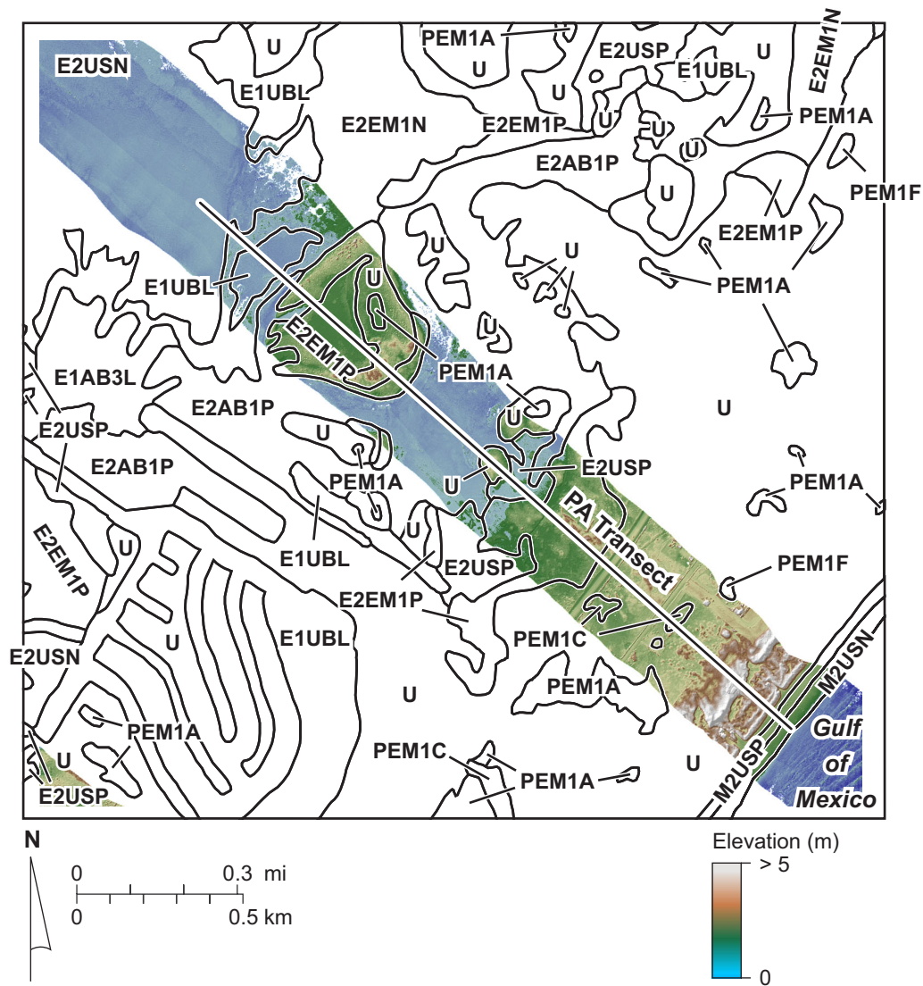
Figure 28. Digital elevation model (DEM) of the PA transect showing habitats identified on the 1992 NWI maps. The DEM was constructed from lidar data acquired along the transect in 2003.
