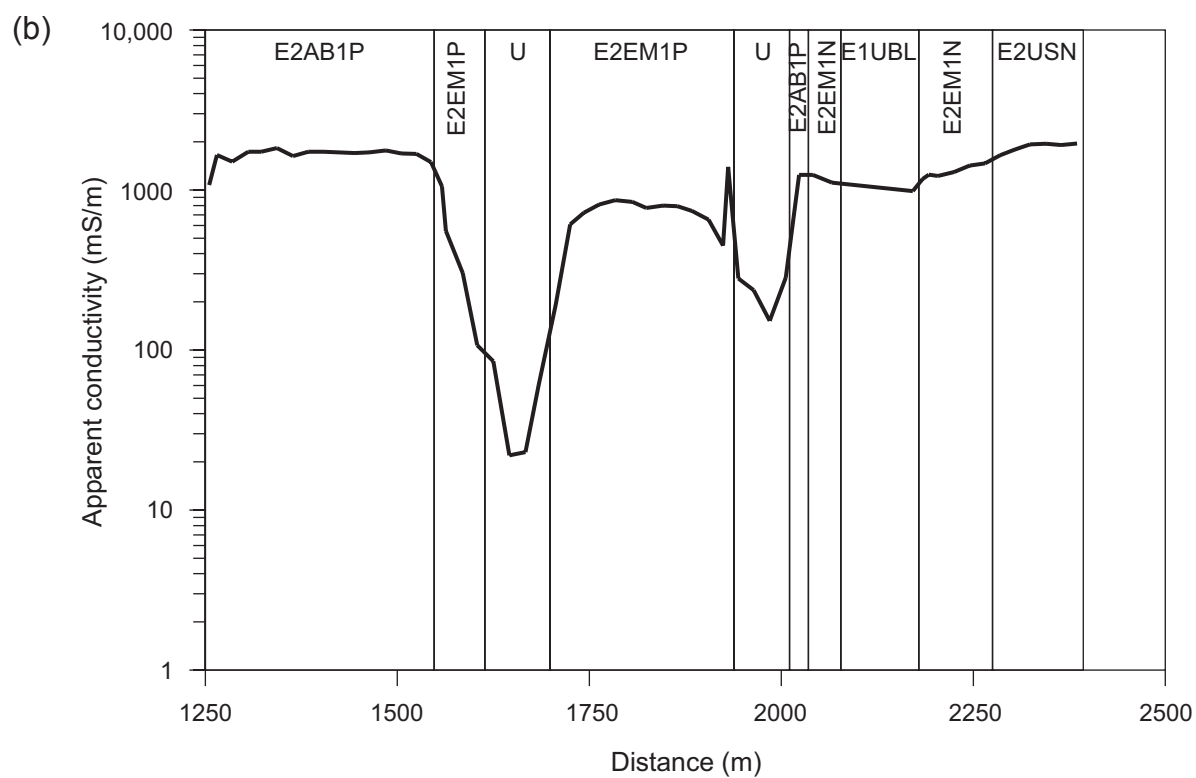
Figure 34. Apparent conductivity profile (vertical dipole orientation) superimposed with 1992 NWI units along the PA transect (a) between 0 and 1250 m and (b) between 1250 and 2400 m from the gulf shoreline.
