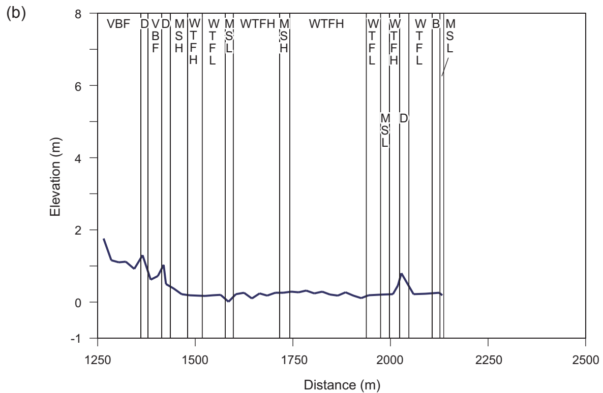
Figure 21. Elevation profile superimposed with surveyed coastal environments along the MISP transect (a) between 0 and 1250 m and (b) between 1250 and 2200 m from the gulf shoreline.
