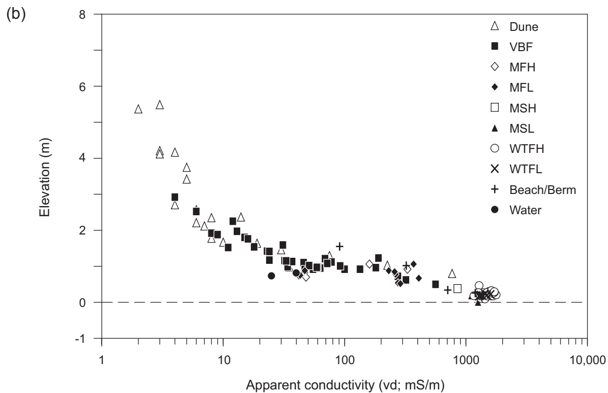
Figure 26. Elevation and apparent conductivity of (a) 1992 NWI units, and (b) coastal environments along the MISP transect. Apparent conductivity measured in the vd orientation.
