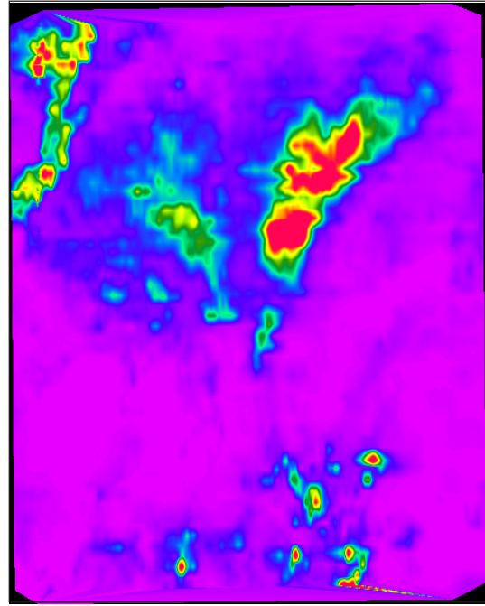
Figure 25. Co-registered images of the Montague Test Site created from (a) radar backscatter for VV polarization (C band = red, L band = green, and P band = blue) and (b) apparent ground conductivity measured at 56,000 Hz. Radar data from AIRSAR flight Montague 180-1.
