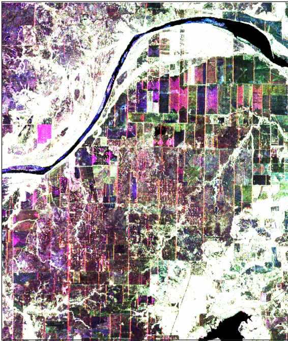
Figure 23. Georeferenced (a) L- and (b) P-band radar backscatter composites for the Prairie Valley School quadrangle, AIRSAR flight Montague 180-1. Composite images created using HH = red, HV = green, and VV = blue.
