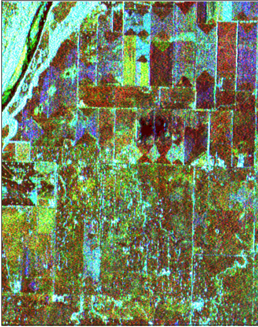
Figure 25. Co-registered images of the Montague Test Site created from (a) radar backscatter for VV polarization (C band = red, L band = green, and P band = blue) and (b) apparent ground conductivity measured at 56,000 Hz. Radar data from AIRSAR flight Montague 180-1.
