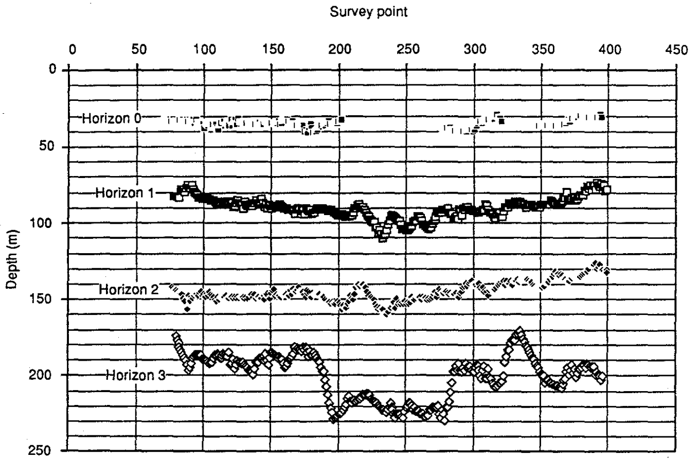
Figure 7. Calculated depths to major reflecting horizons interpreted from line PRLA.
