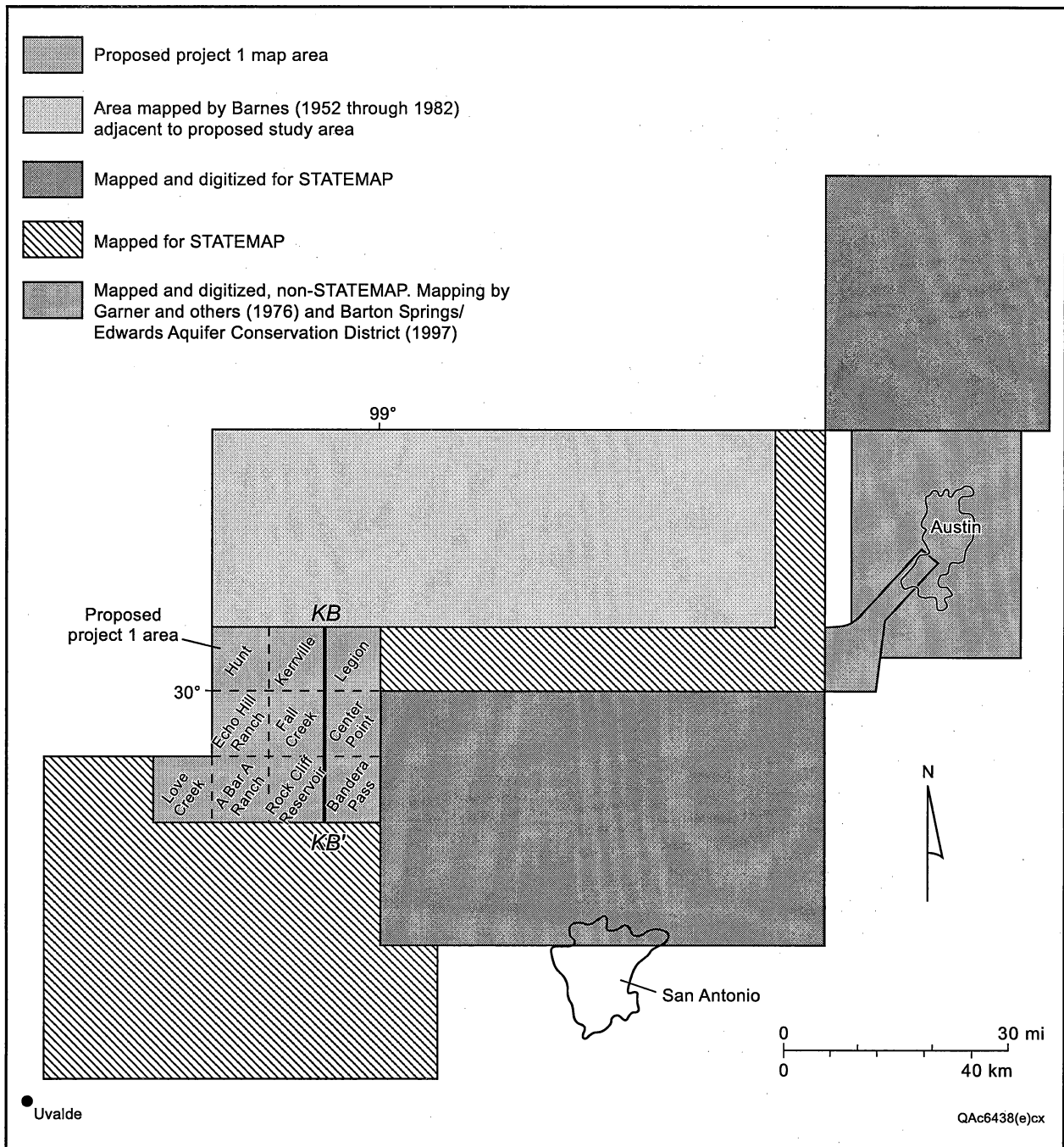
FIGURE 3. Location and quadrangles (1:24,000 scale) for project 1 area, Hill Country Trinity aquifer, Kerrville and Bandera area, Central Texas.
