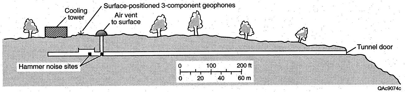
Fig. 2. Generalized section view of Fort Hood tunnel system along profile of Access Tunnel No. 2 (Fig. 1).
