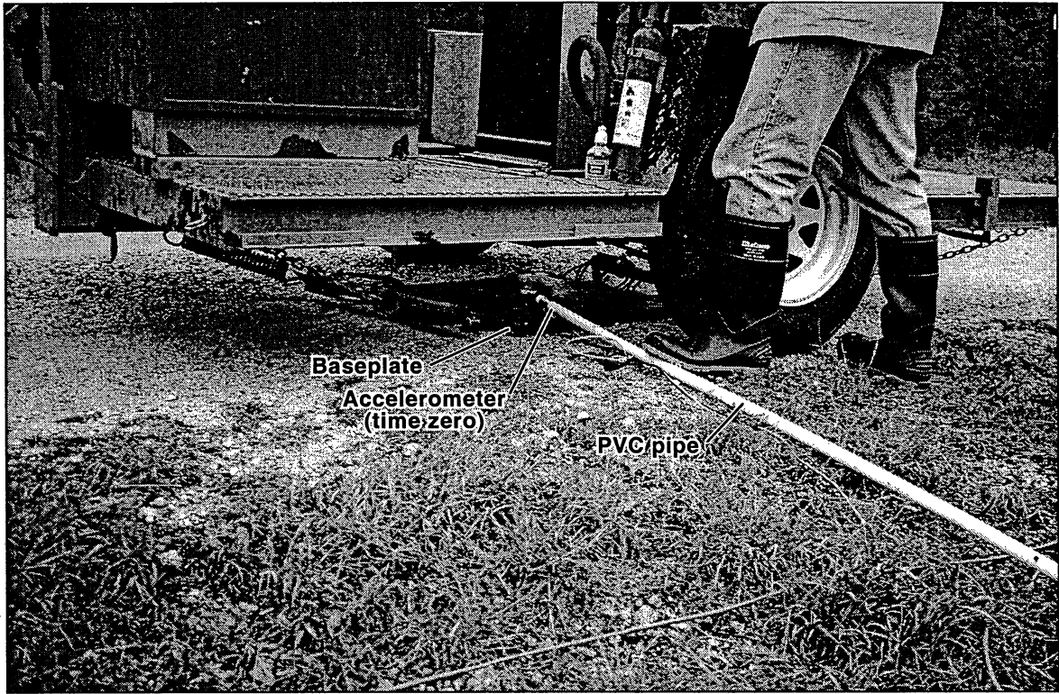
Fig. 16. Baseplate of weight-drop source and accelerometer used to establish time zero of the seismic impulse.
