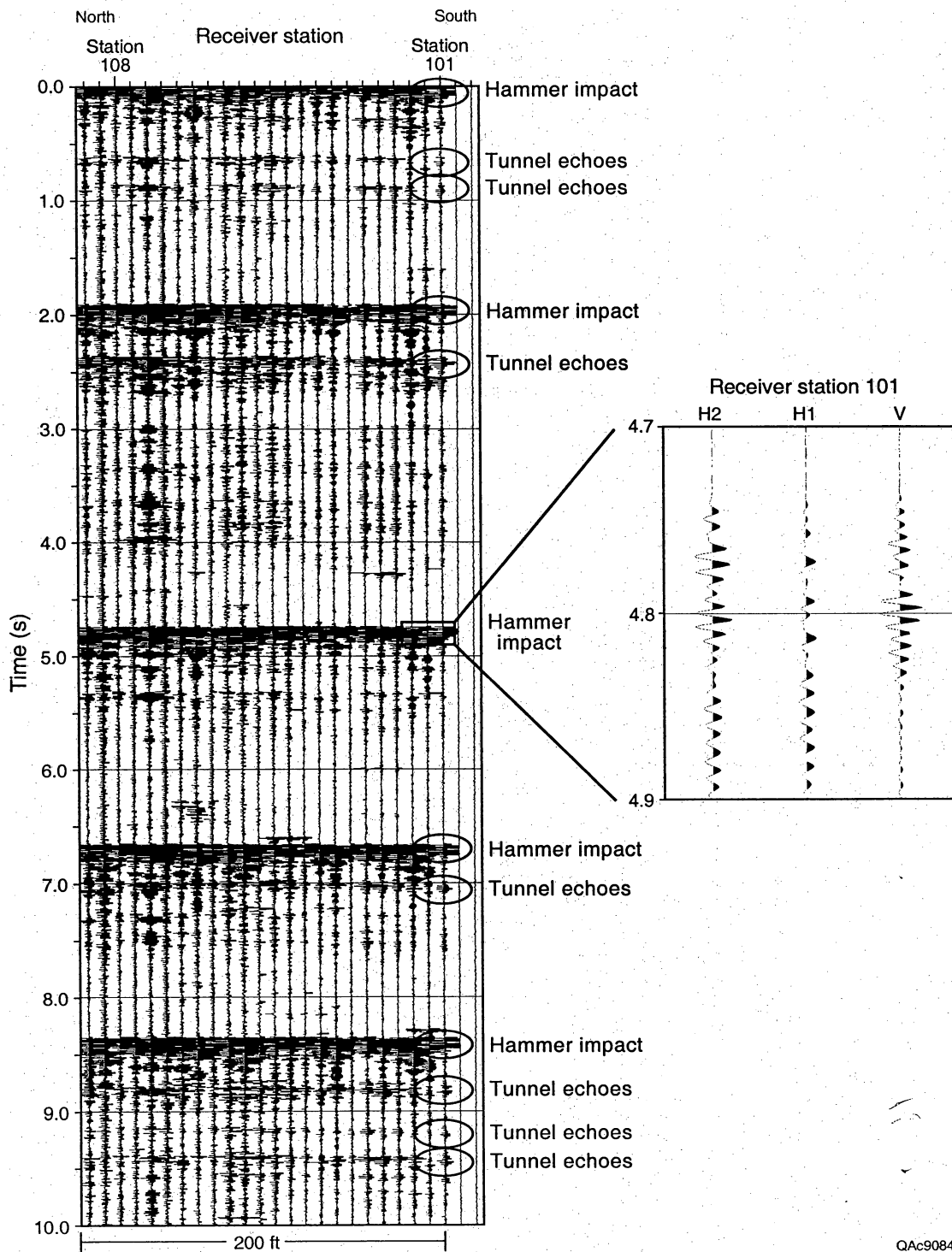
Fig. 8. Data recorded by 3-C surface geophones when hammer noise was created at site 1 in tunnel (Fig. 7).
