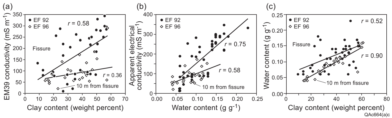
Figure 11. Relationship between EC_a measured with an EM39 meter and (a) clay content and (b) water content and relationship between water content and clay content for profiles in (EF 92) and 10 m away from (EF 96) the fissure.
