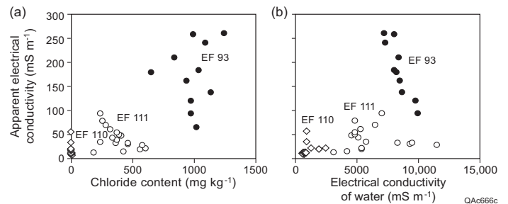
Figure 13. Relationship between EC_a measured with the EM39 downhole meter and (a) chloride content and (b) electrical conductivity of pore water ( EC_w ) in samples from EF 110 (draw), EF 93 (slope), and EF 111 (interdrainage).
