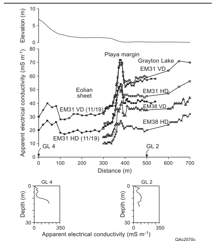
Figure 2. Variations in EC a along a transect from the sand sheet adjacent to Grayton Lake to Grayton Lake playa measured with EM31 and EM38 ground conductivity meters (VD, HD) and downhole EC a measured with the EM39 meter in boreholes GL 4 and GL 2. For location of transect see Fig. 1.
