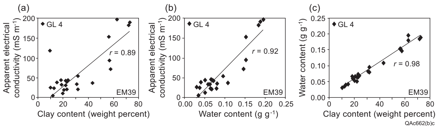
Figure 9. Relationship between EC_a measured with the downhole EM39 meter and (a) clay content, (b) water content, and (c) relationship between water content and clay content in samples from GL 4 adjacent to Grayton Lake.
