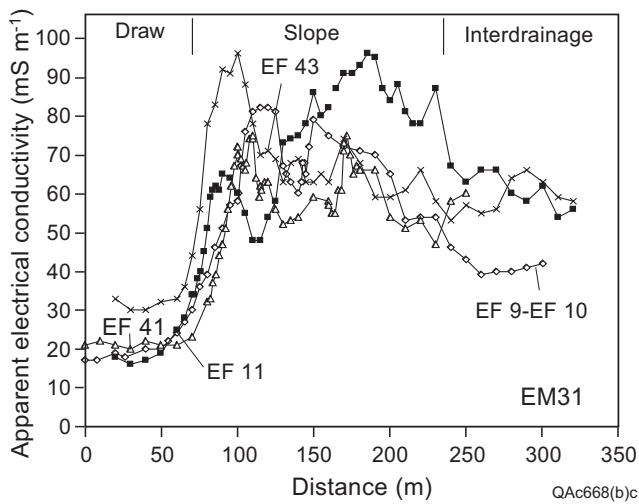
Figure 6. Variations in EC_a along transects at right angles to Blanca Draw measured with an EM31 ground conductivity meter (VD). For location of transects see Fig. 1.
