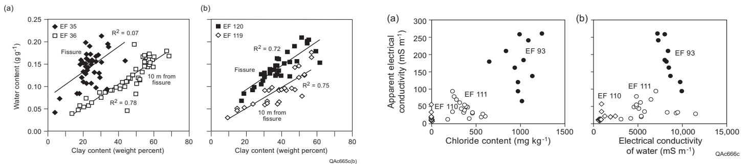
Figure 13. Relationship between EC_a measured with the EM39 downhole meter and (a) chloride content and (b) electrical conductivity of pore water ( EC_w ) in samples from EF 110 (draw), EF 93 (slope), and EF 111 (interdrainage).
