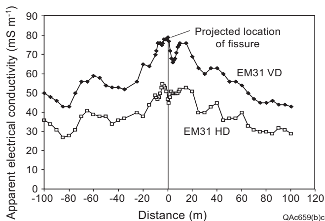
Figure 4. Electromagnetic induction transect measured with the EM31 meter (VD) across the projected line of the fissure, where there is no surface expression of the fissure. For location of transect see Fig. 1.
