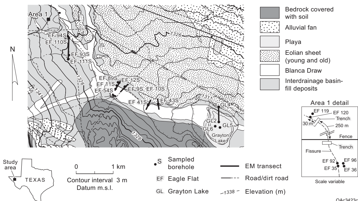
Figure 1. Location of electromagnetic induction transects and sampled boreholes relative to surface geomorphic settings in Eagle Flat Basin.
